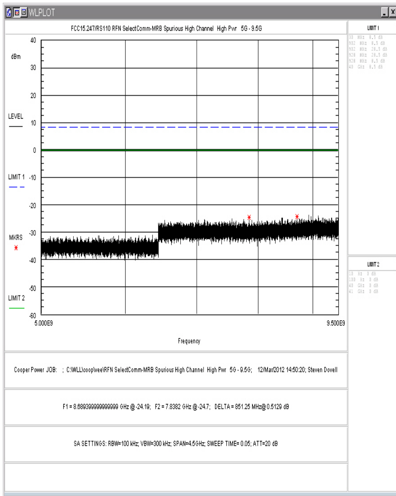
Figure 26: Conducted Spurious Emissions, High Power, High Channel 5-9.5GHz
