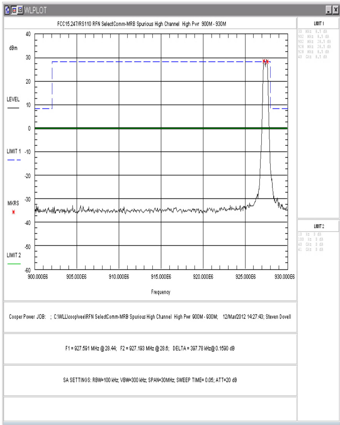
Figure 24: Conducted Spurious Emissions, High Power, High Channel 900 – 930MHz
