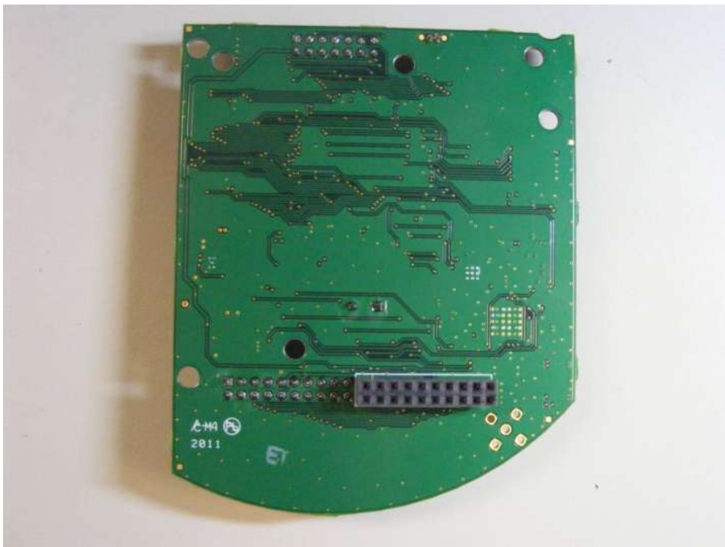
Figure 2: RFN430EL-A3 – Bottom
