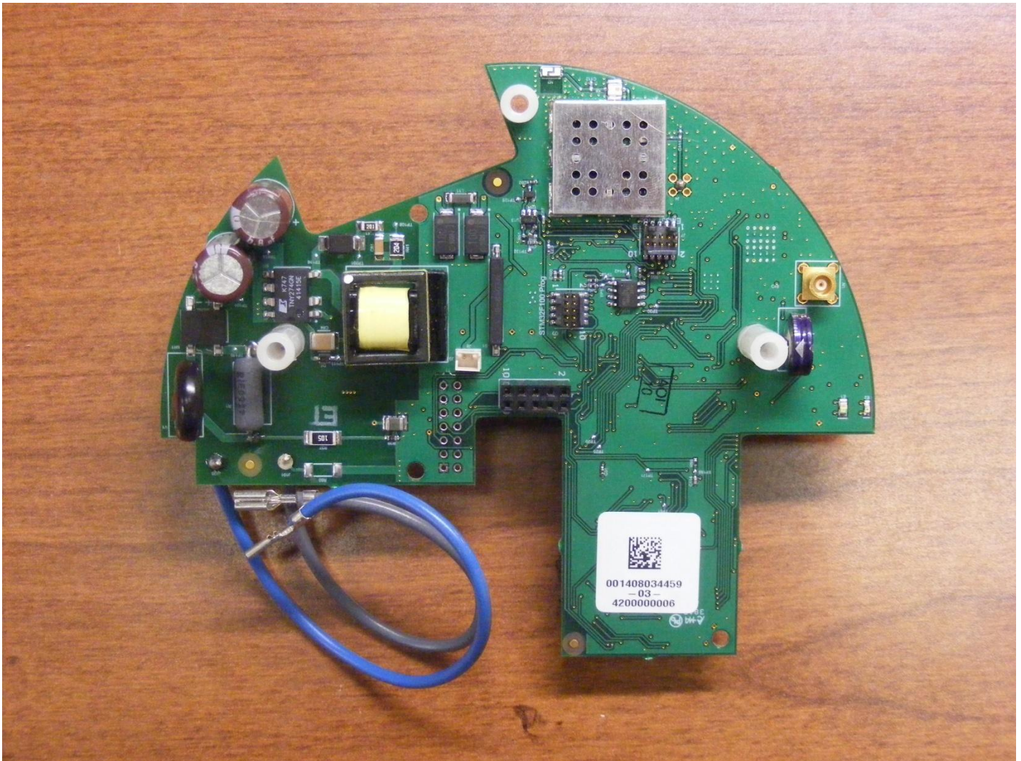
Figure 1: RFN420fL - Bottom
