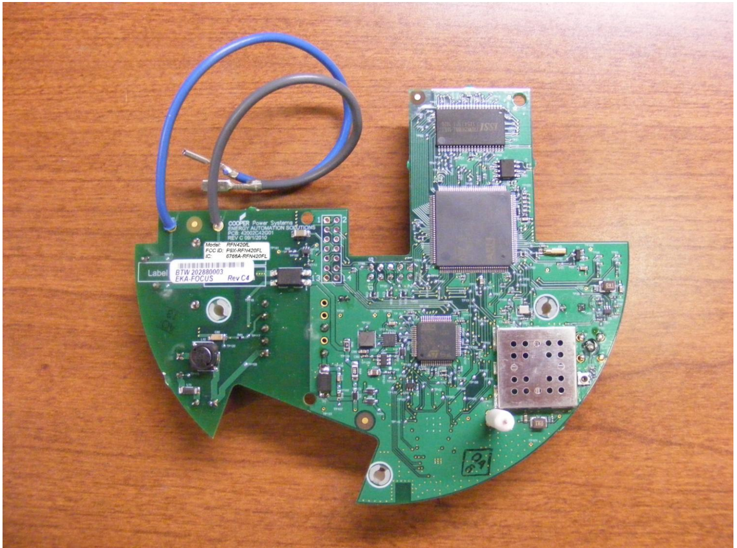
Figure 1: RFN420fL - Top
