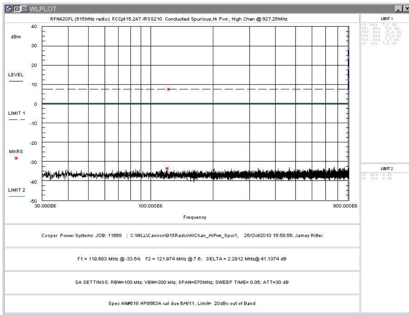
Figure 23: Conducted Spurious Emissions, High Power, High Channel 30 - 900MHz
