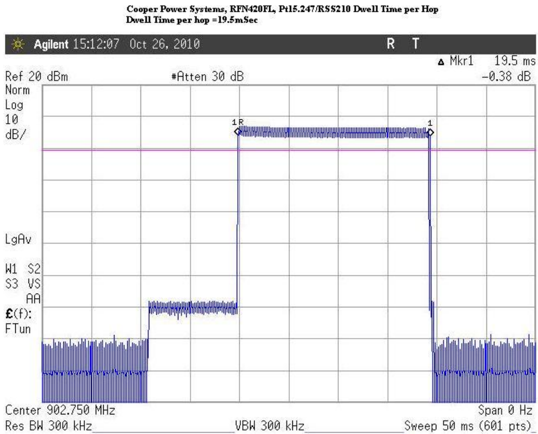
Figure 1: Single Hop Duty Cycle Plot
