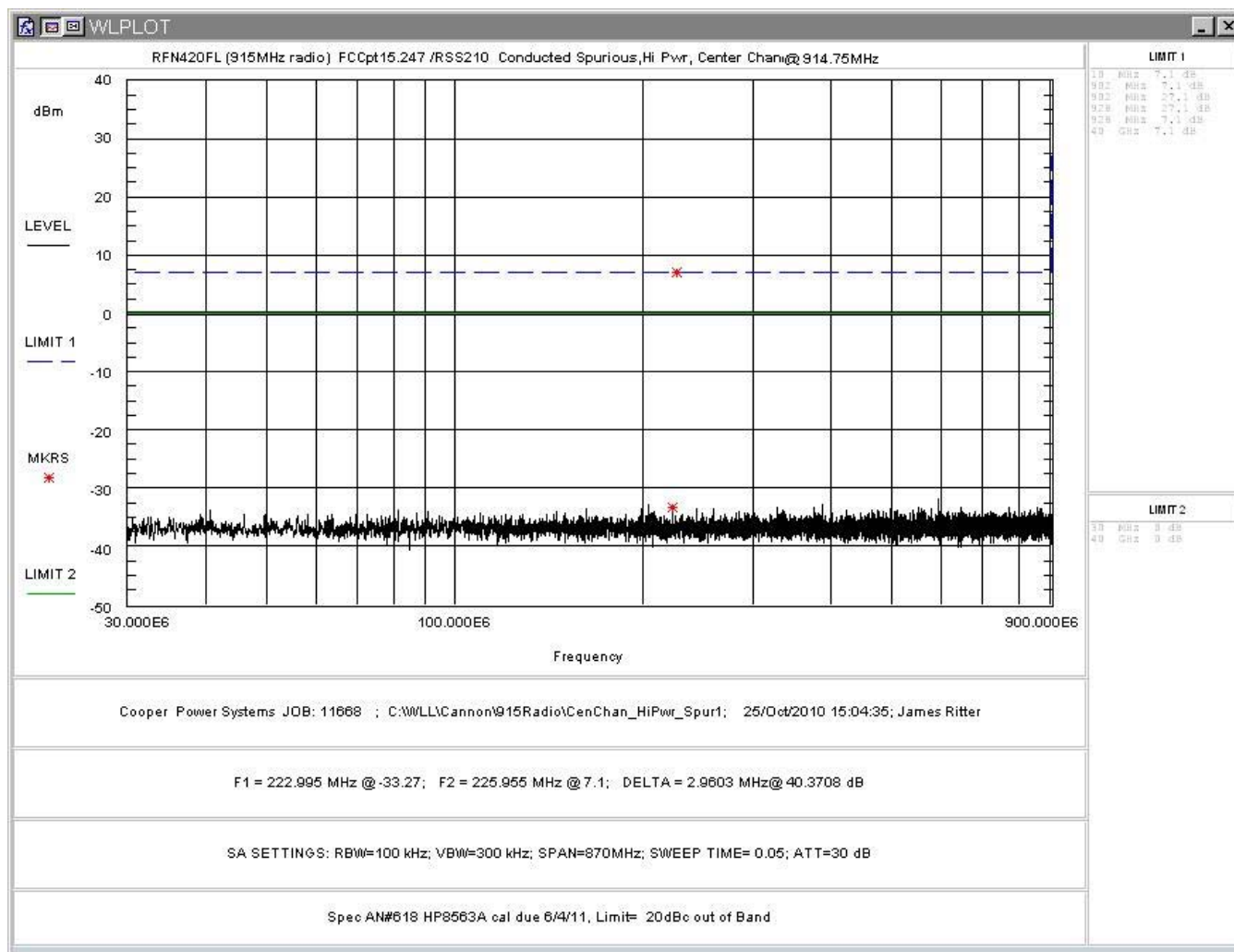
Figure 19: Conducted Spurious Emissions, High Power, Center Channel 30 - 900MHz
