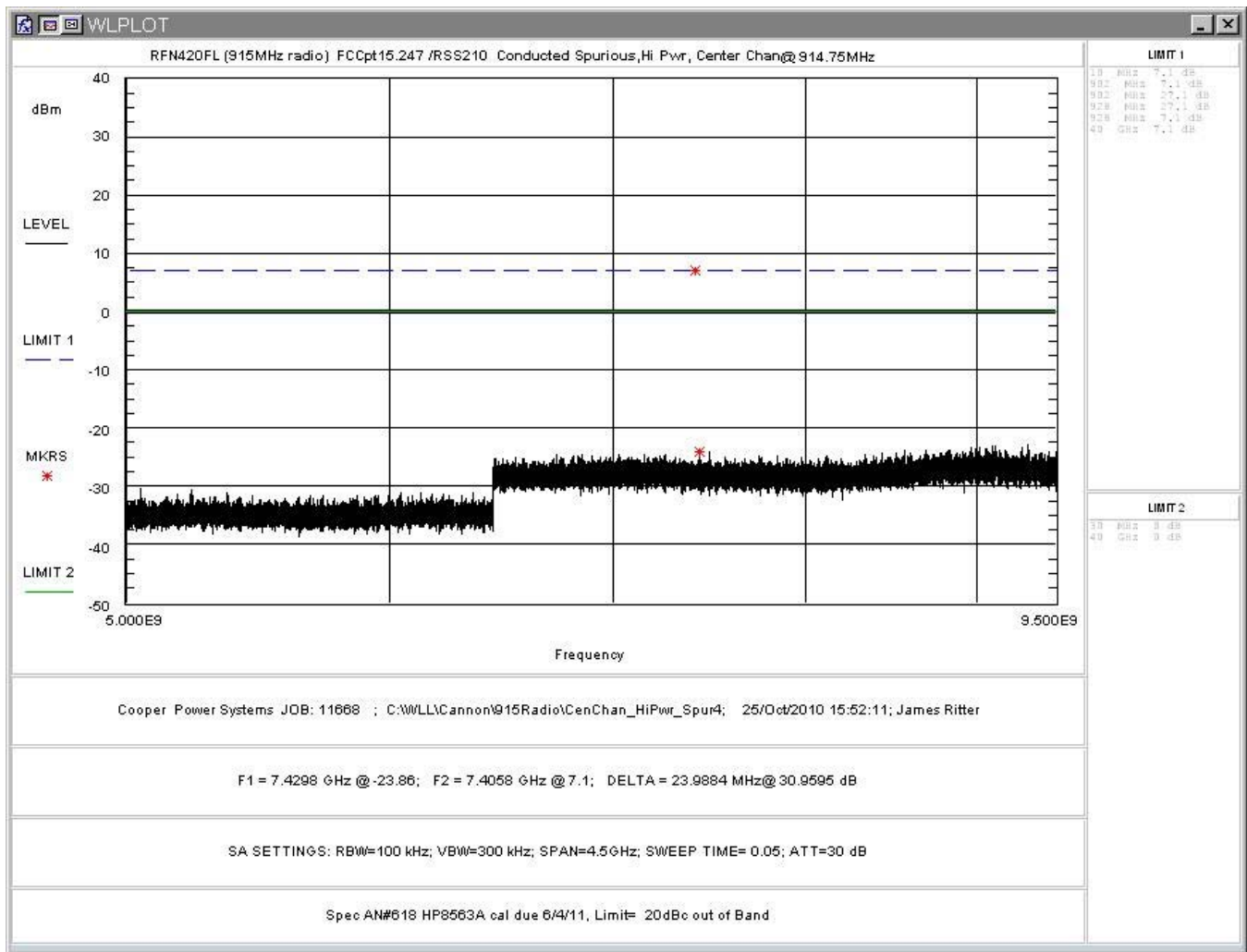
Figure 22: Conducted Spurious Emissions, High Power, Center Channel 5-9.5GHz
