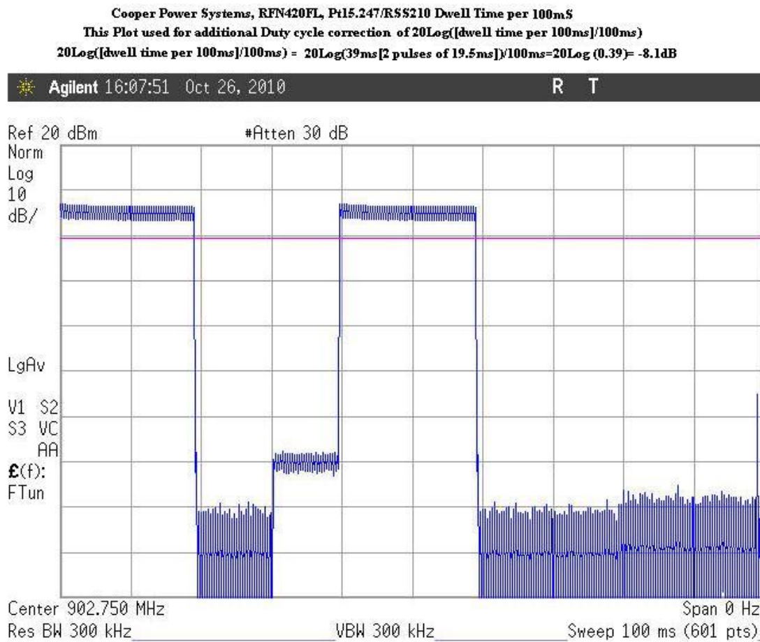
Figure 2: Dwell time per 100ms
