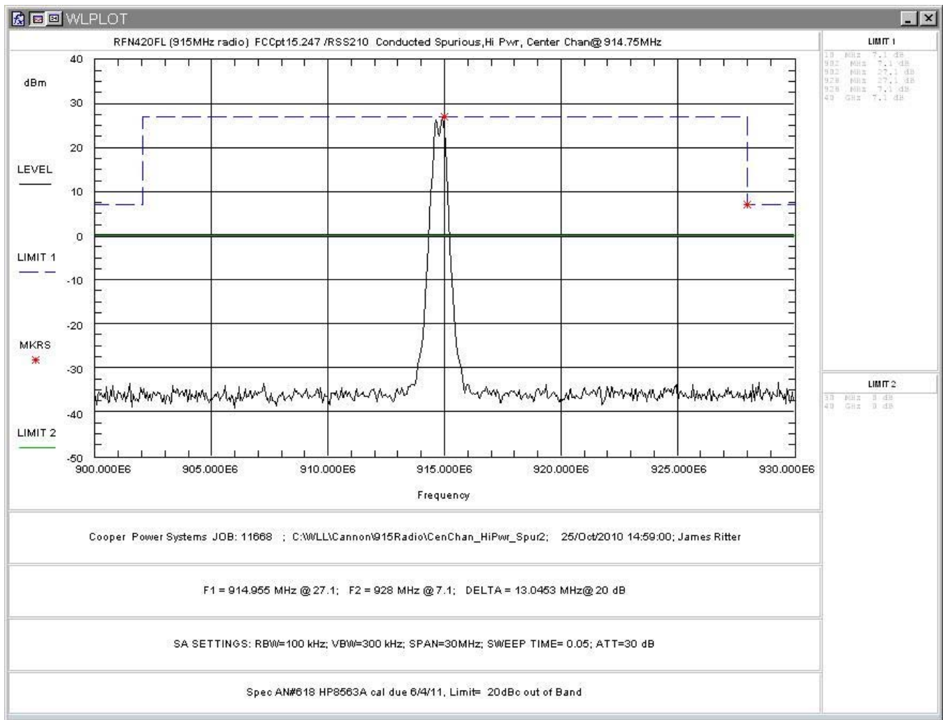
Figure 20: Conducted Spurious Emissions, High Power, Center Channel 900 – 930MHz
