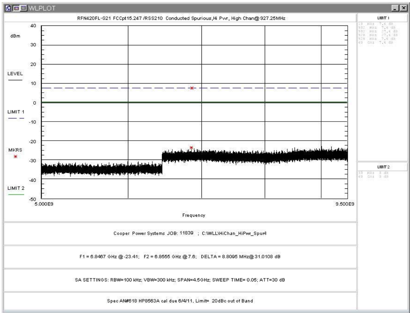
Figure 26: Conducted Spurious Emissions, High Power, High Channel 5-9.5GHz
