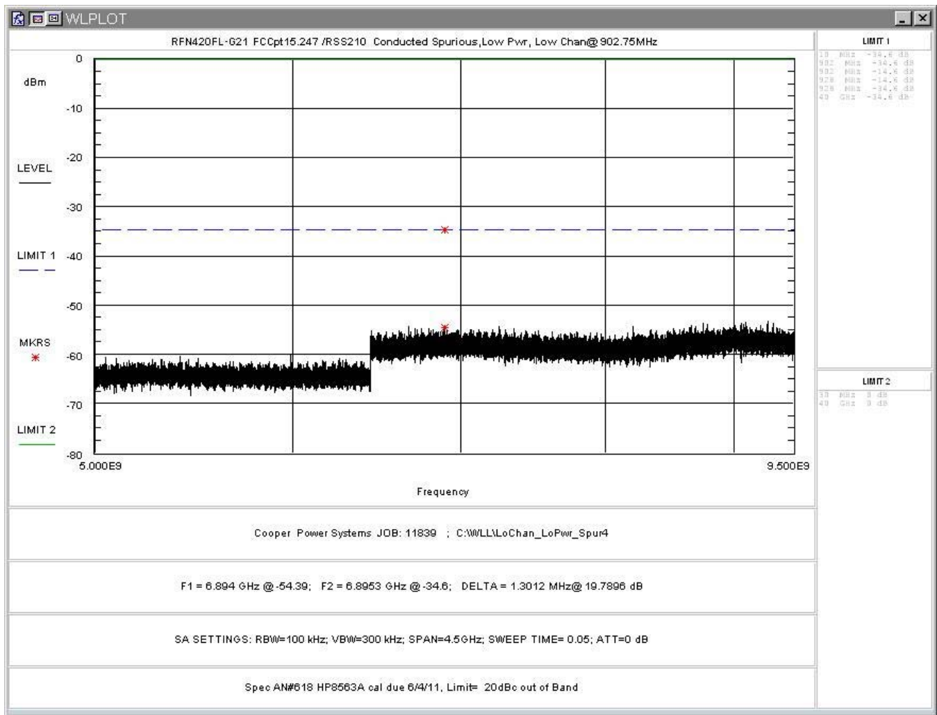
Figure 30: Conducted Spurious Emissions, Low Power, Low Channel 5-9.5GHz
