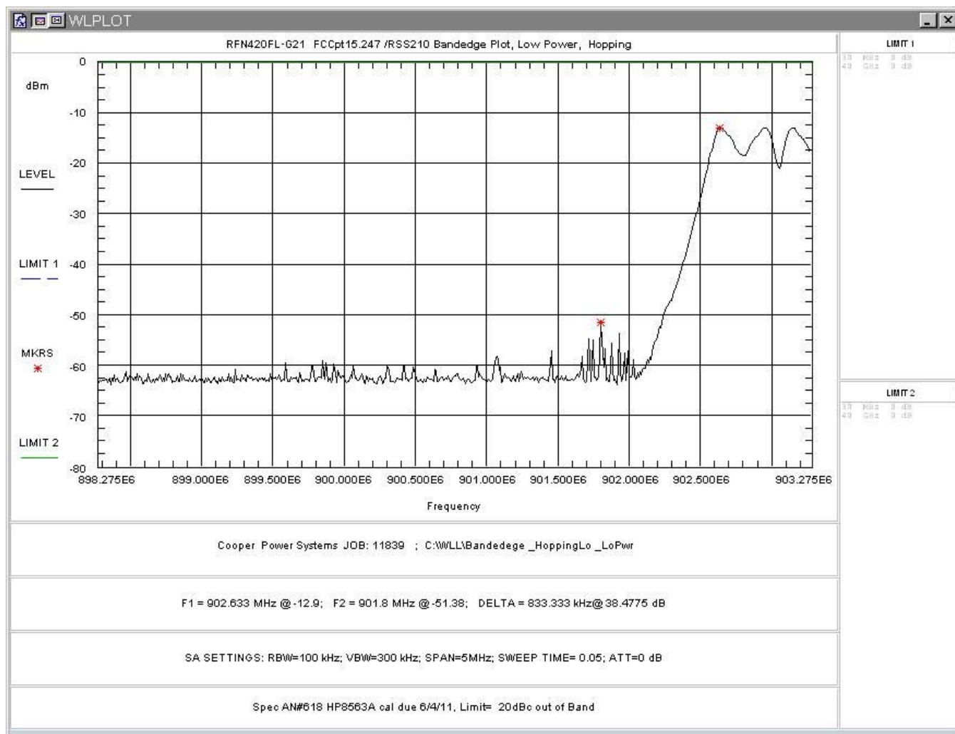
Figure 42: Lower Band-edge, Hopping Mode, Low Power
