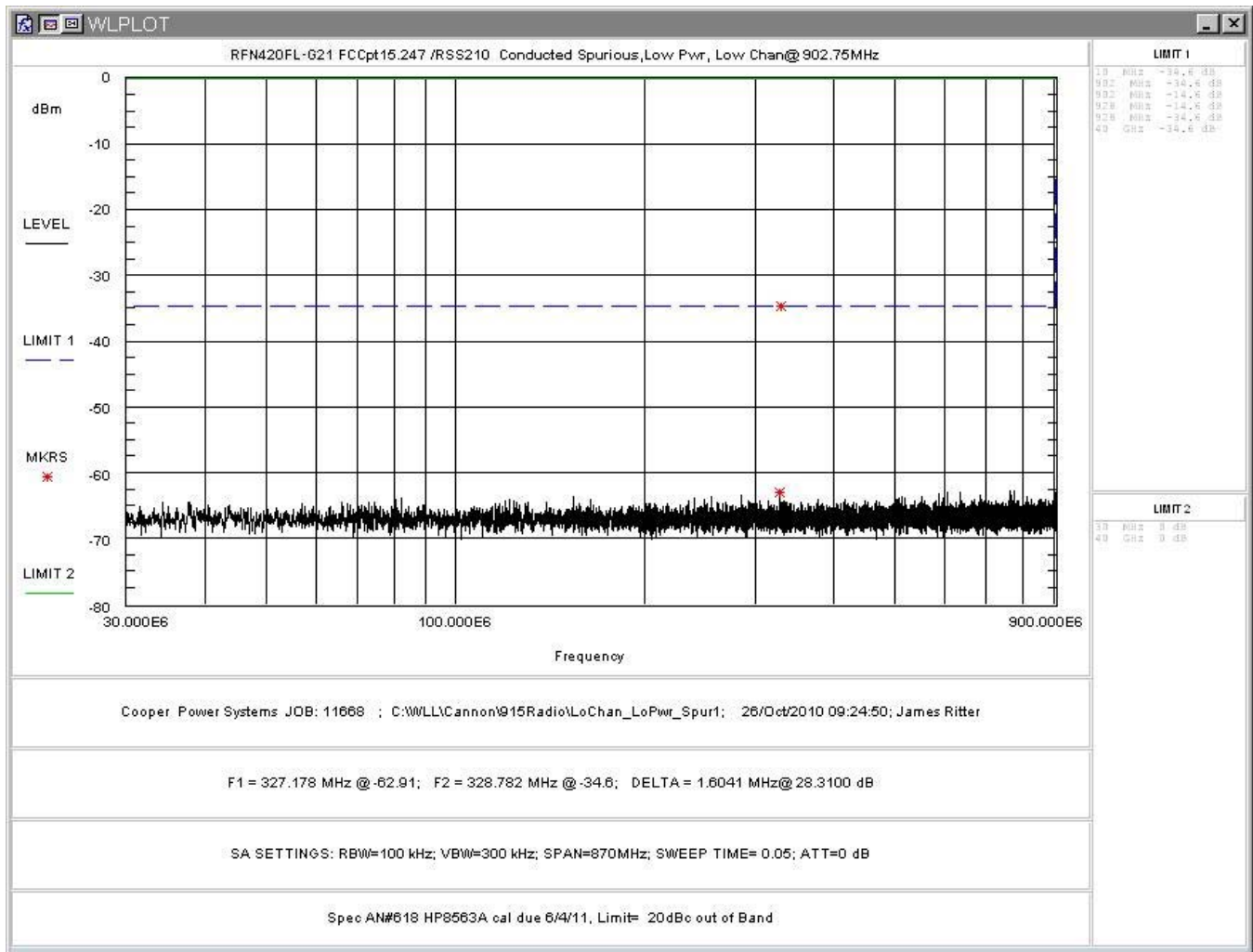
Figure 27: Conducted Spurious Emissions, Low Power, Low Channel 30 - 900MHz
