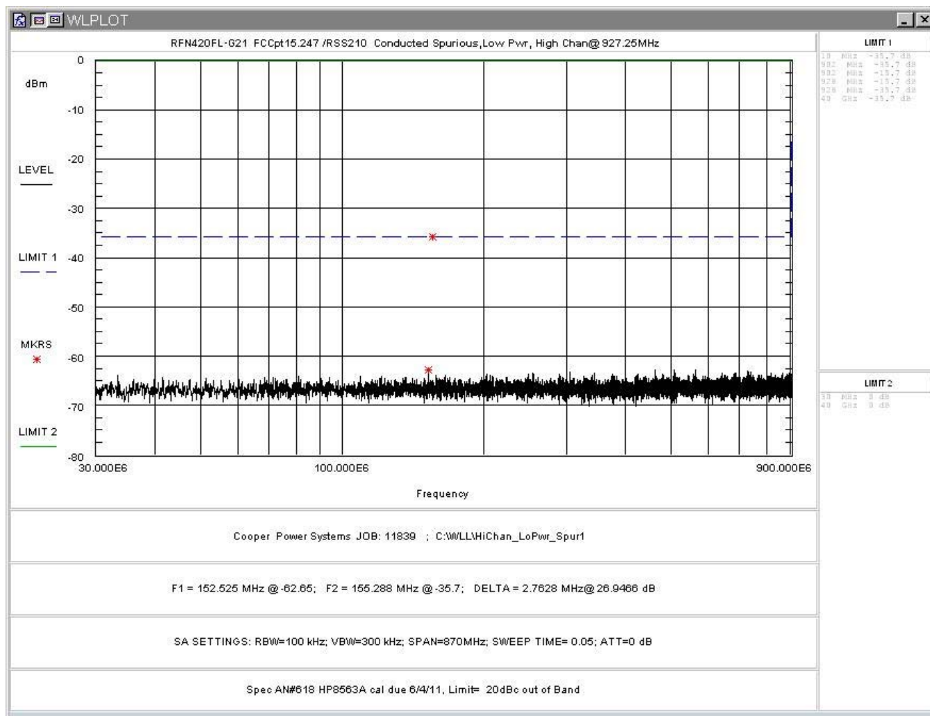
Figure 35: Conducted Spurious Emissions, Low Power, High Channel 30 - 900MHz
