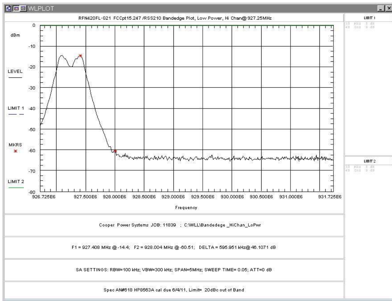
Figure 45: Upper Band-edge, High Channel, Low Power
