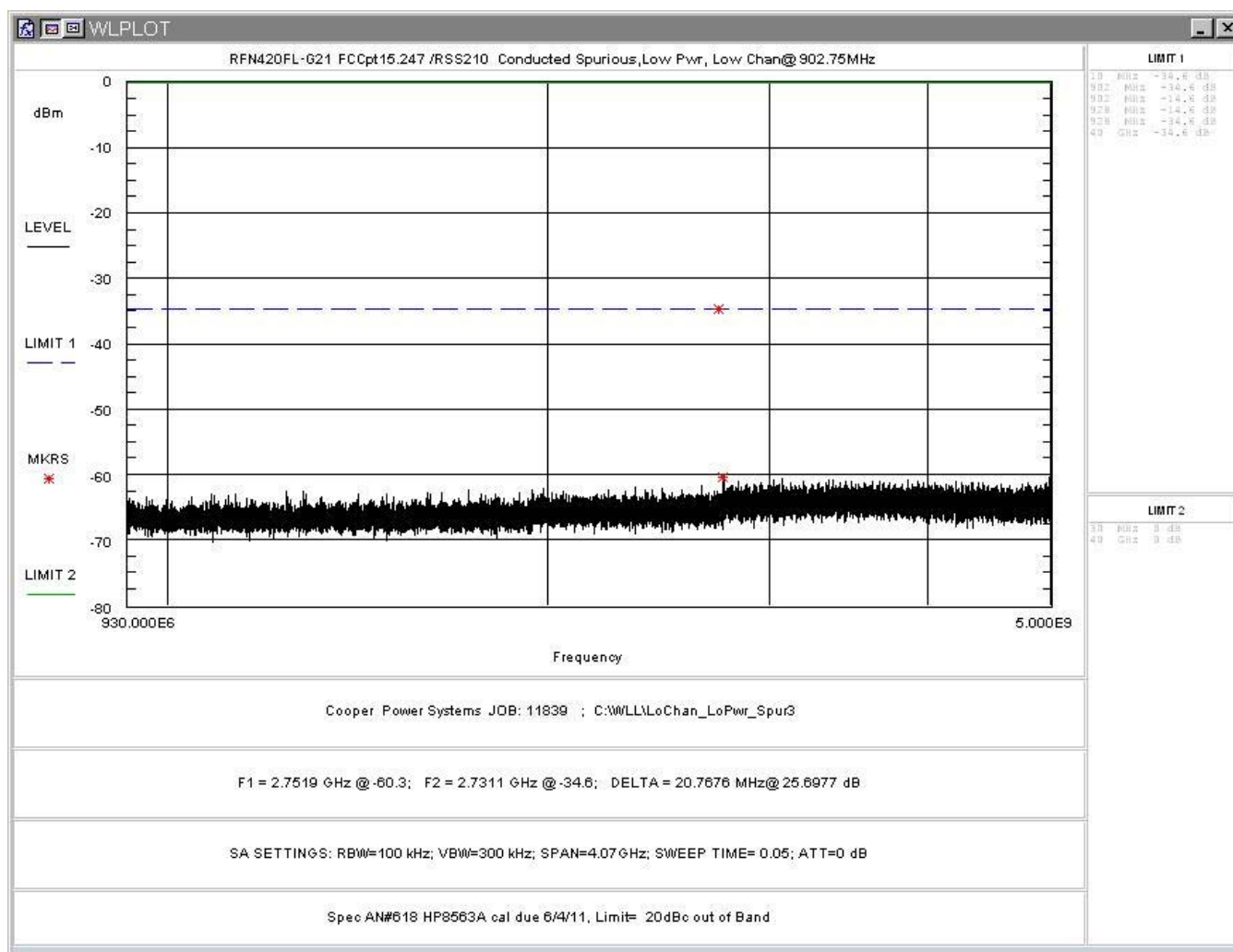
Figure 29: Conducted Spurious Emissions, Low Power, Low Channel 930-5000MHz
