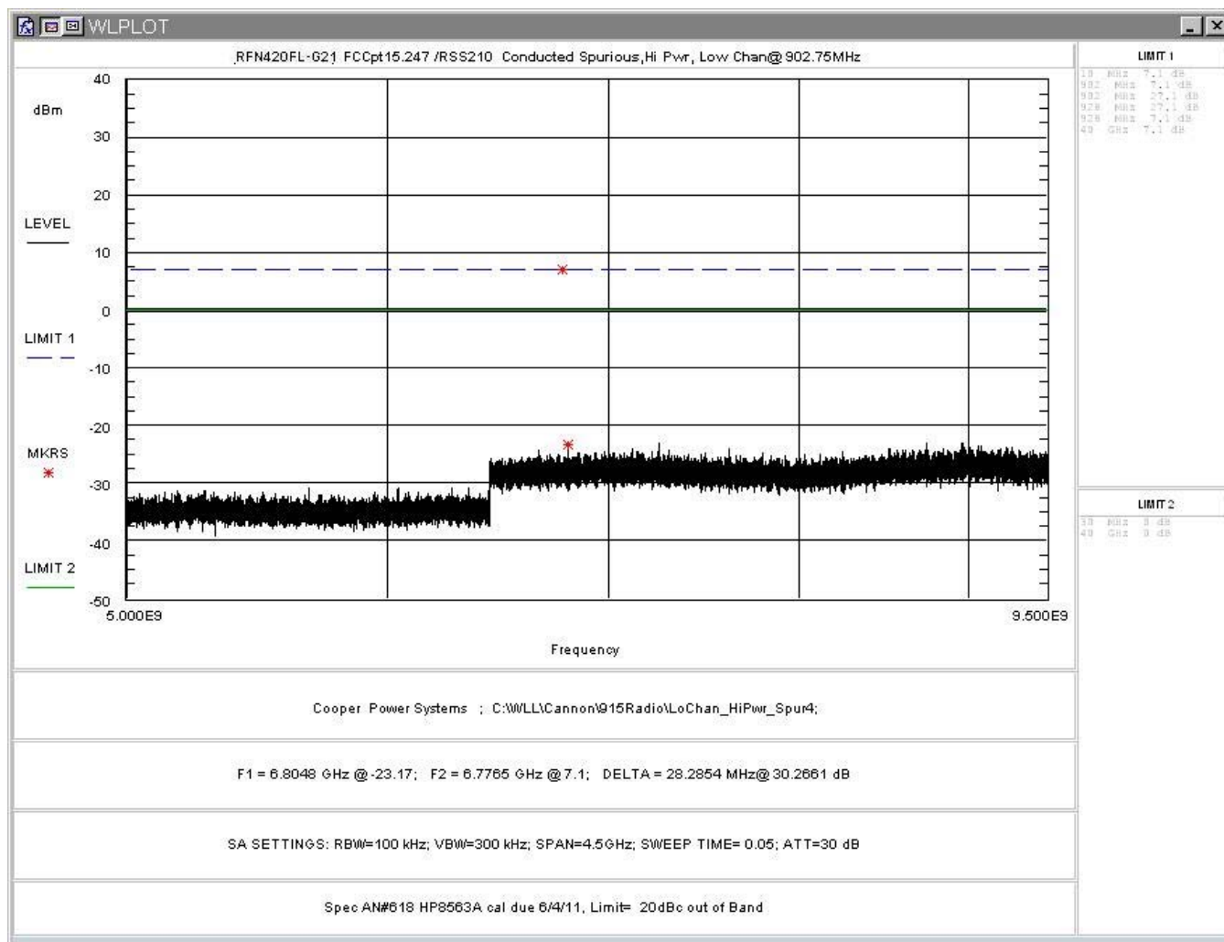
Figure 18: Conducted Spurious Emissions, High Power, Low Channel 5-9.5GHz
