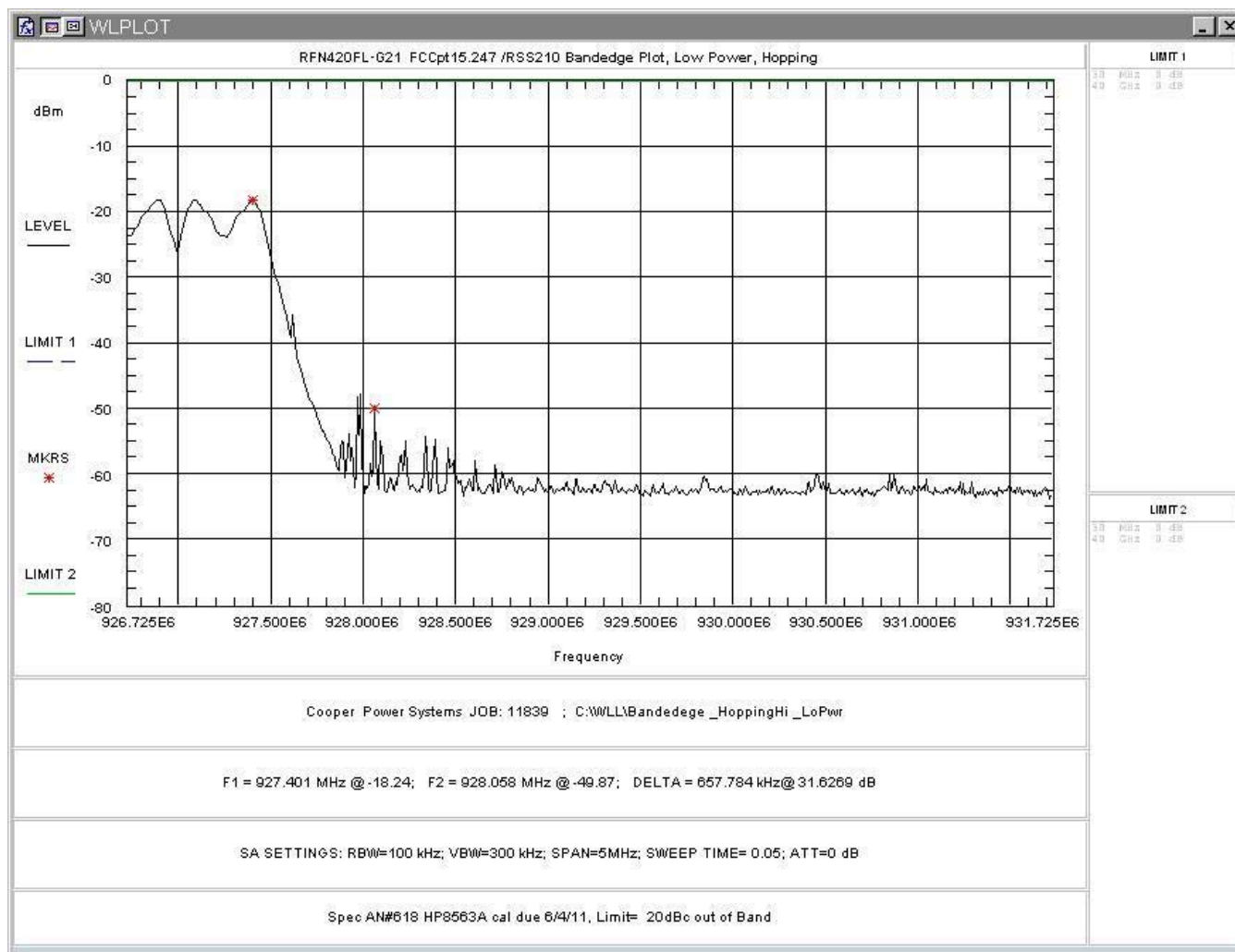
Figure 46: Upper Band-edge, Hopping Mode, Low Power
