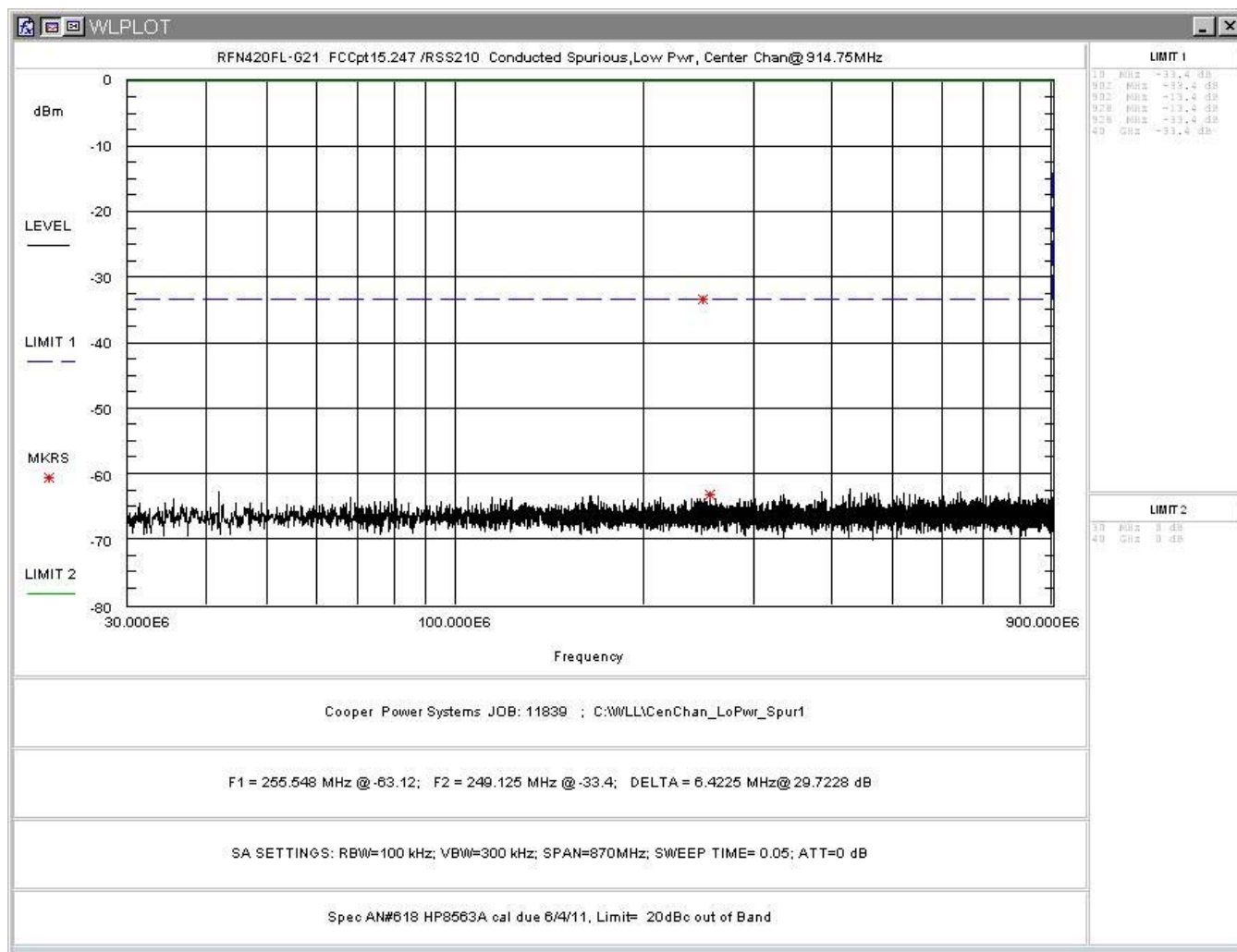
Figure 31: Conducted Spurious Emissions, Low Power, Center Channel 30 - 900MHz
