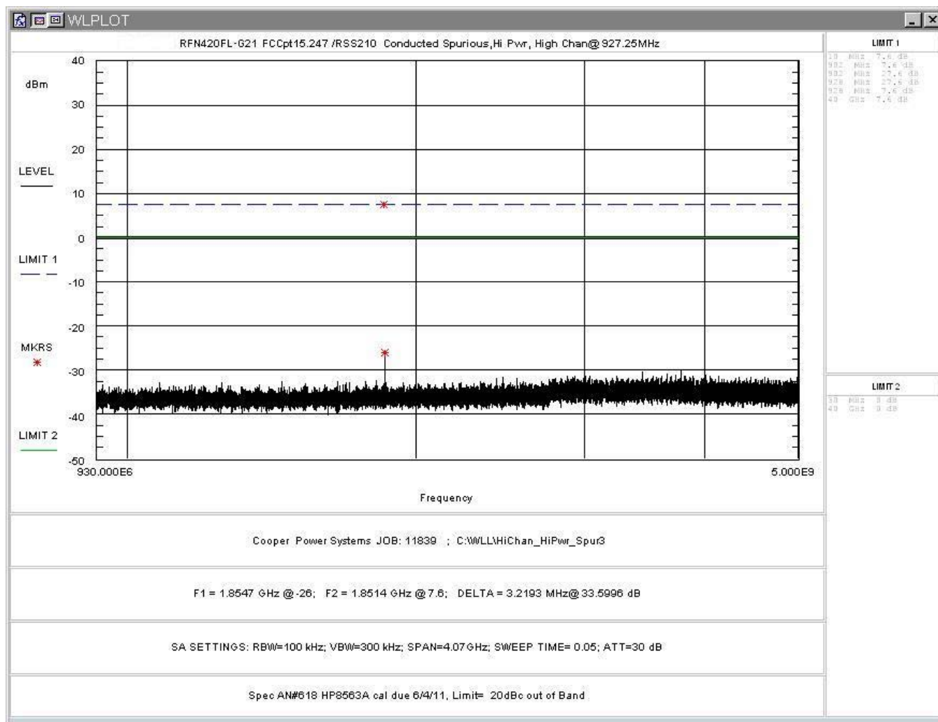
Figure 25: Conducted Spurious Emissions, High Power, High Channel 930-5000MHz
