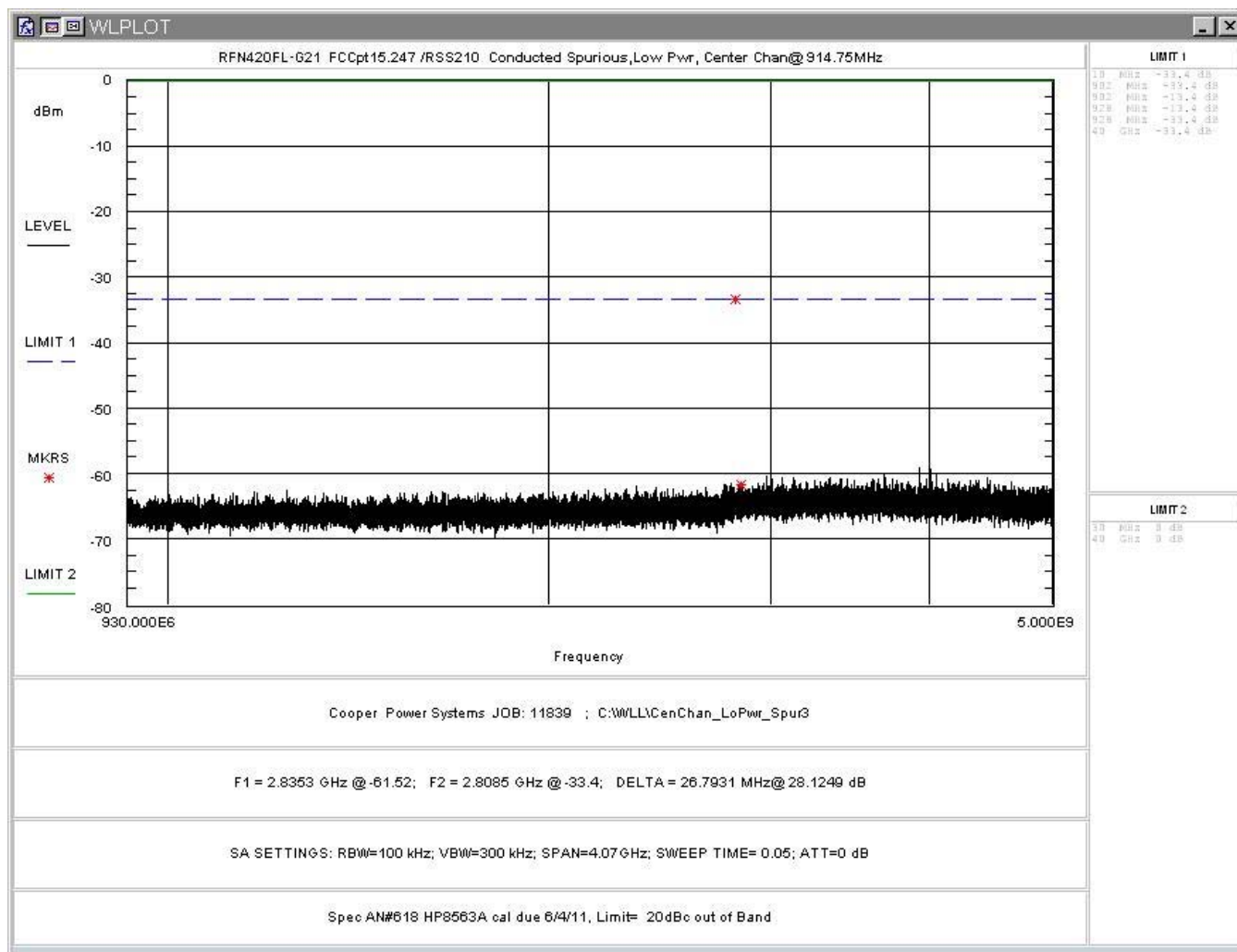
Figure 33: Conducted Spurious Emissions, Low Power, Center Channel 930-5000MHz
