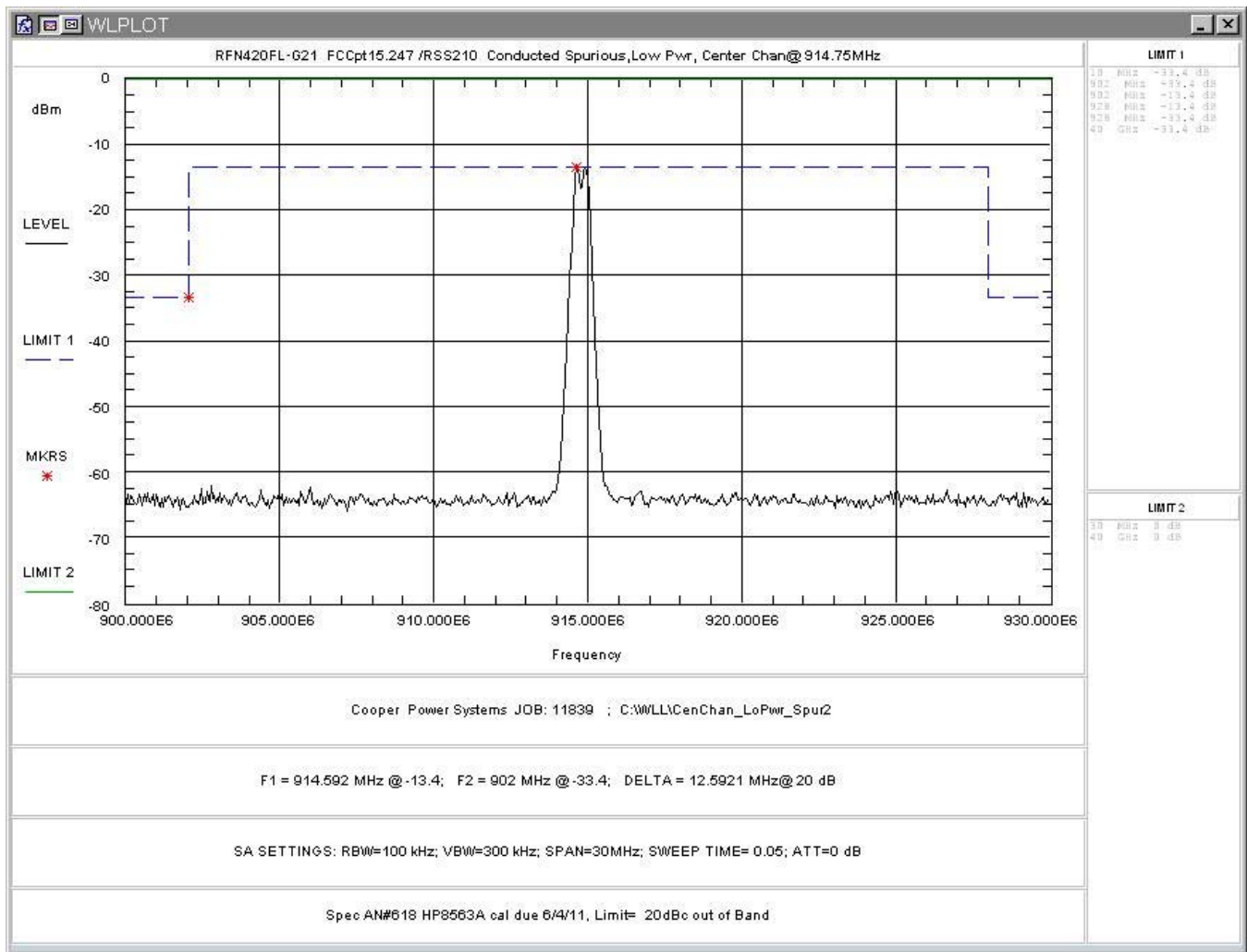
Figure 32: Conducted Spurious Emissions, Low Power, Center Channel 900 – 930MHz
