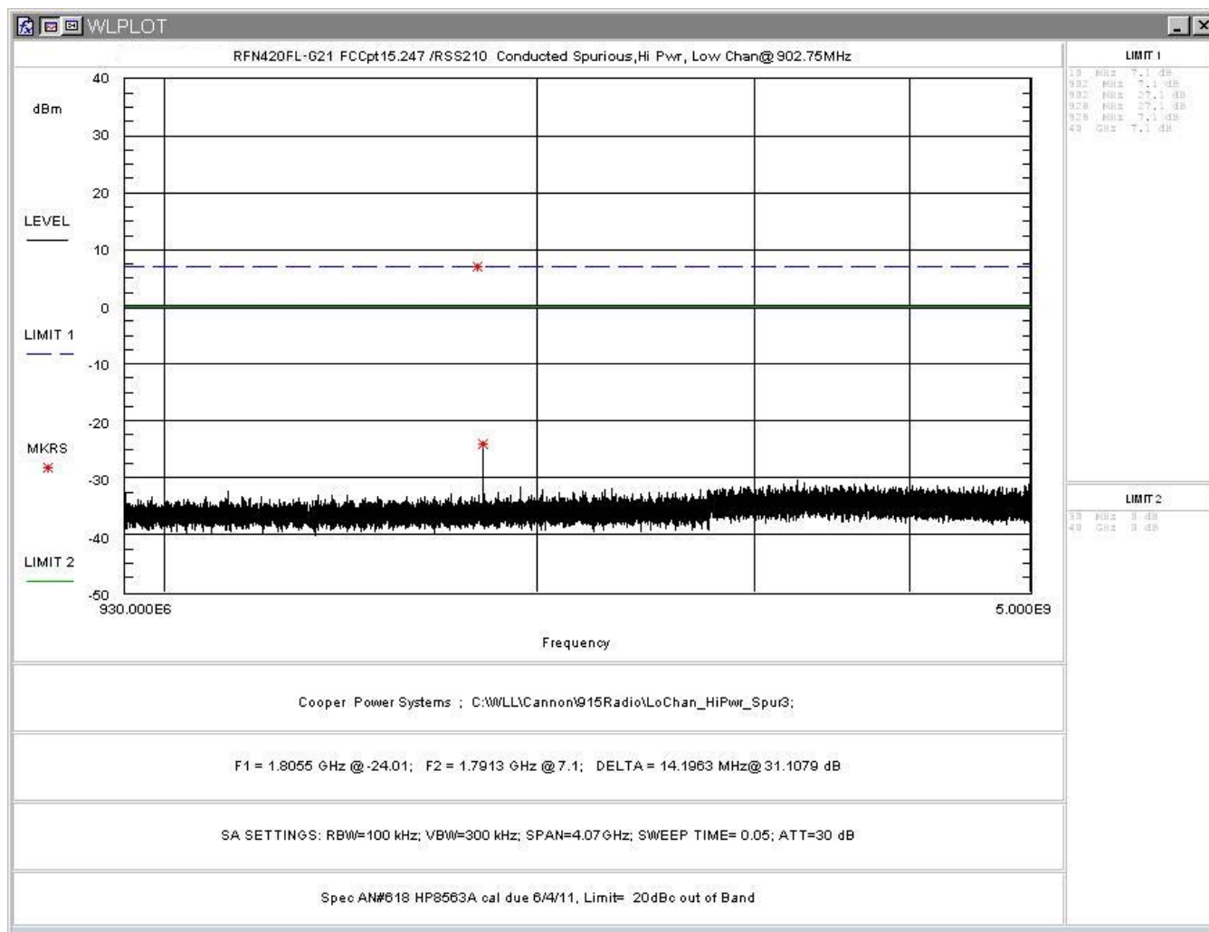
Figure 17: Conducted Spurious Emissions, High Power, Low Channel 930-5000MHz
