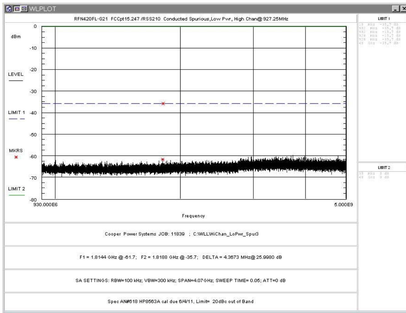
Figure 37: Conducted Spurious Emissions, Low Power, High Channel 930-5000MHz
