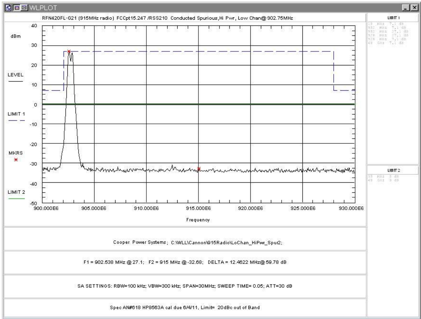
Figure 16: Conducted Spurious Emissions, High Power, Low Channel 900 – 930MHz
