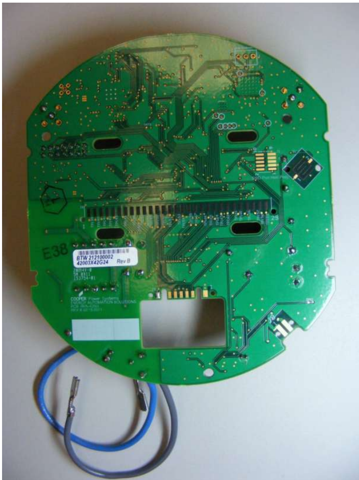
Figure 2: RFN420CL – Bottom
