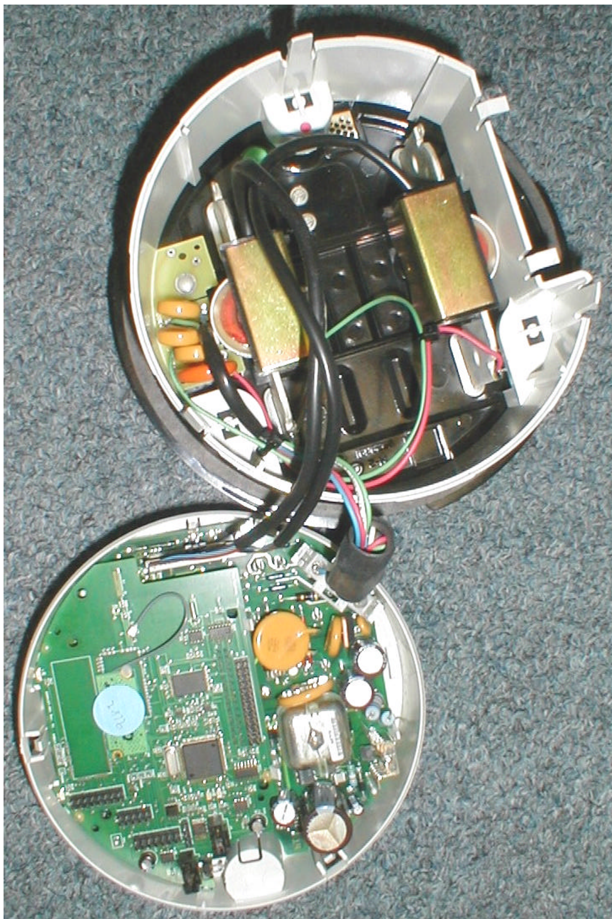
Interior of Meter with Eka Tx Module In Place
