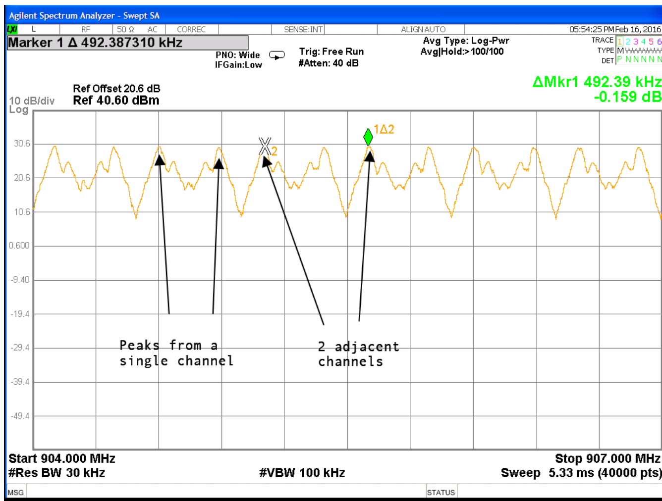
Figure 13: Channel Spacing
