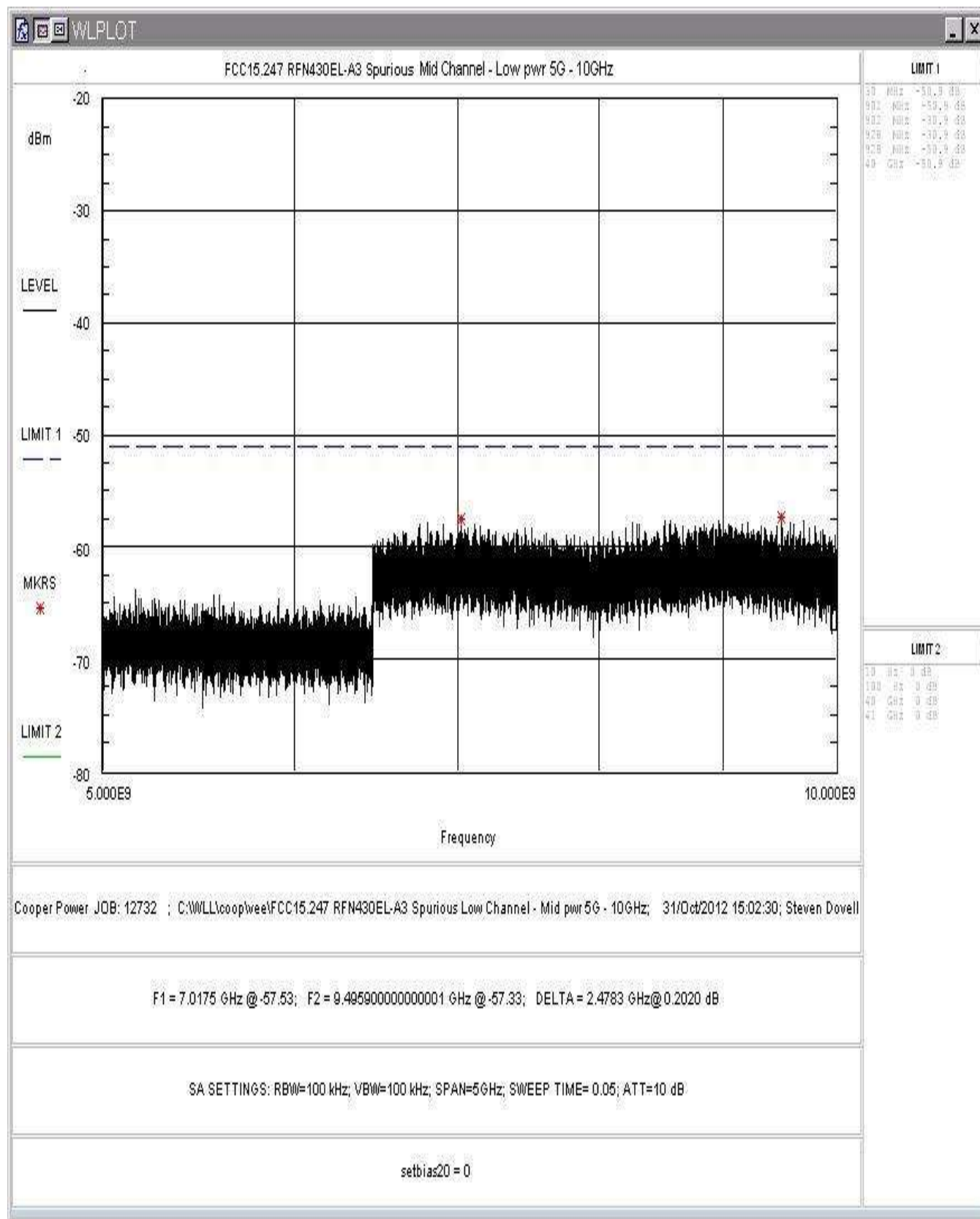
Figure 34: Conducted Spurious Emissions, Low Power, Center Channel 5-10GHz
