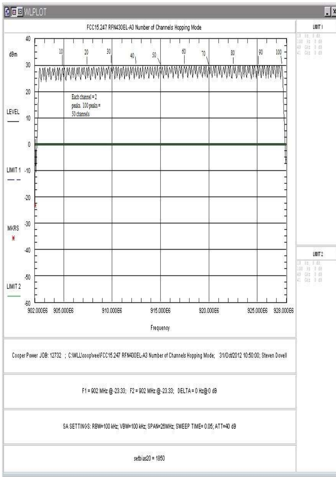
Figure 14: Number of Hopping Channels
