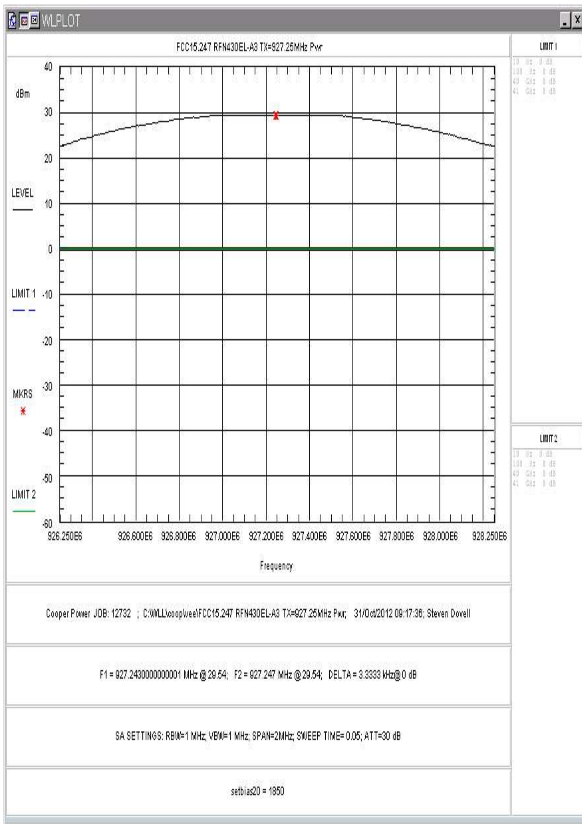
Figure 6: RF Peak Power, High Power, High Channel
