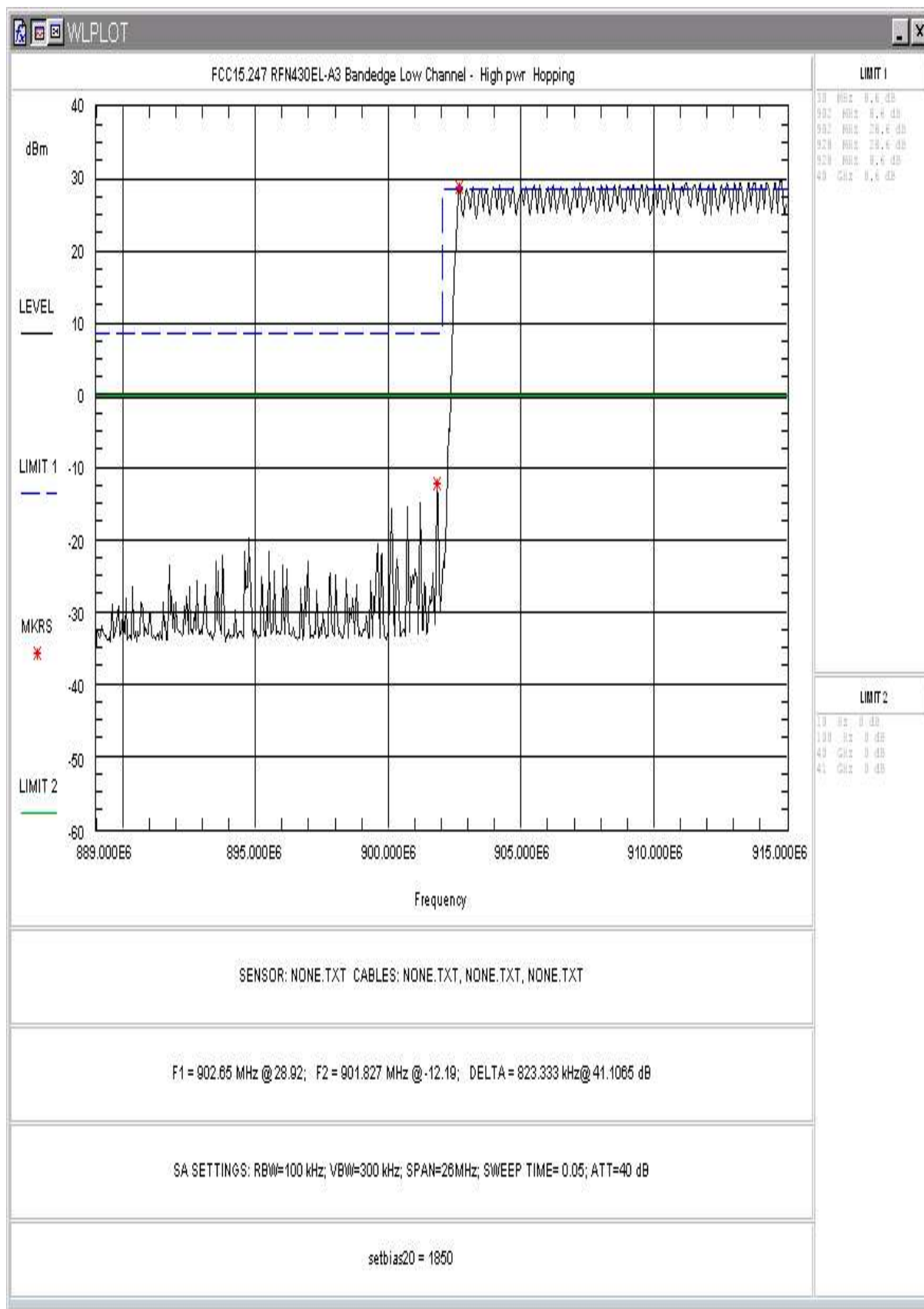
Figure 40: Lower Band-edge, Hopping Mode, High Power
