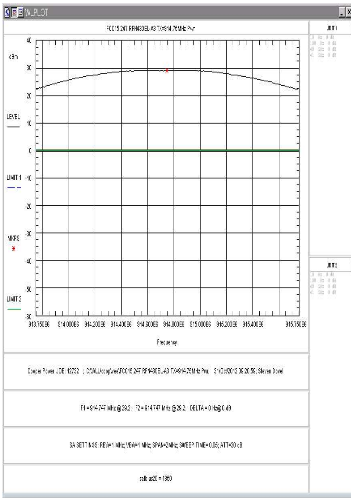
Figure 5: RF Peak Power, High Power, Center Channel
