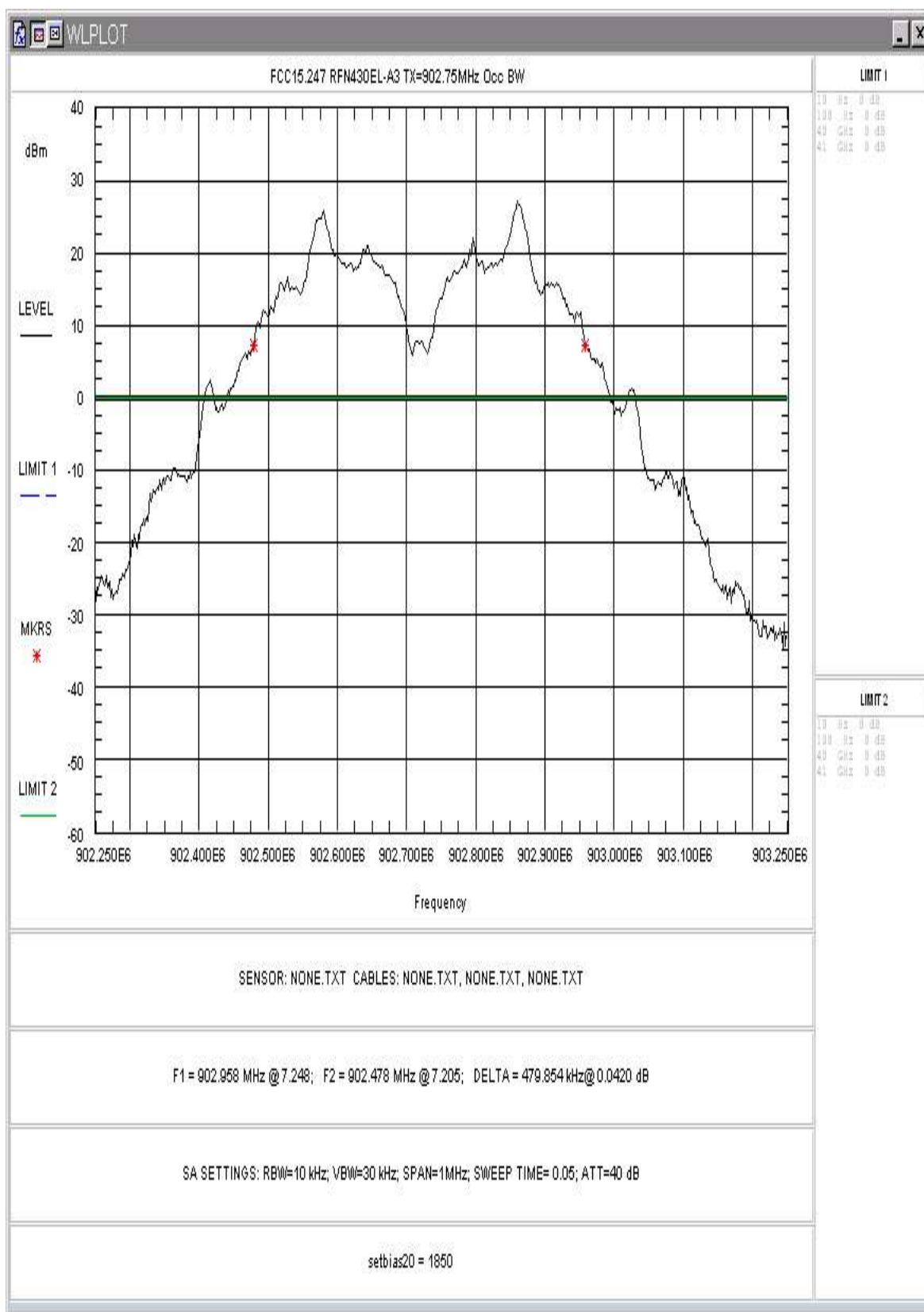
Figure 10: Occupied Bandwidth, Low Channel
