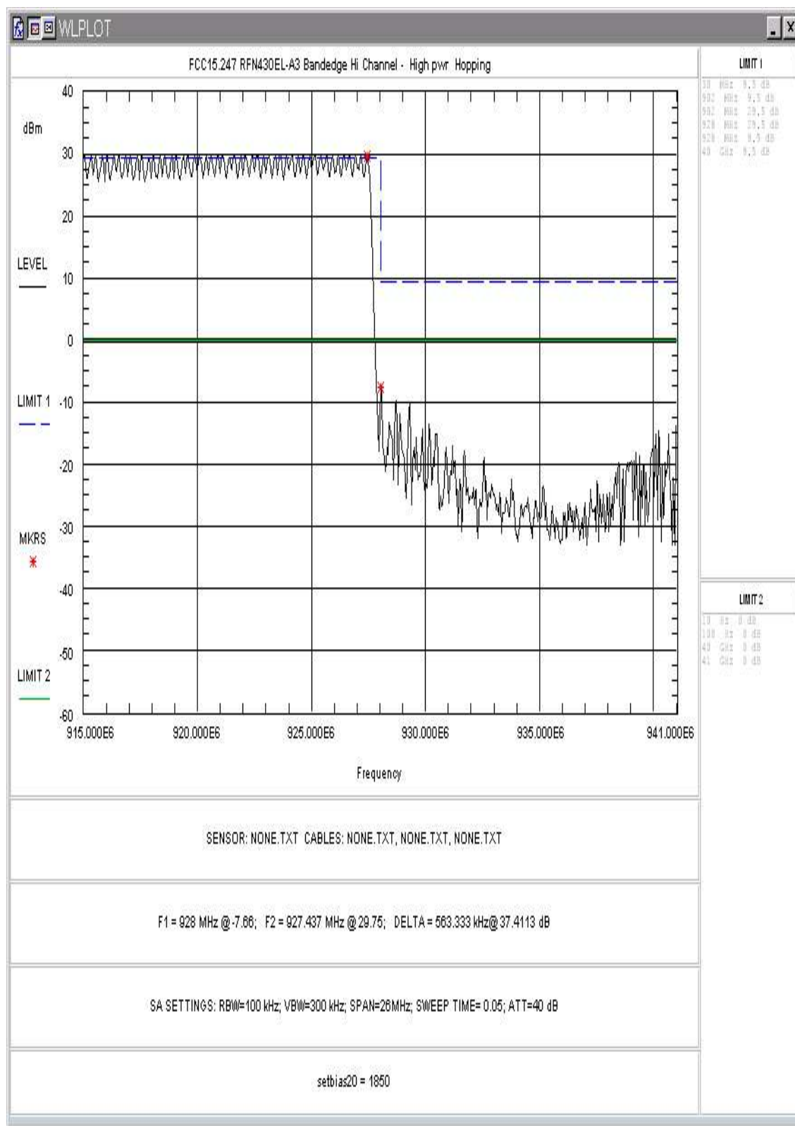
Figure 44: Upper Band-edge, Hopping Mode, High Power
