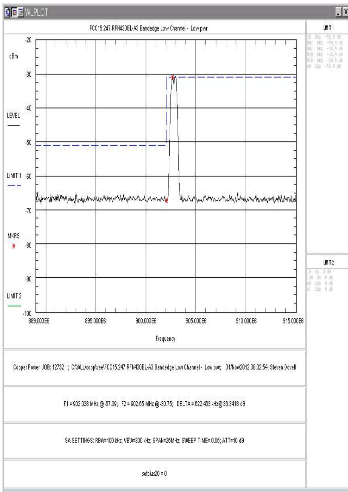
Figure 41: Lower Band-edge, Low Channel, Low Power
