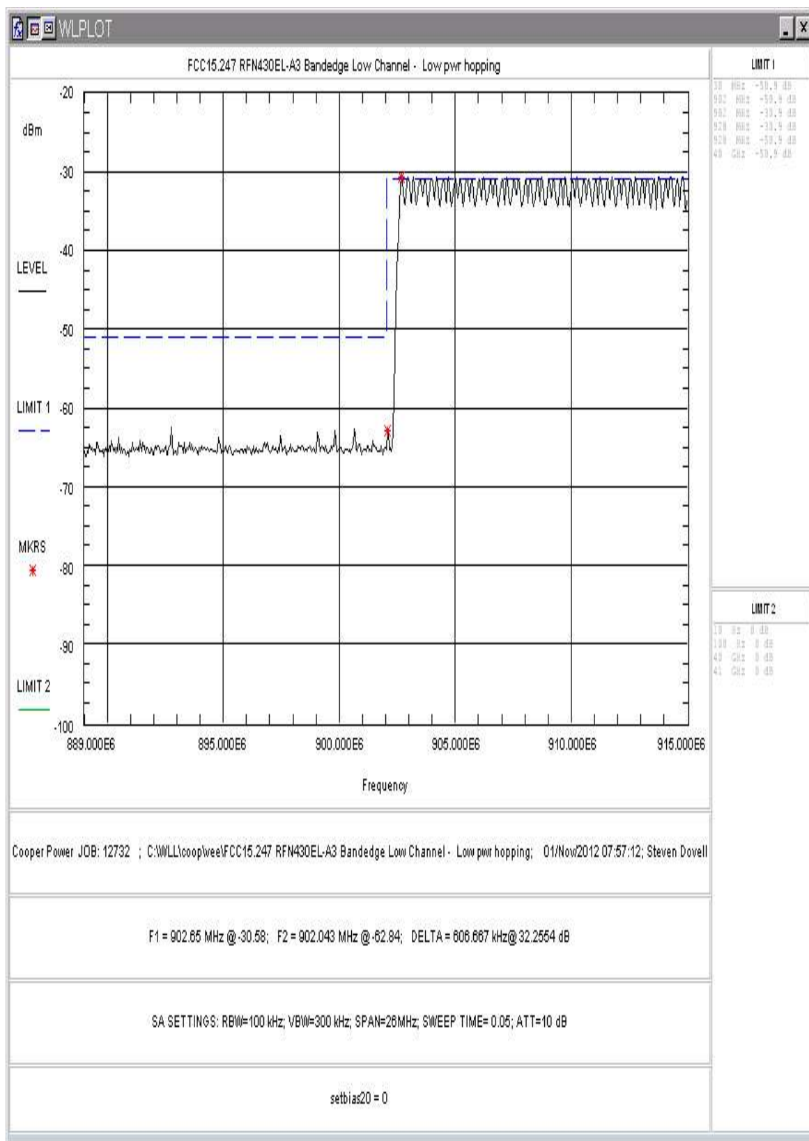
Figure 42: Lower Band-edge, Hopping Mode, Low Power
