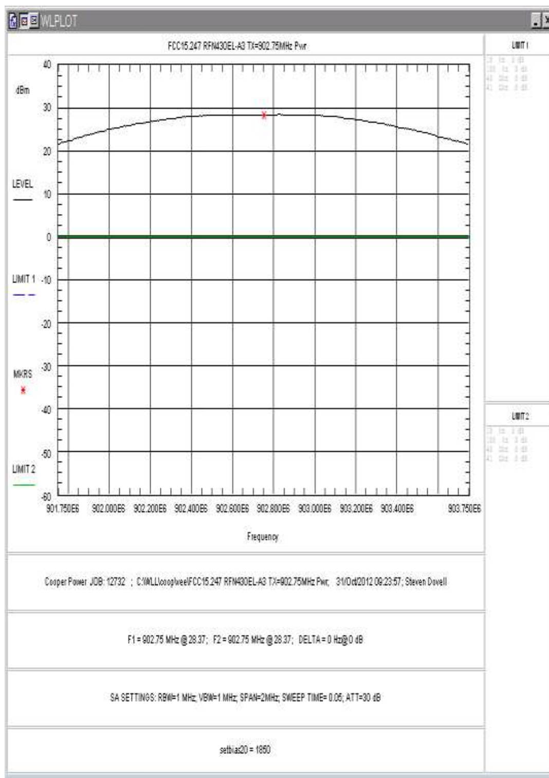
Figure 4: RF Peak Power, High Power, Low Channel
