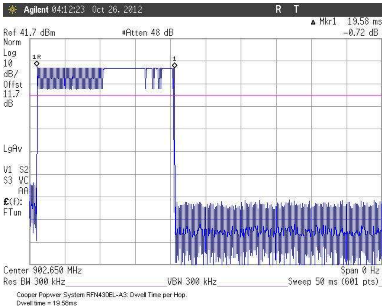
Figure 1: Single Hop Duty Cycle Plot
