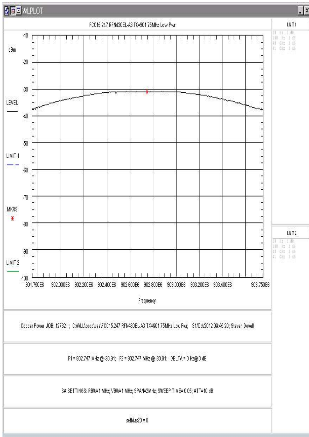
Figure 7: RF Peak Power, Low Power, Low Channel
