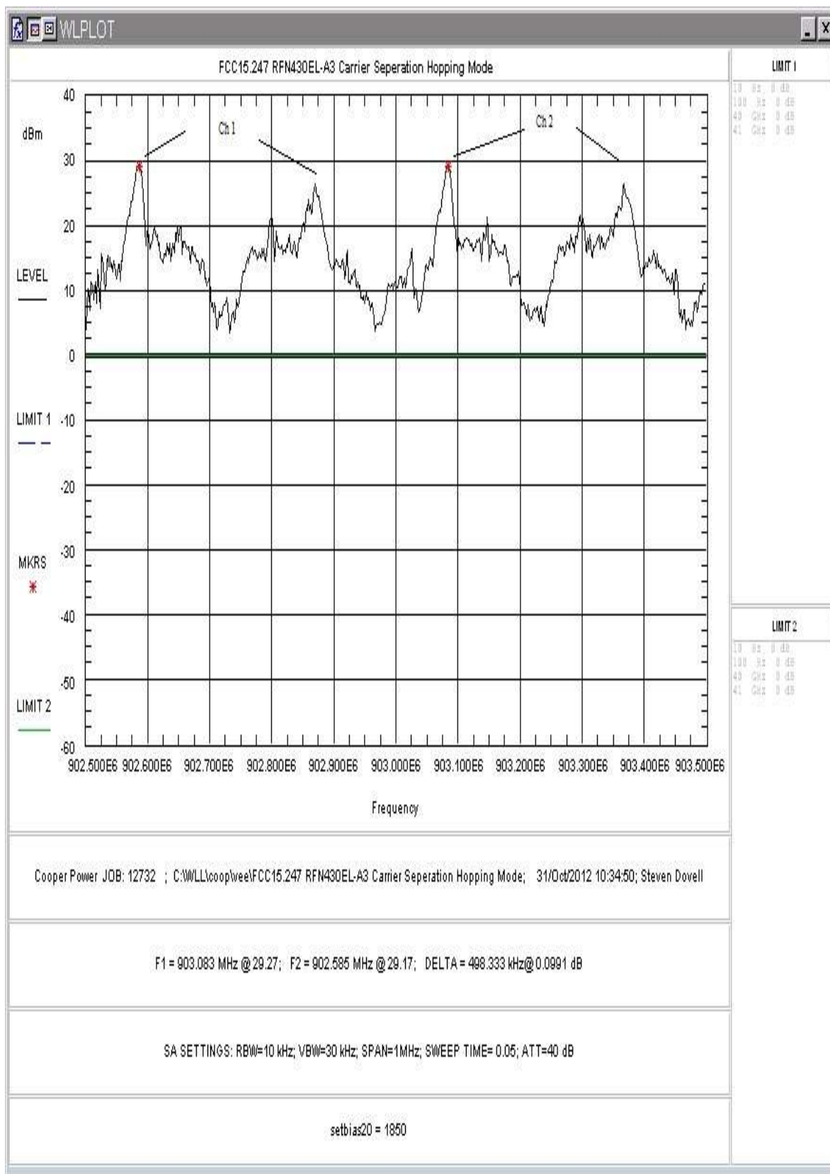
Figure 13: Channel Spacing
