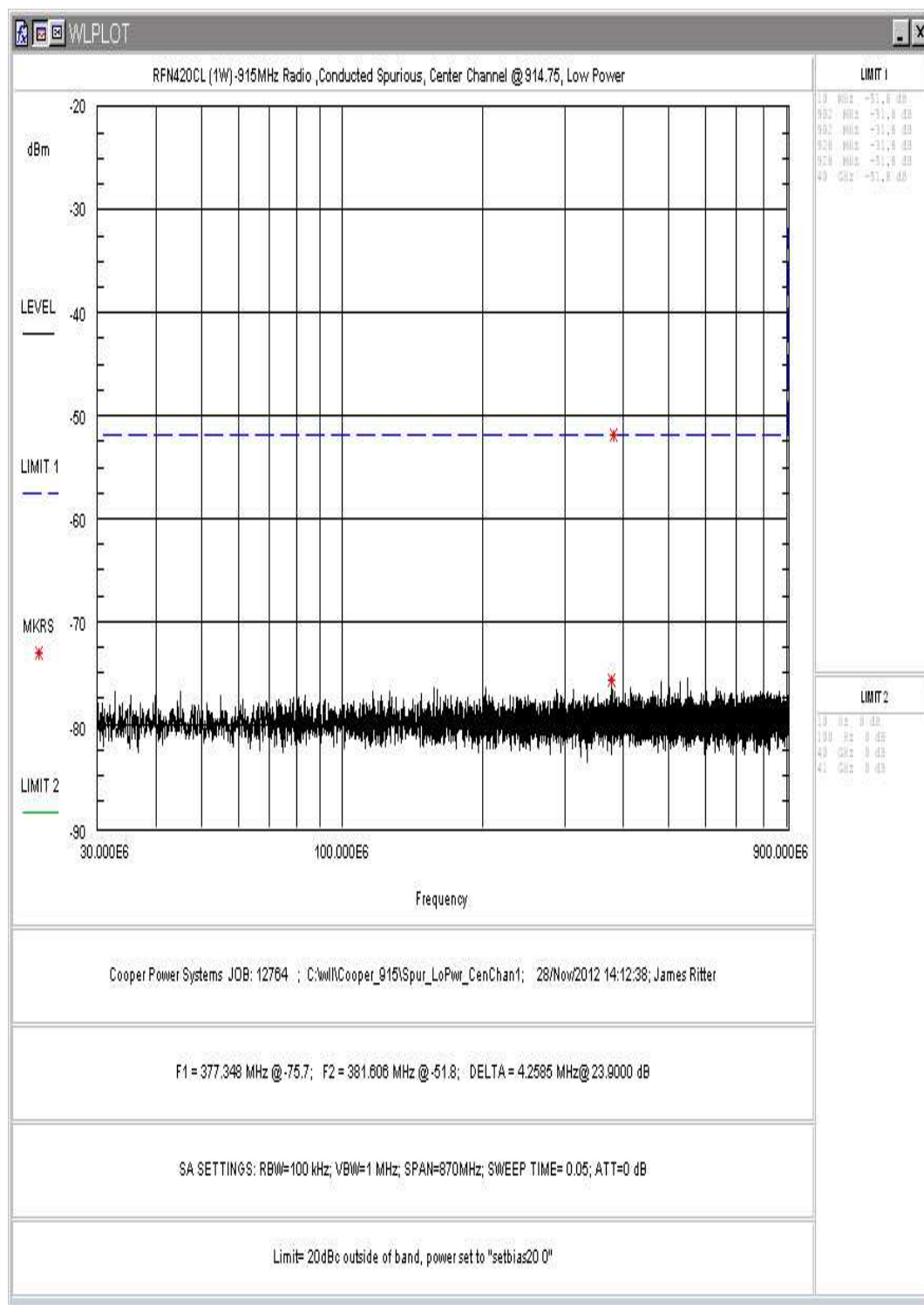
Figure 31: Conducted Spurious Emissions, Low Power, Center Channel 30 - 900MHz
