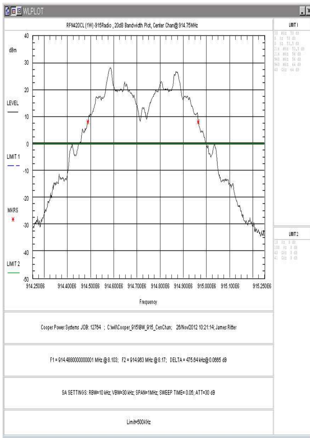
Figure 11: Occupied Bandwidth, Center Channel
