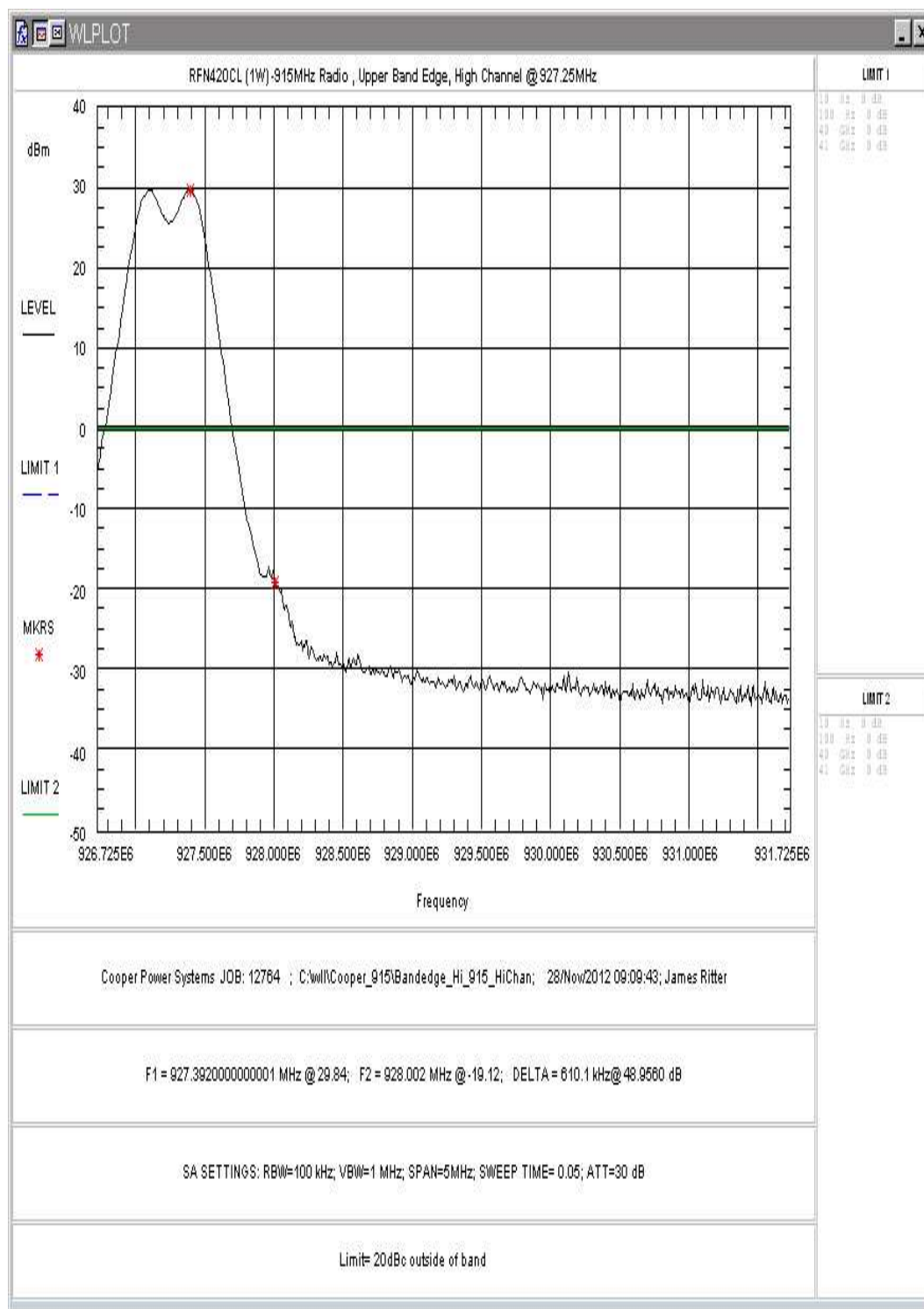
Figure 43: Upper Band-edge, High Channel, High Power
