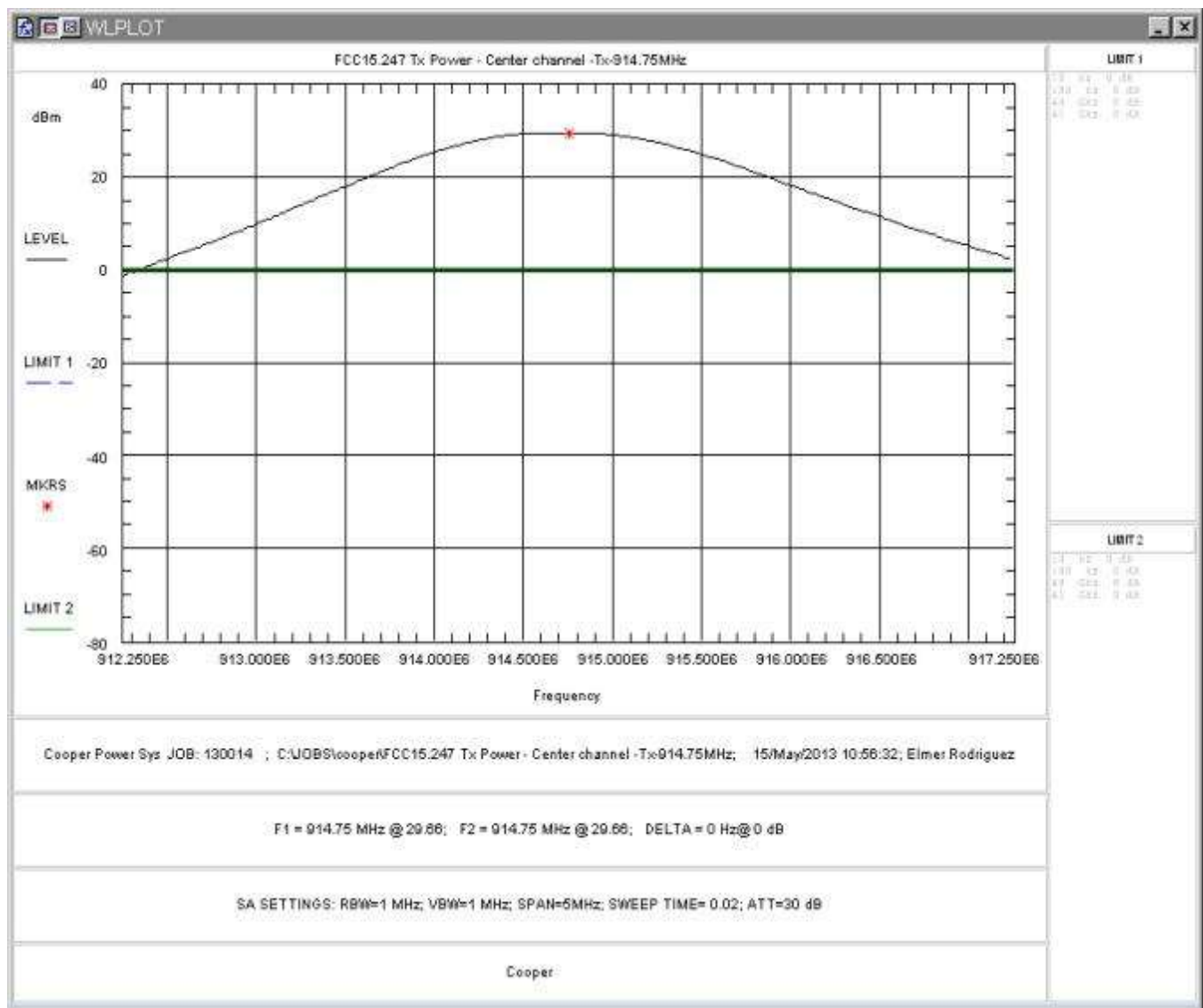
Figure 5: RF Peak Power, High Power, Center Channel
