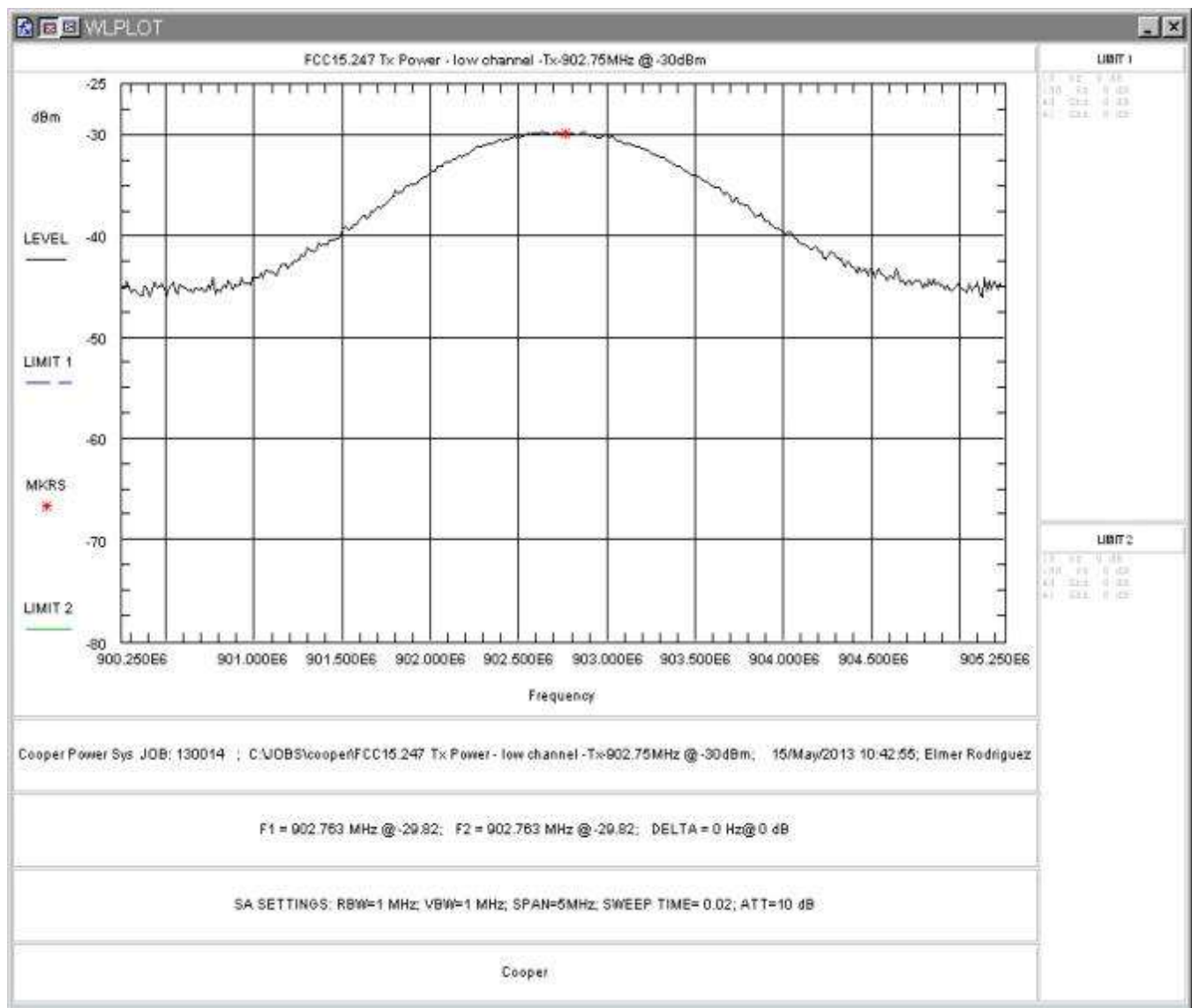
Figure 7: RF Peak Power, Low Power, Low Channel
