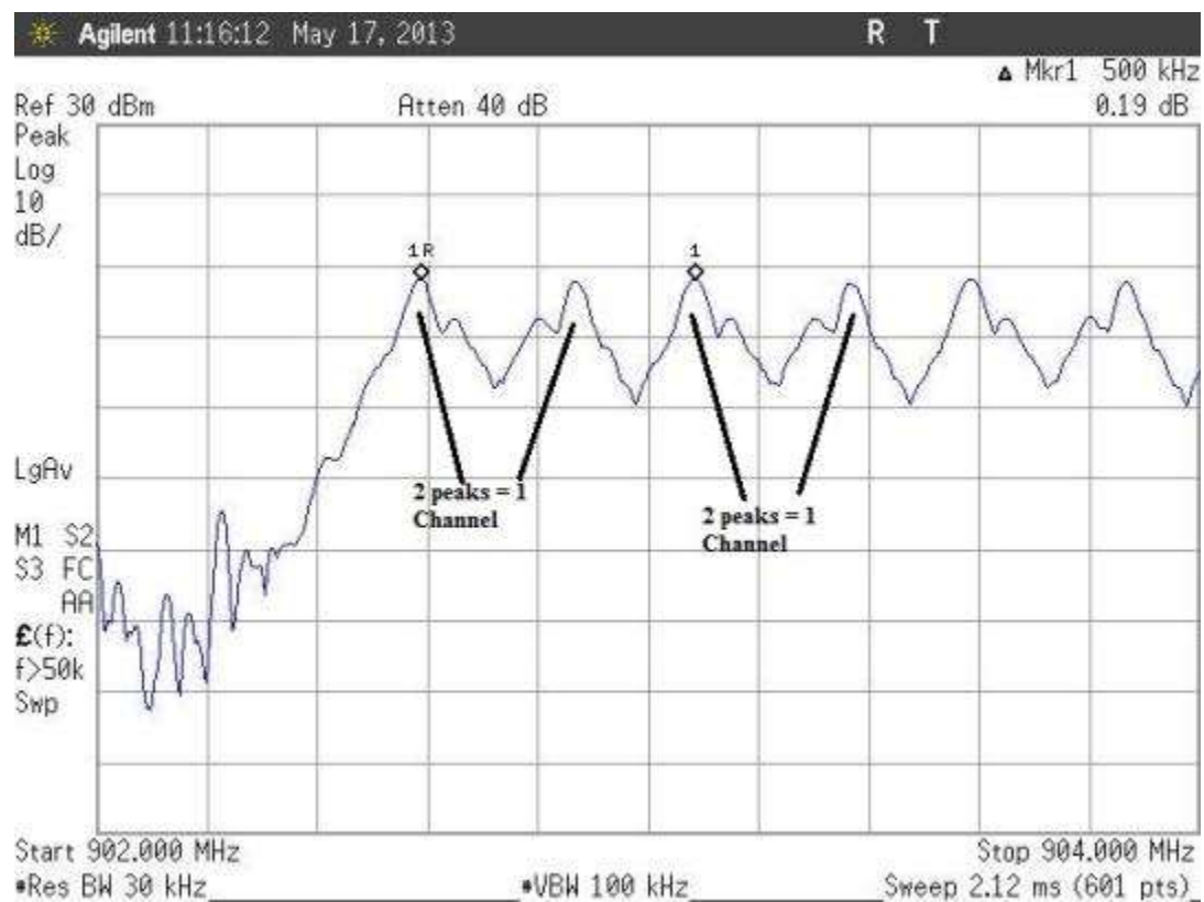
Figure 13: Channel Spacing
