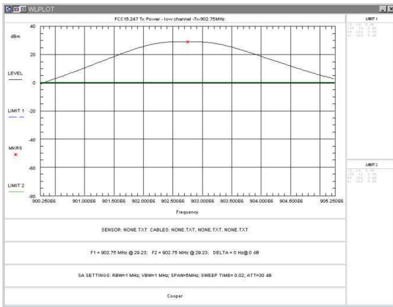
Figure 4: RF Peak Power, High Power, Low Channel
