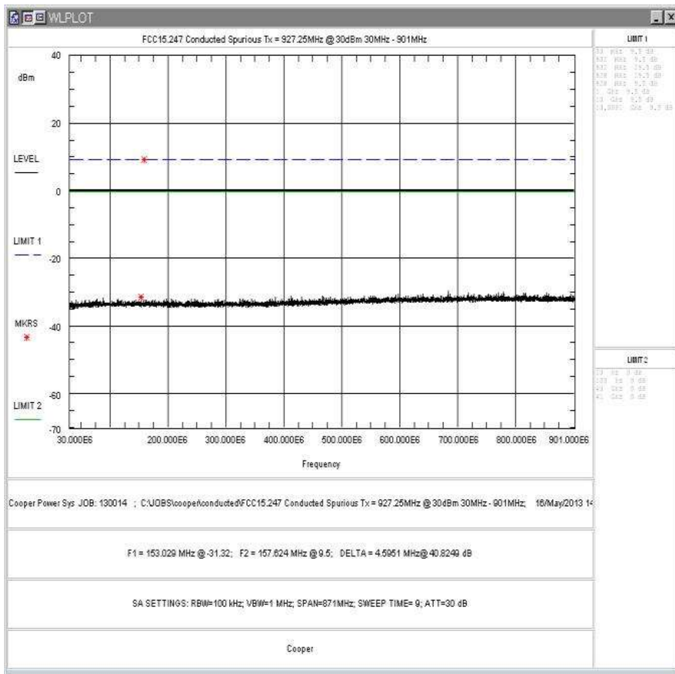
Figure 23: Conducted Spurious Emissions, High Power, High Channel 30 - 901MHz
