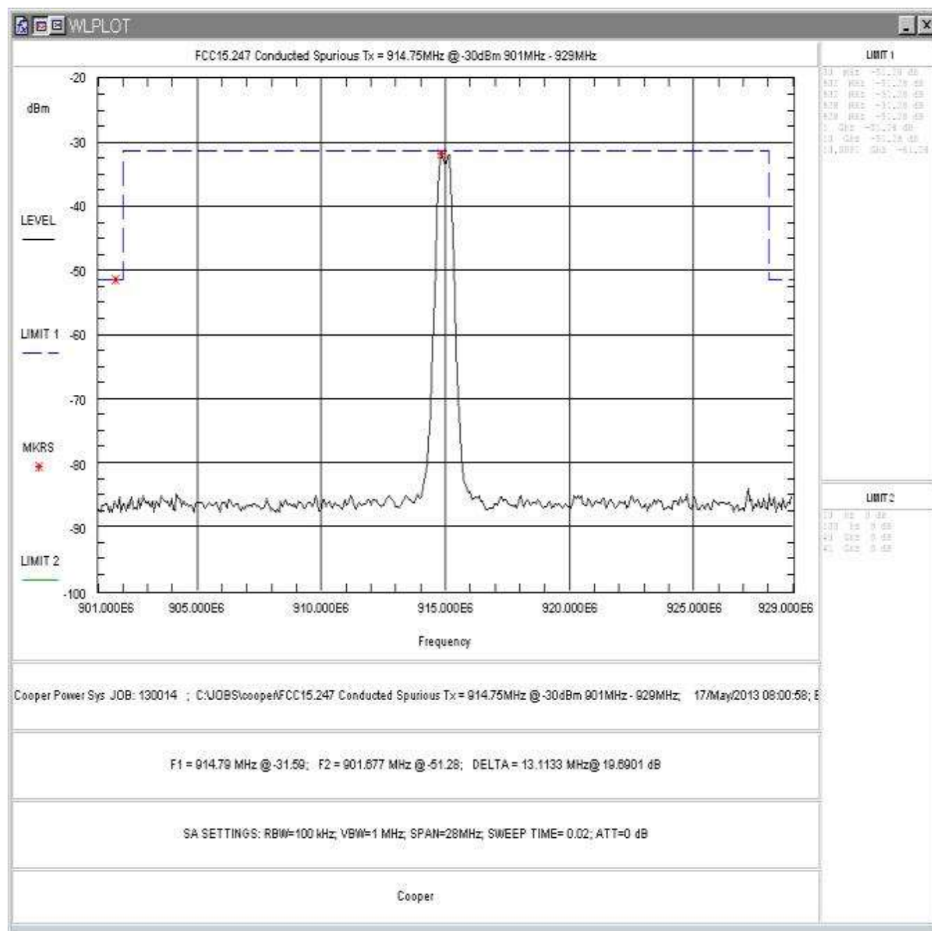
Figure 32: Conducted Spurious Emissions, Low Power, Center Channel 901 – 929MHz
