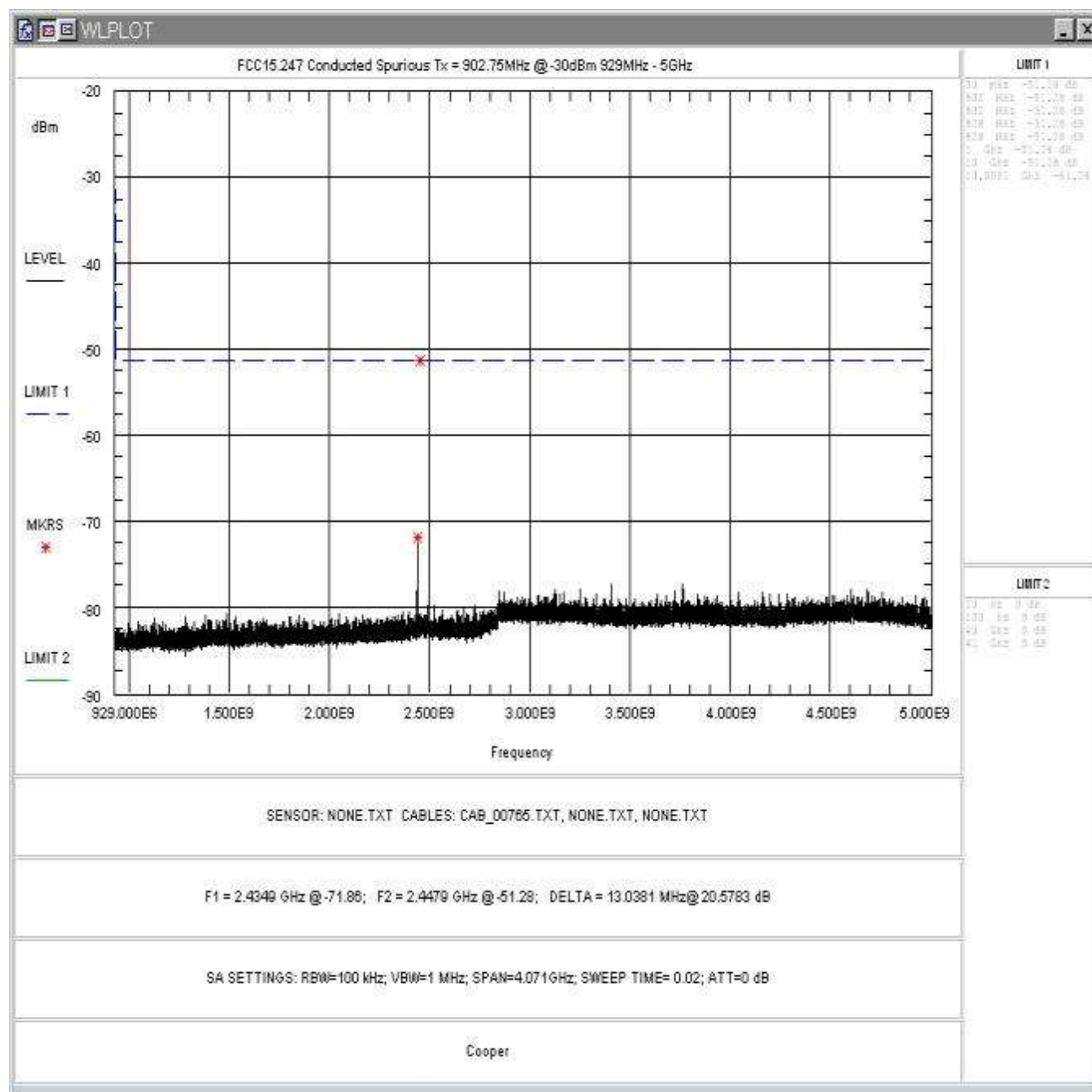
Figure 29: Conducted Spurious Emissions, Low Power, Low Channel 929-5000MHz
