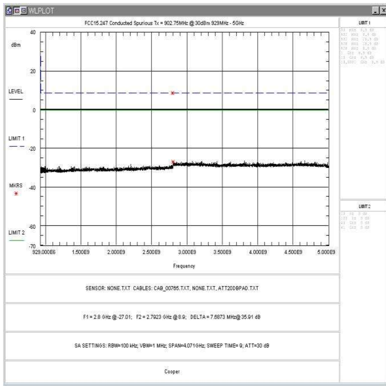
Figure 17: Conducted Spurious Emissions, High Power, Low Channel 929-5000MHz
