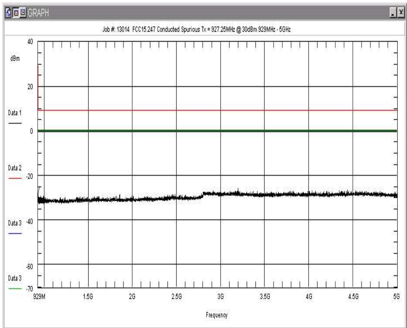
Figure 25: Conducted Spurious Emissions, High Power, High Channel 929-5000MHz
