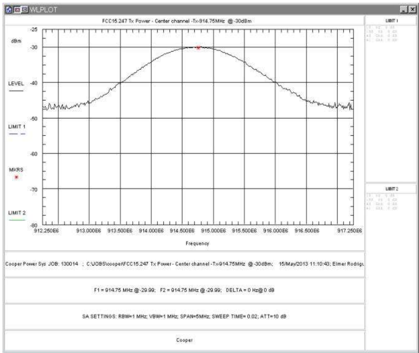
Figure 8: RF Peak Power, Low Power, Center Channel
