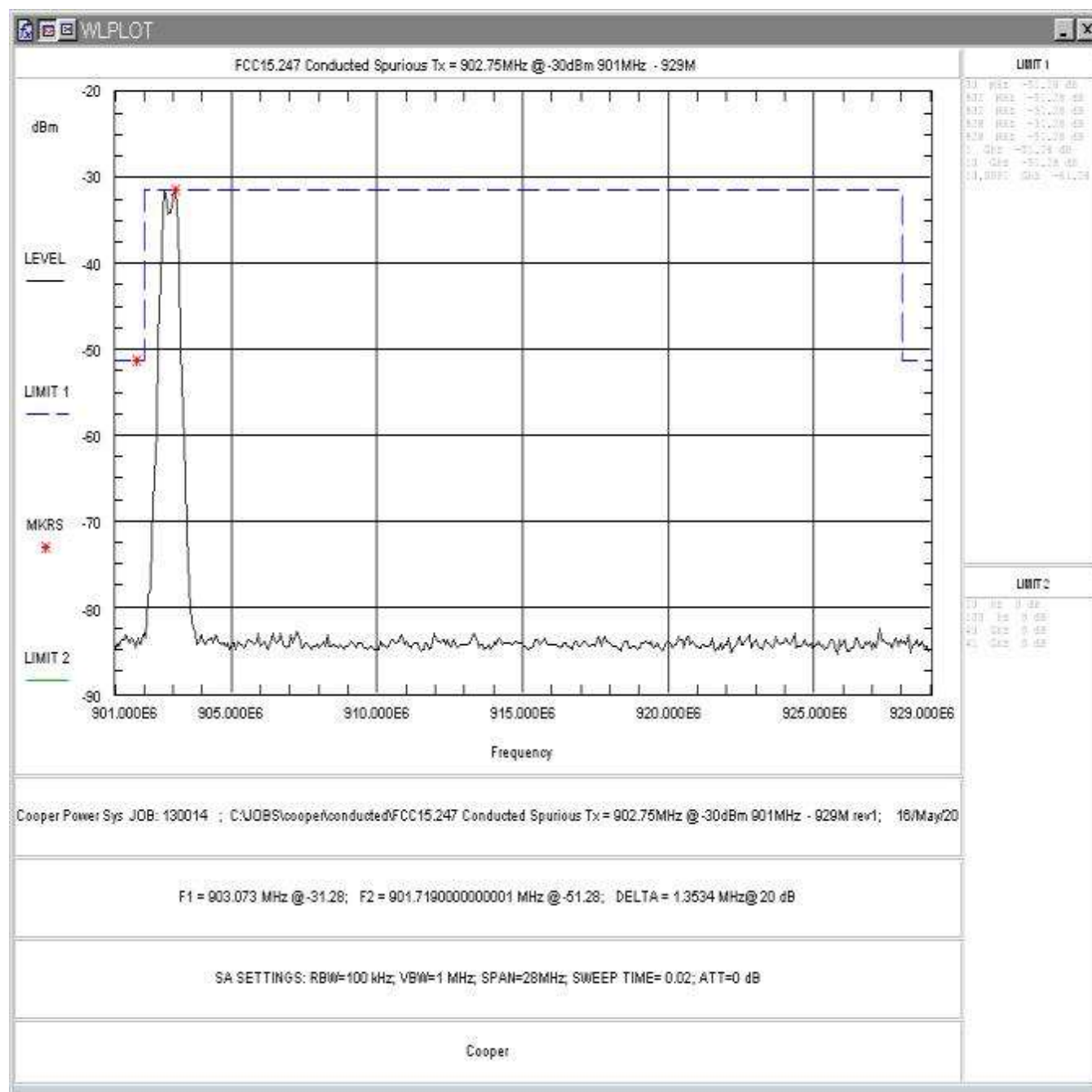
Figure 28: Conducted Spurious Emissions, Low Power, Low Channel 901 – 929MHz
