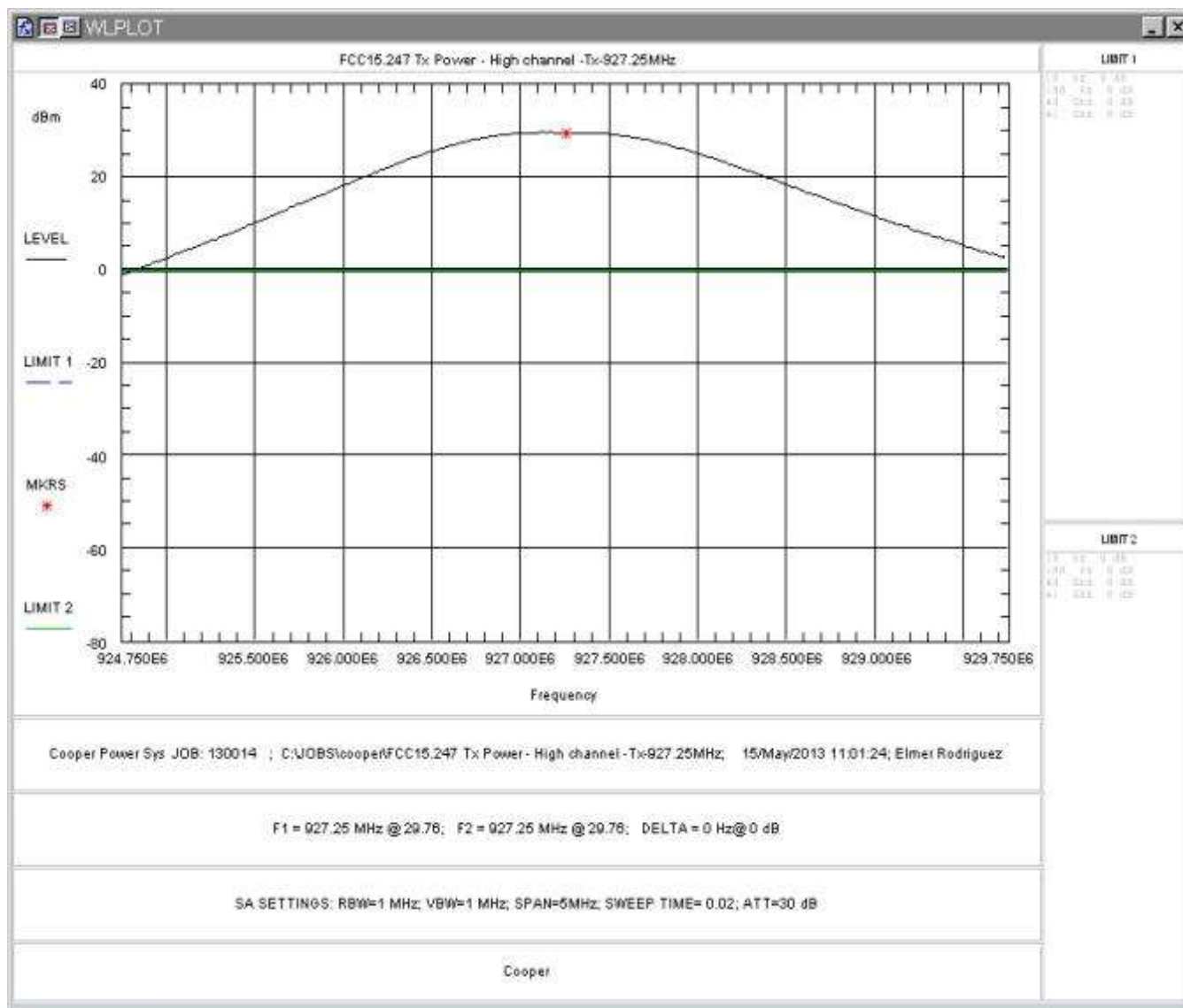
Figure 6: RF Peak Power, High Power, High Channel
