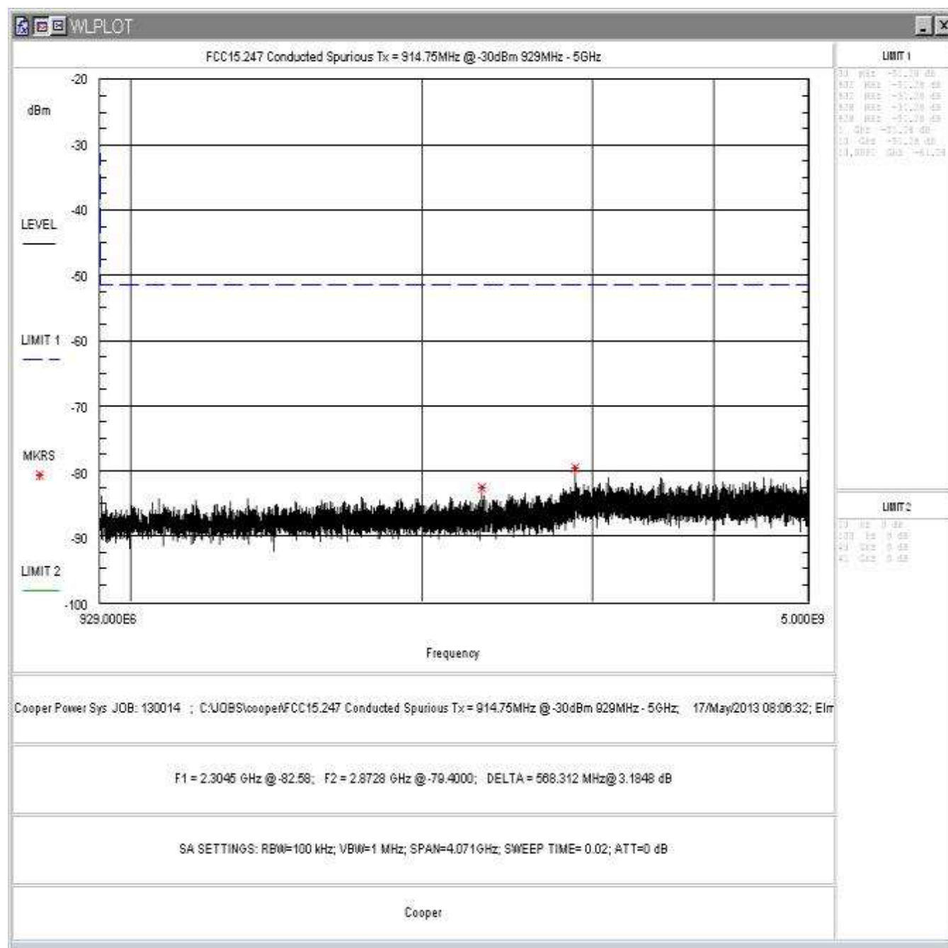
Figure 33: Conducted Spurious Emissions, Low Power, Center Channel 929-5000MHz
