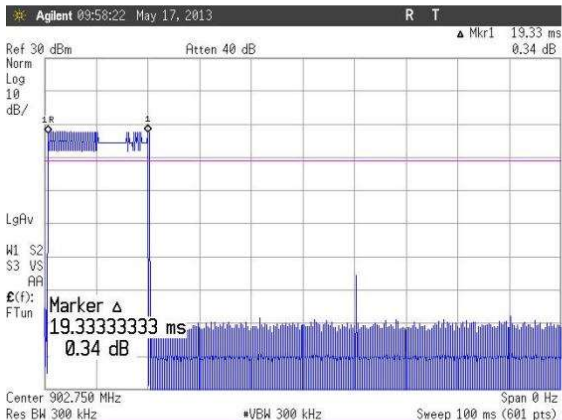
Figure 2: Dwell time per 100ms (Duty Cycle)
