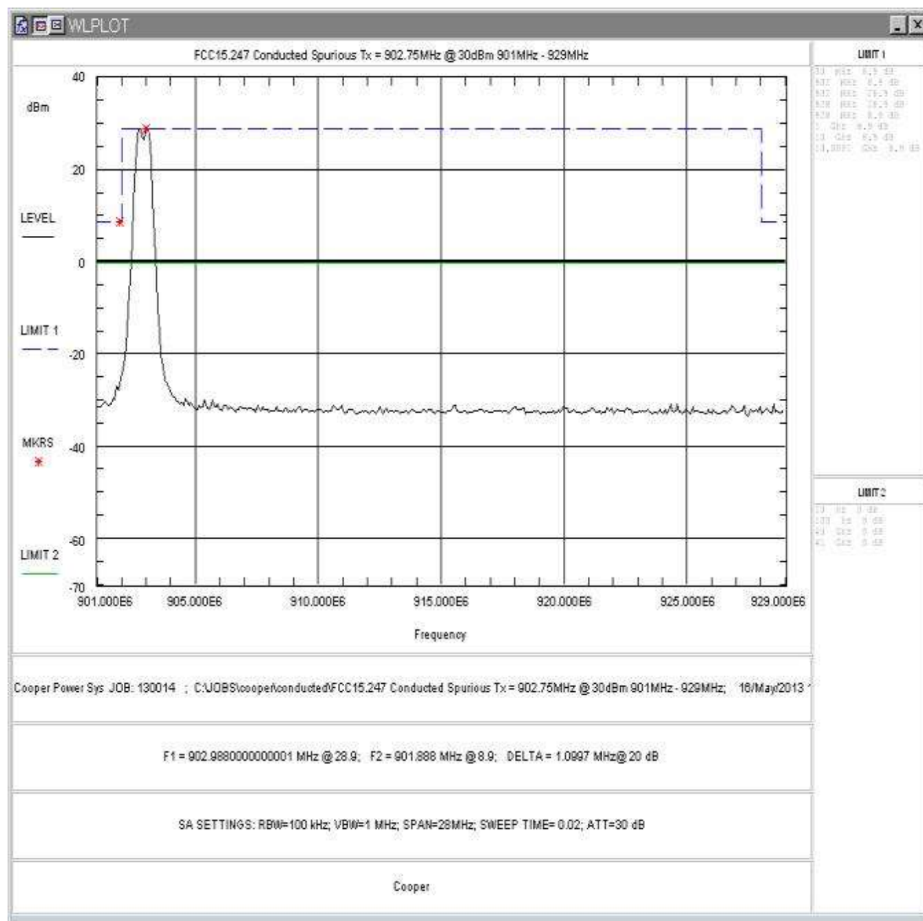
Figure 16: Conducted Spurious Emissions, High Power, Low Channel 901 – 929MHz
