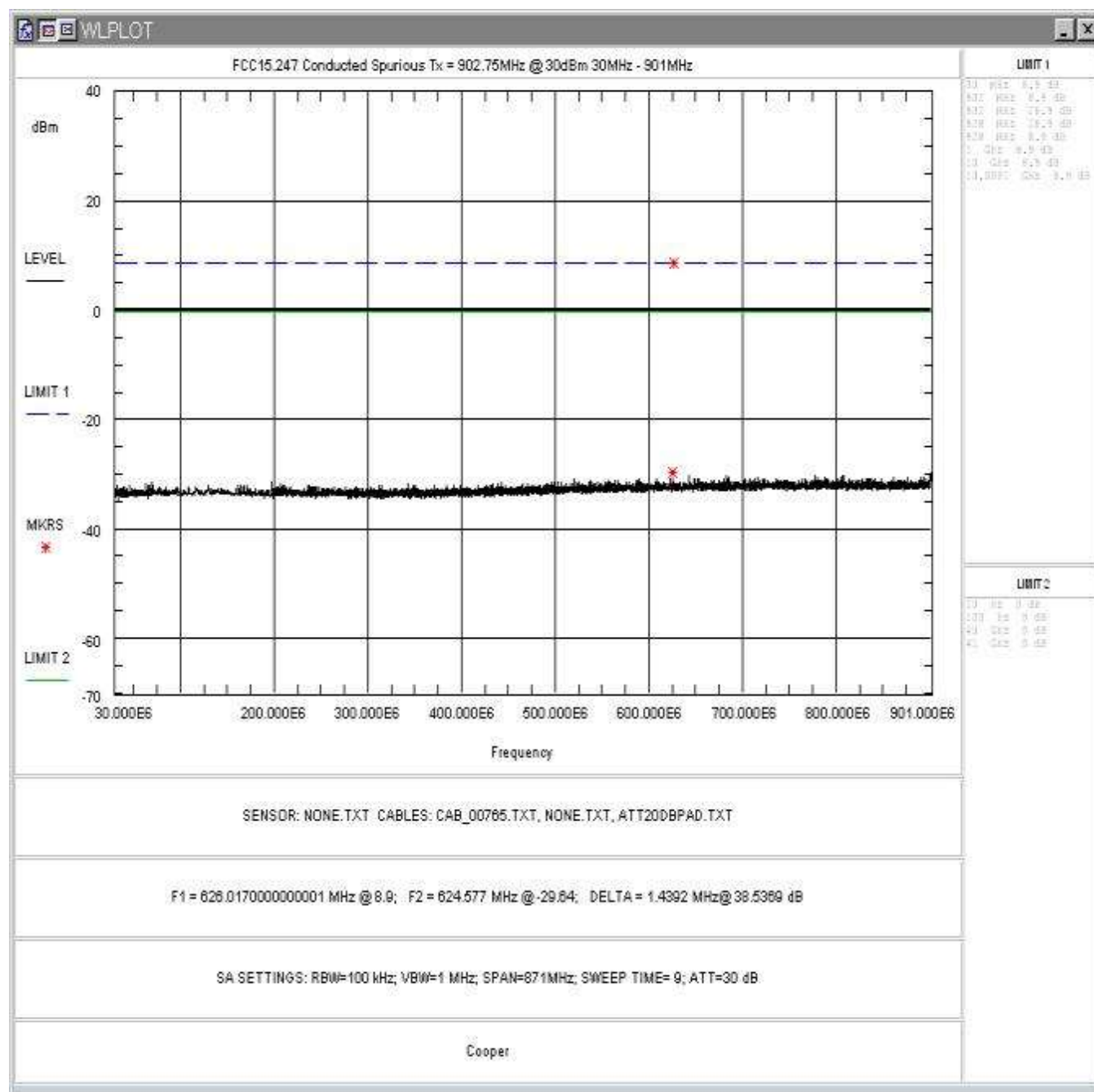
Figure 15: Conducted Spurious Emissions, High Power, Low Channel 30 - 901MHz
