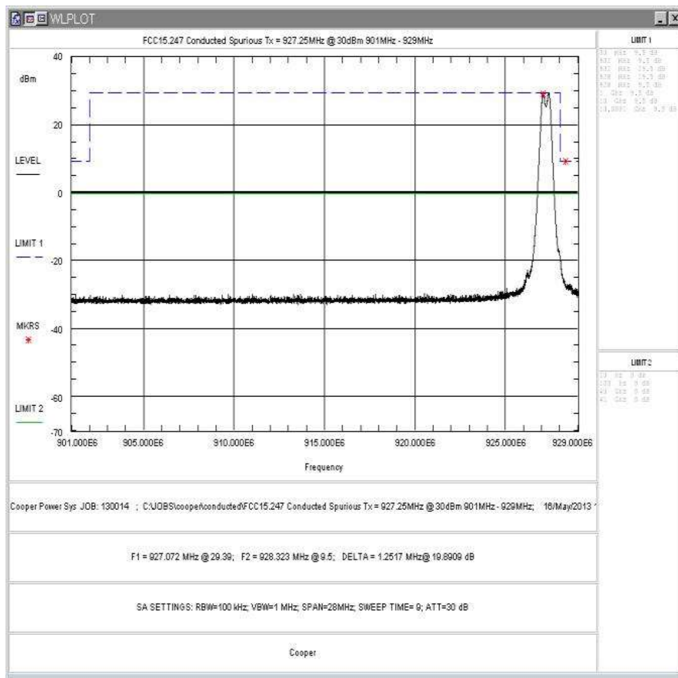
Figure 24: Conducted Spurious Emissions, High Power, High Channel 901 – 929MHz
