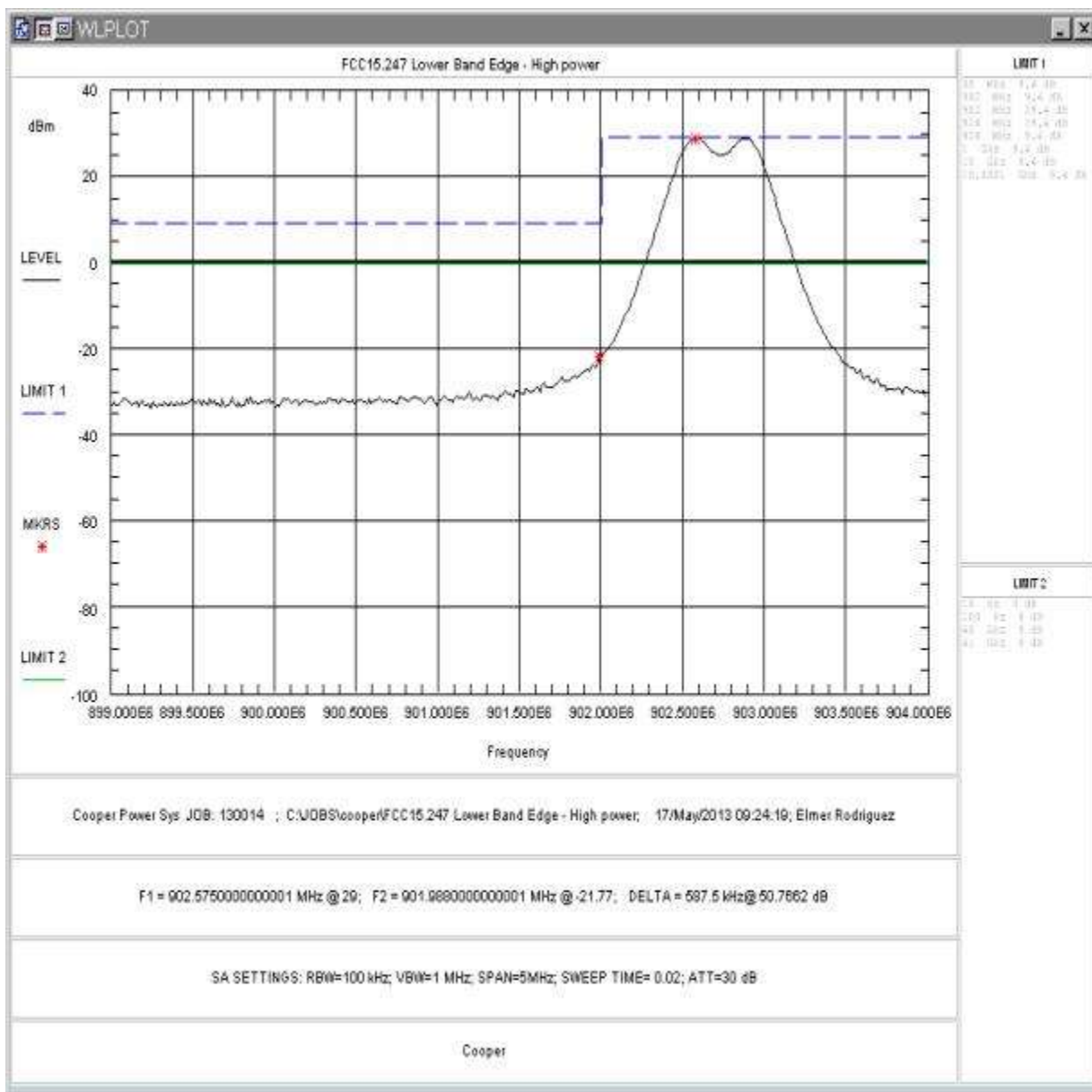
Figure 39: Lower Band-edge, Low Channel, High Power
