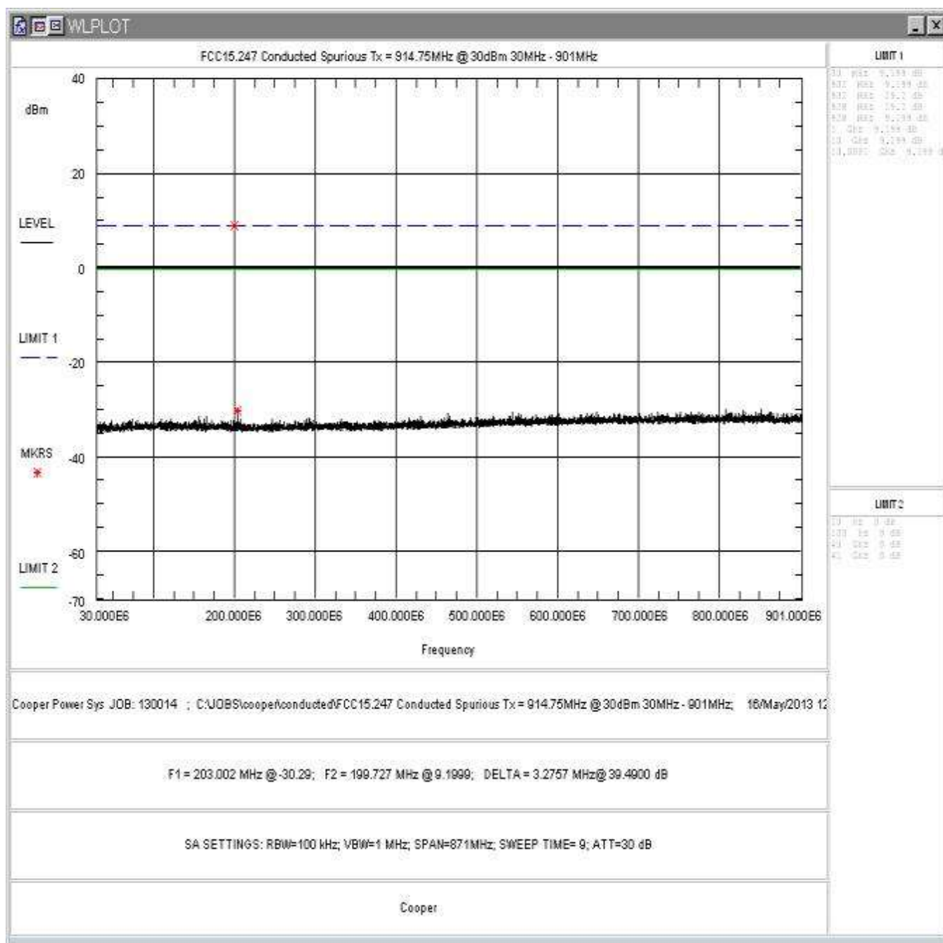
Figure 19: Conducted Spurious Emissions, High Power, Center Channel 30 - 901MHz
