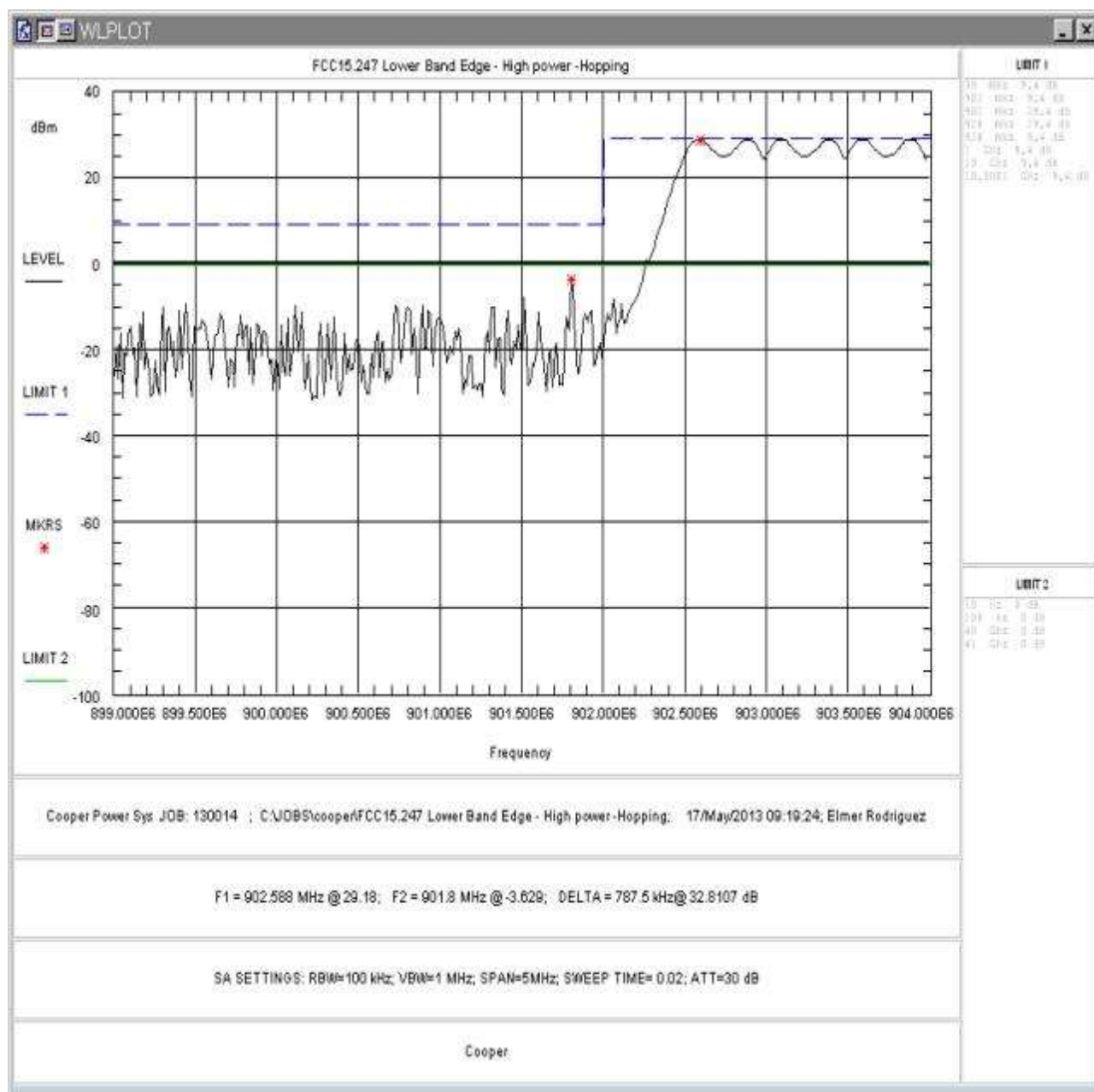
Figure 40: Lower Band-edge, Hopping Mode, High Power
