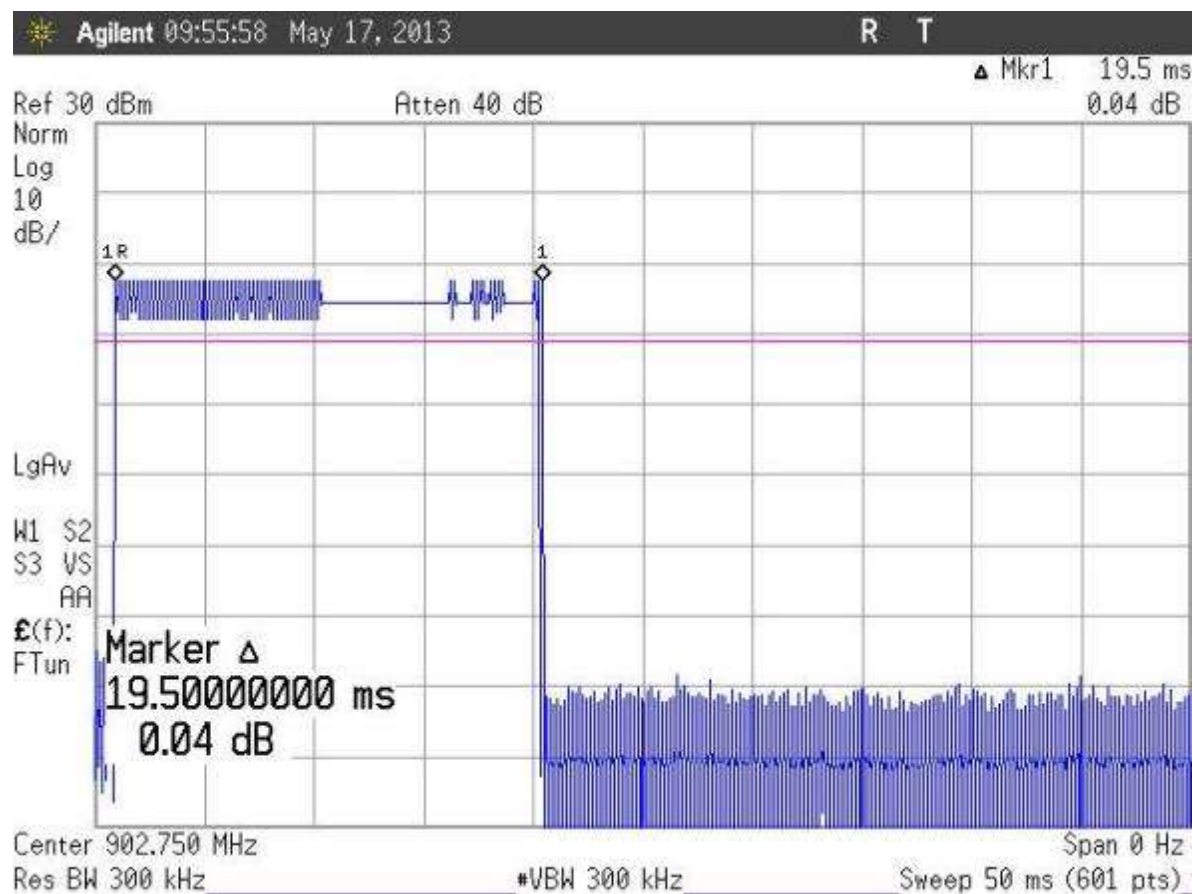
Figure 1: Single Hop Plot
