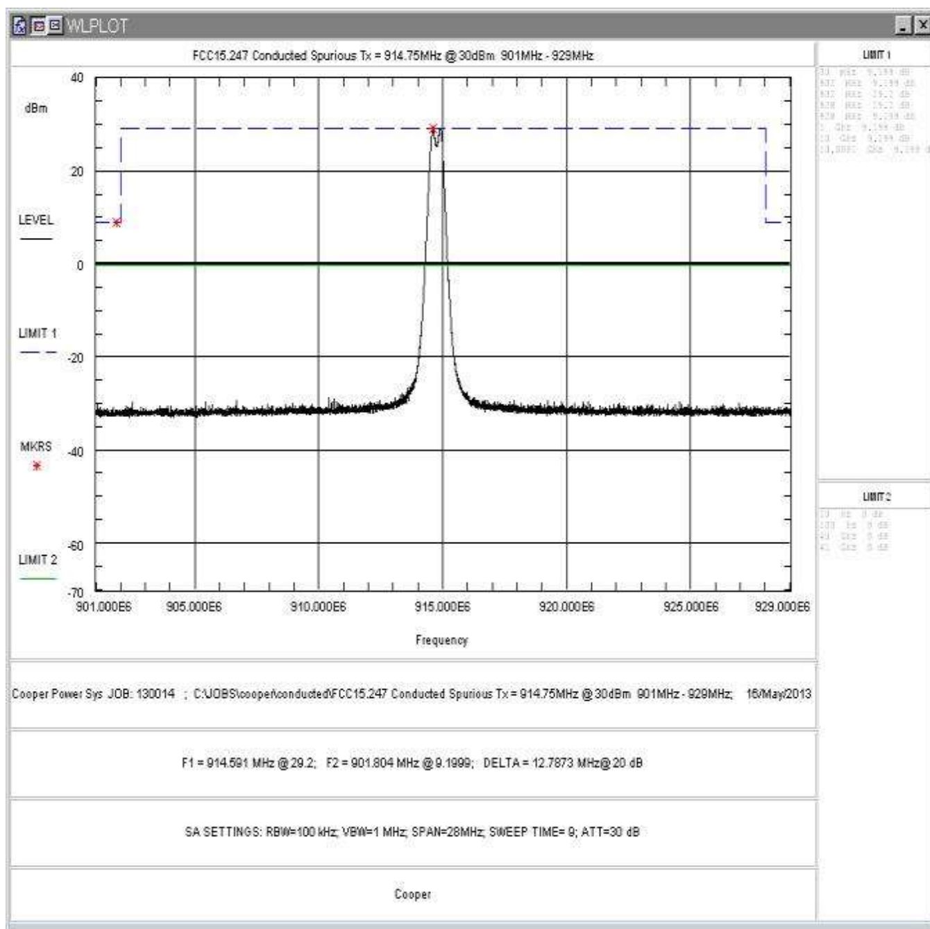
Figure 20: Conducted Spurious Emissions, High Power, Center Channel 901 – 929MHz
