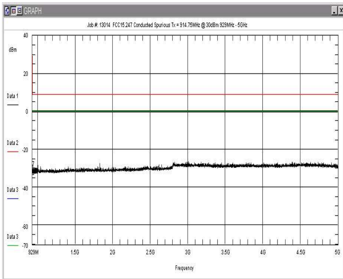
Figure 21: Conducted Spurious Emissions, High Power, Center Channel 929-5000MHz
