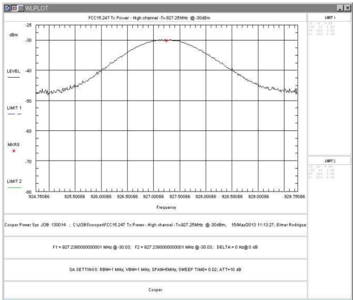
Figure 9: RF Peak Power, Low Power, High Channel
