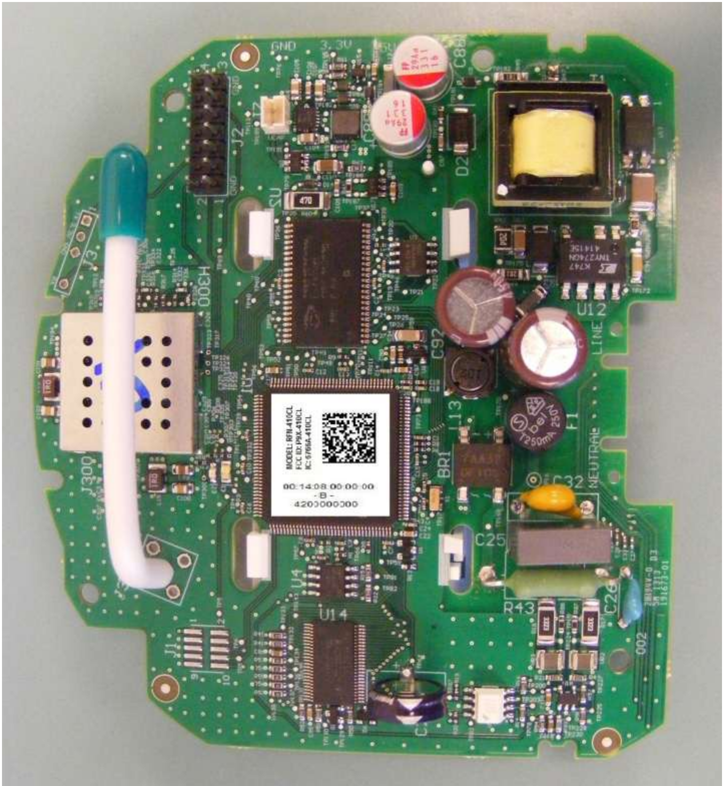
Figure 1: RFN-410CL - Top
