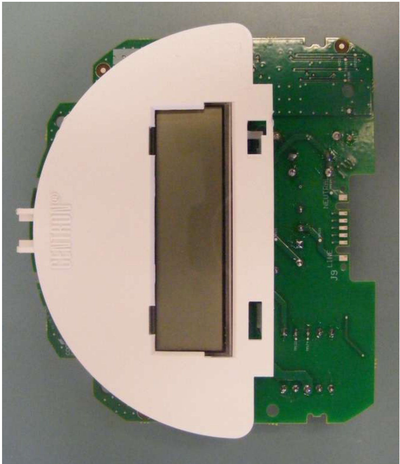
Figure 2: RFN-410CL – Bottom
