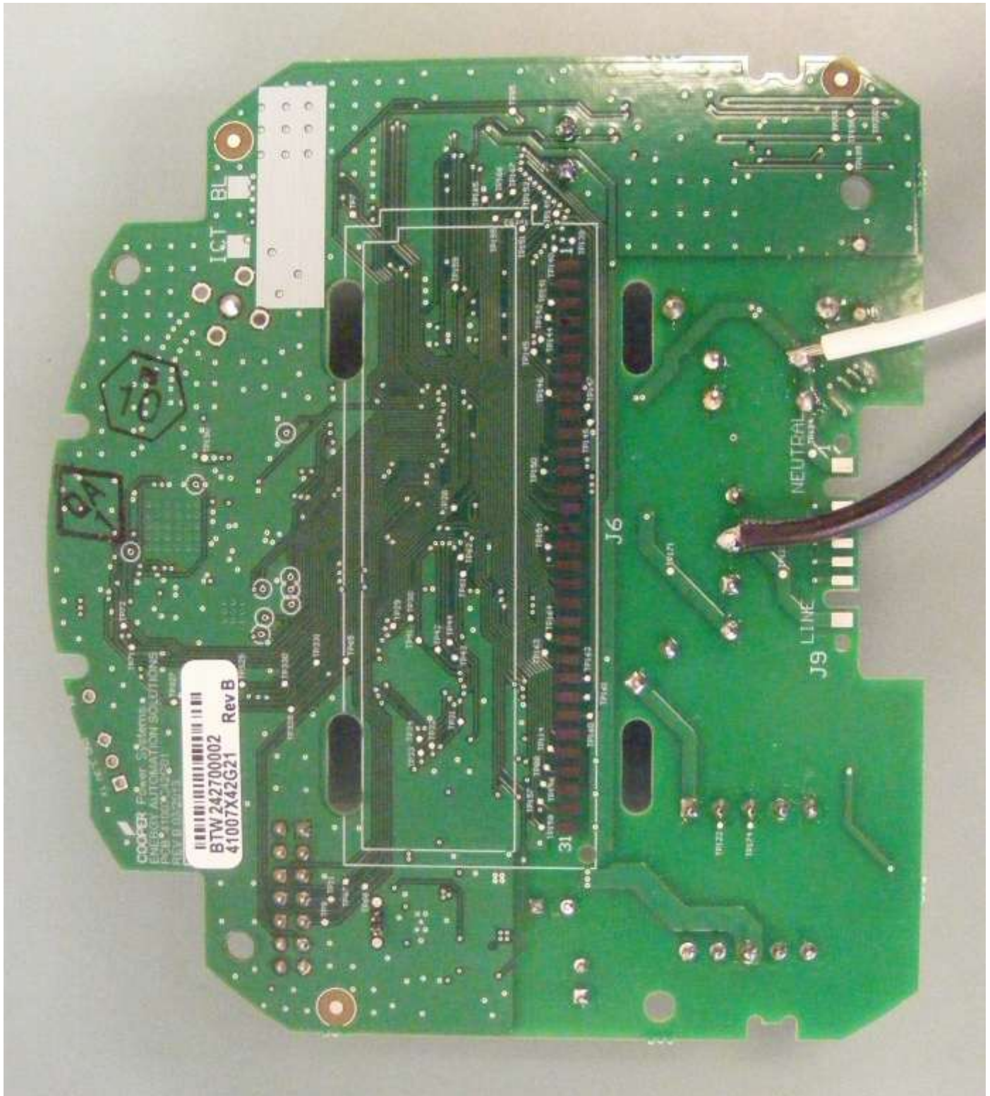
Figure 4: RFN-410CL – Bottom, meter display board removed
