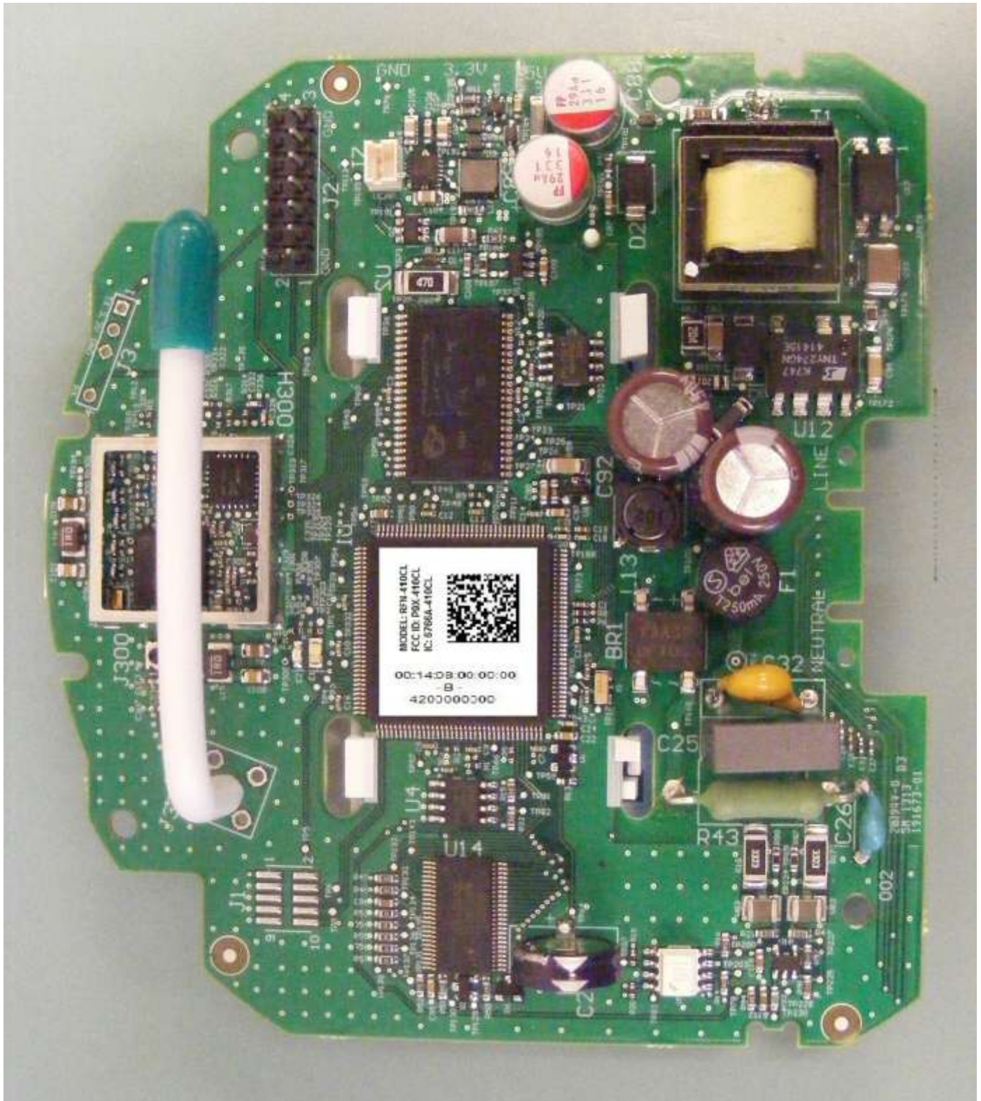
Figure 3: RFN-410CL – Top, shield removed
