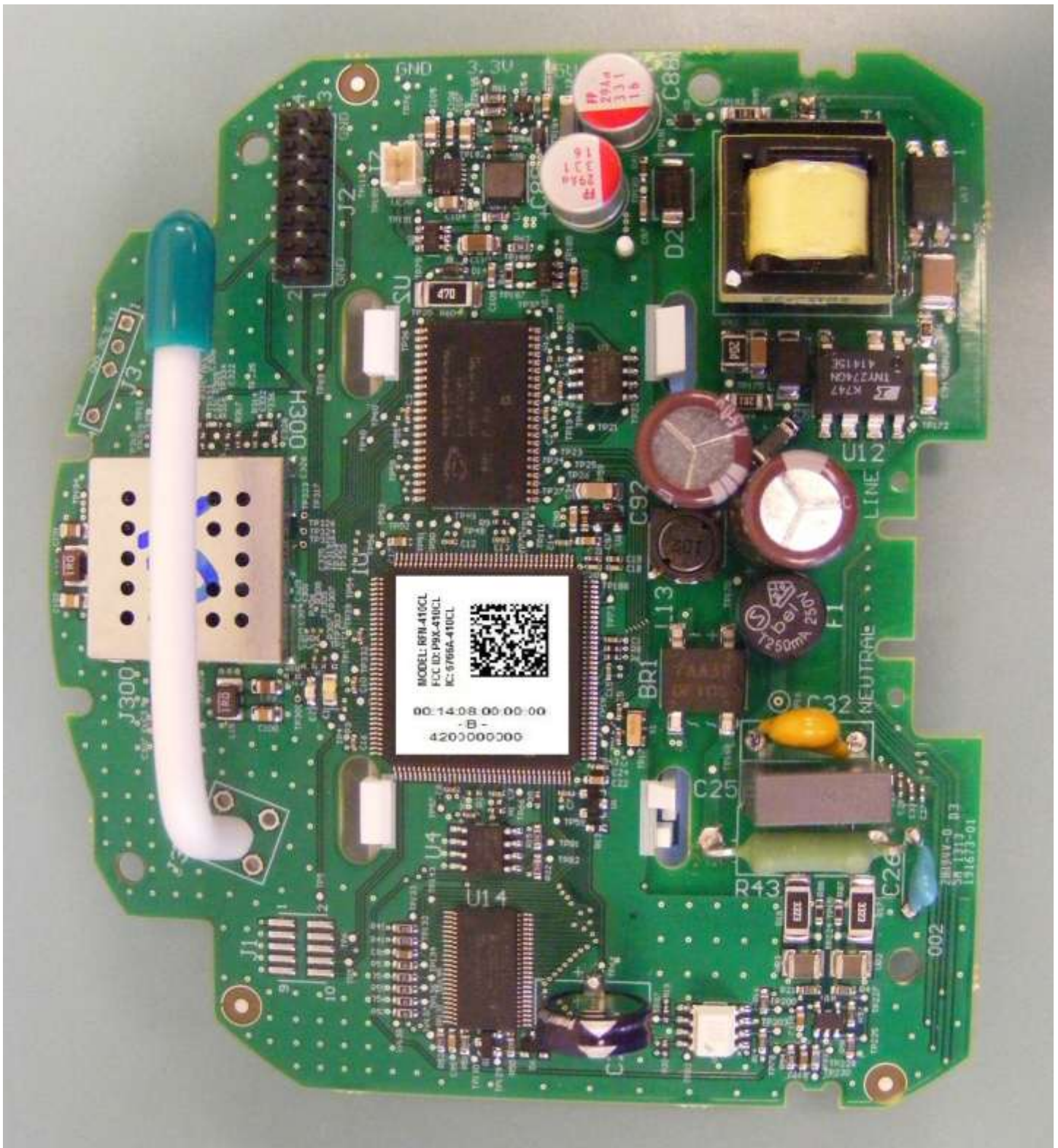
Figure 1: RFN-410CL - Top
