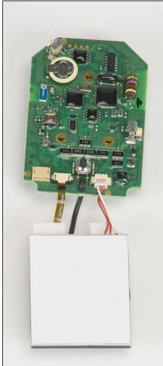
Display connections
