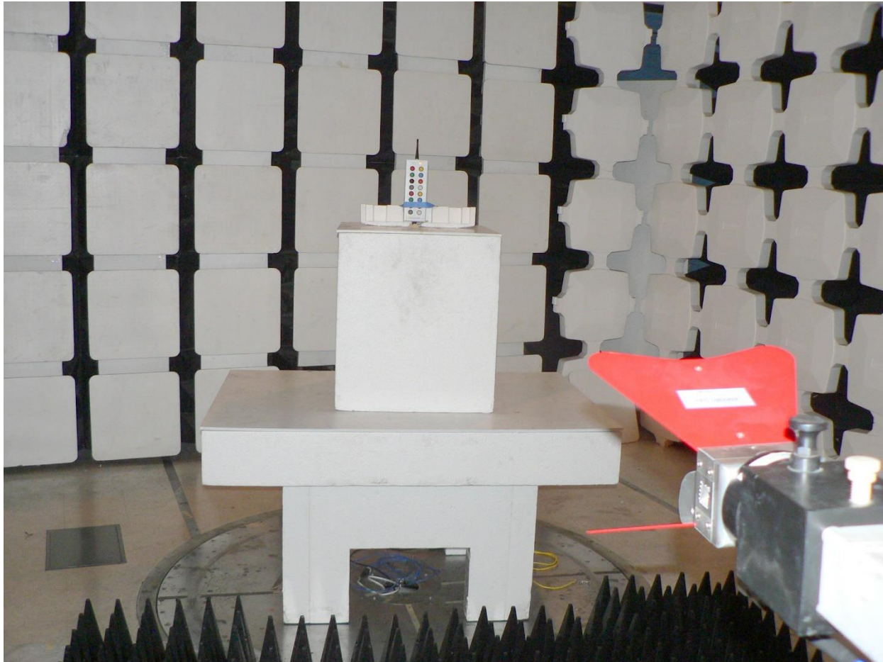
TCFS03 TX Spurious 1-10GHz
