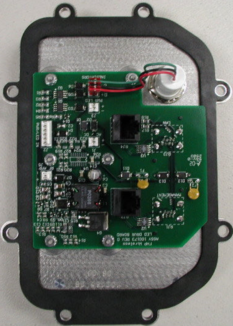
Power Supply Board Component Side
