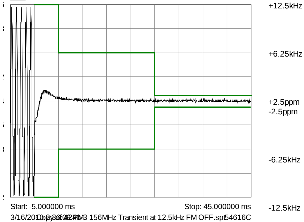
4240-3 156MHz Transient at 12.5kHz FM OFF
