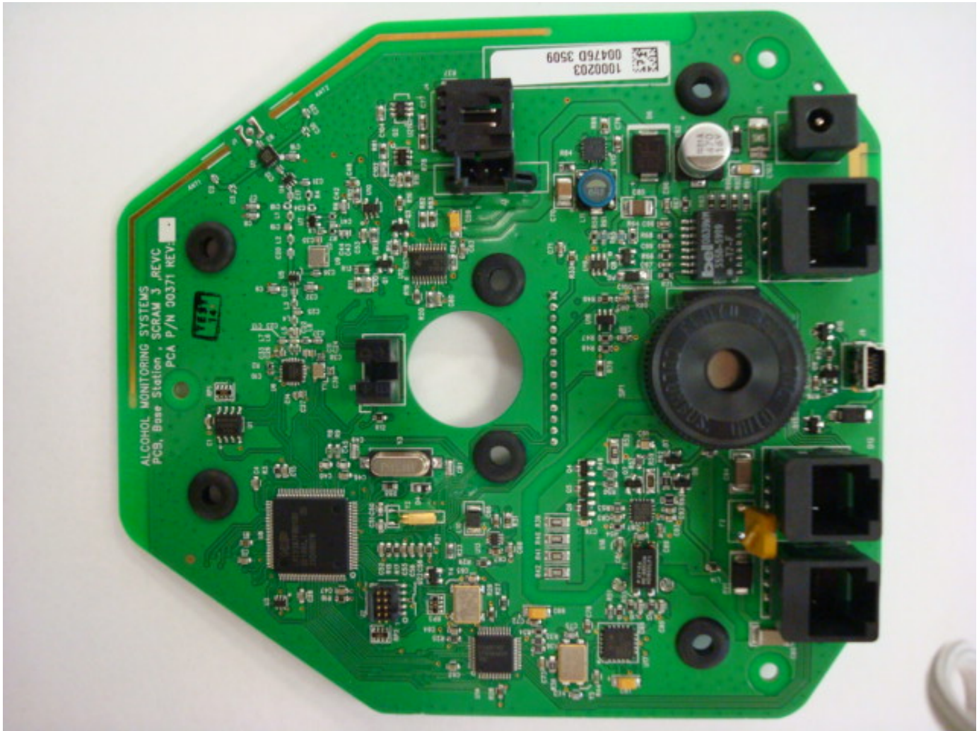
SM03 Internal Photo: PCB Top
