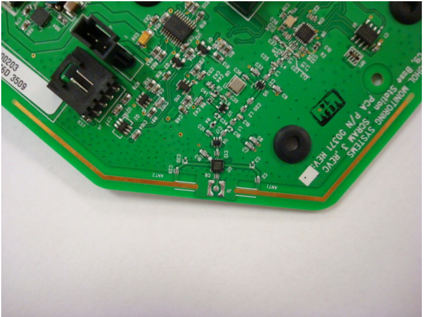
SM03 Internal Photo: RF Antenna
