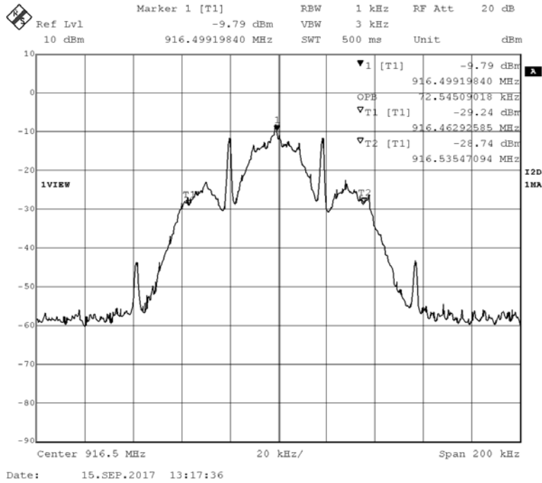
99% Power Bandwidth
