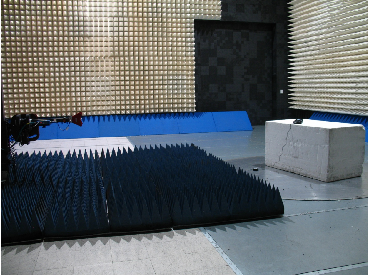
Radiated emissions > 1GHz (unintentional transmission)
