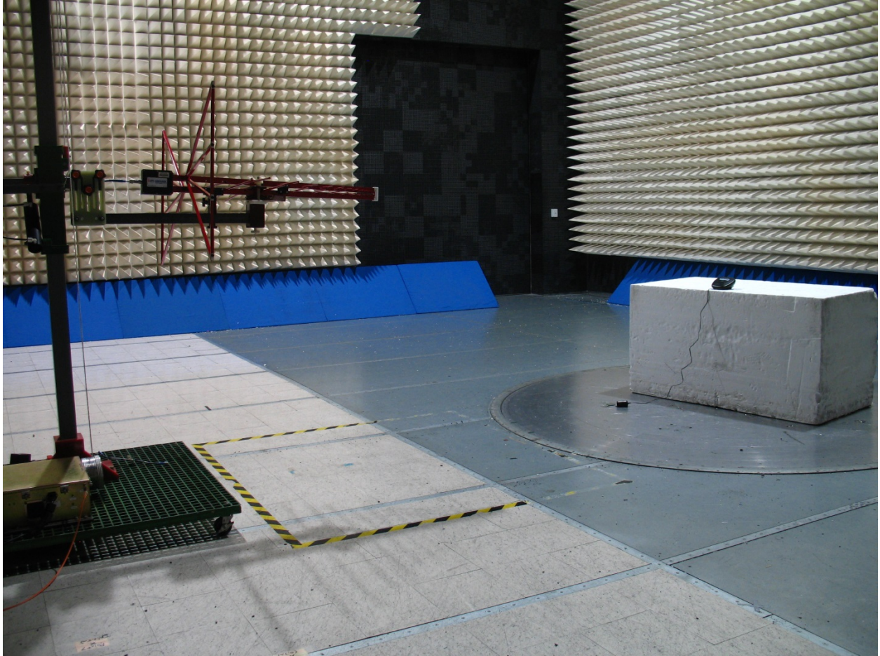
Radiated Emissions 30MHz-1GHz (intentional transmission)
