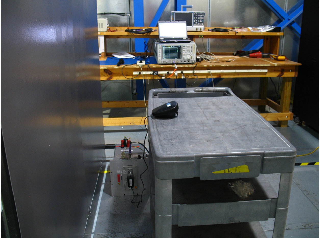
Conducted voltage emissions
