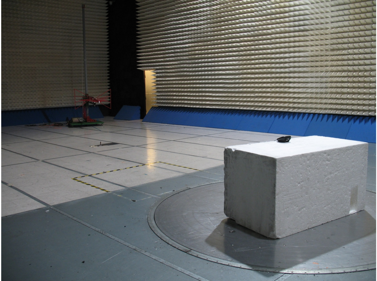
Radiated emissions 30MHz-1GHz (unintentional transmission)
