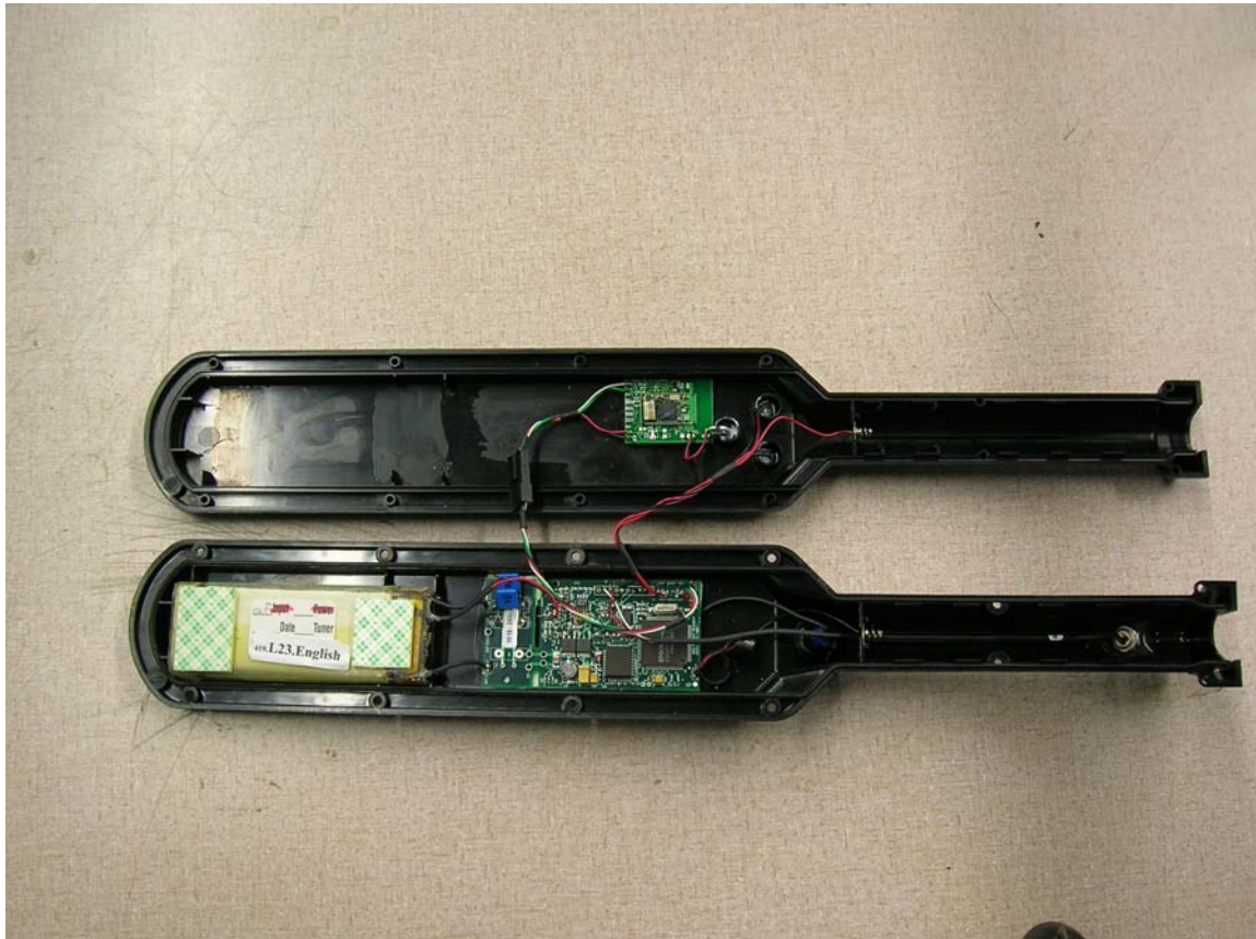
Inside of Handle
