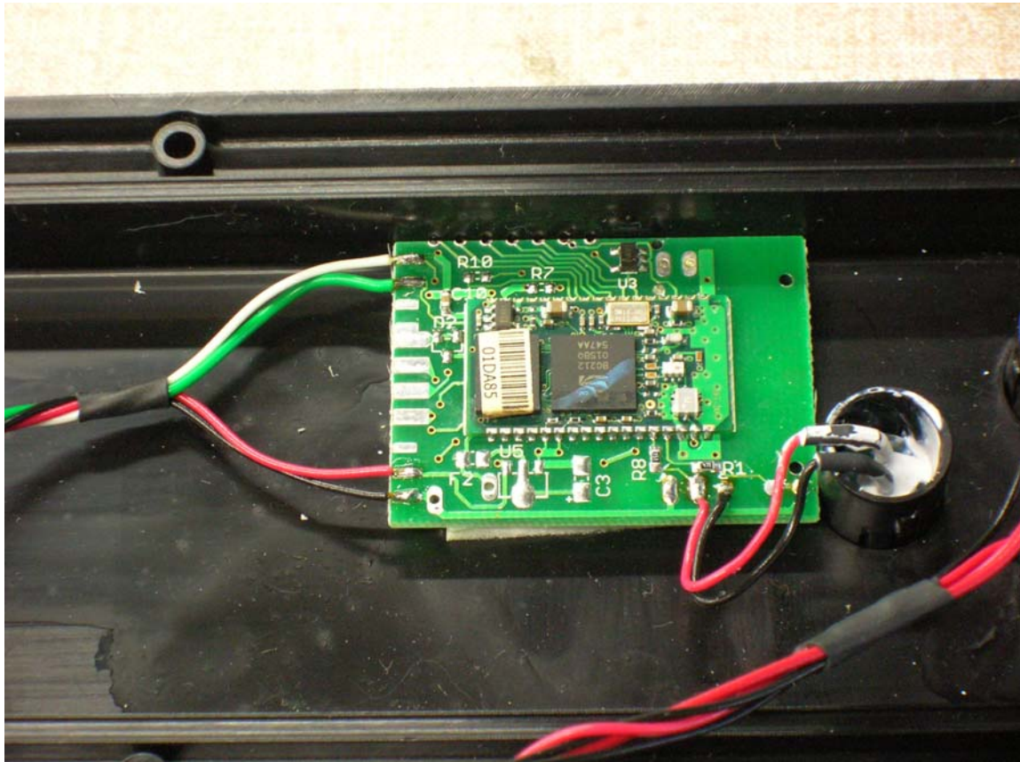
Bluetooth Board Connections
