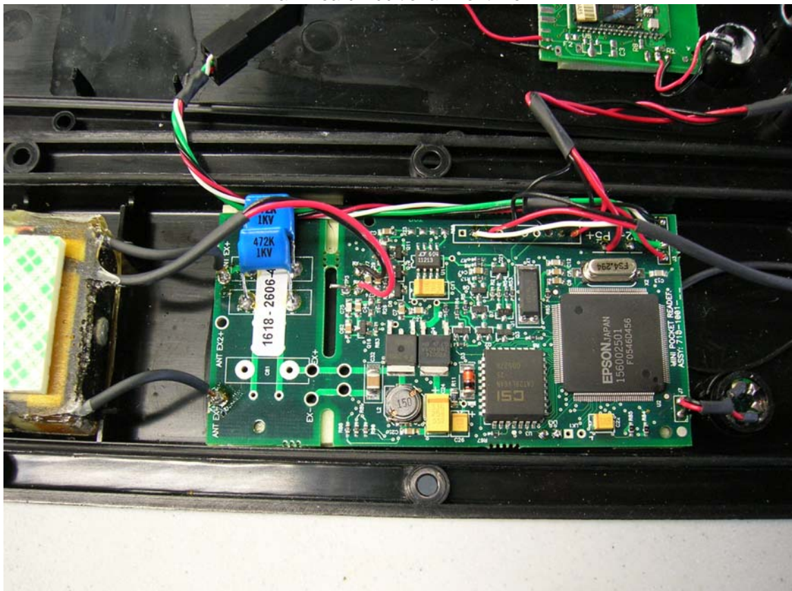
Main Board Additional Front View
