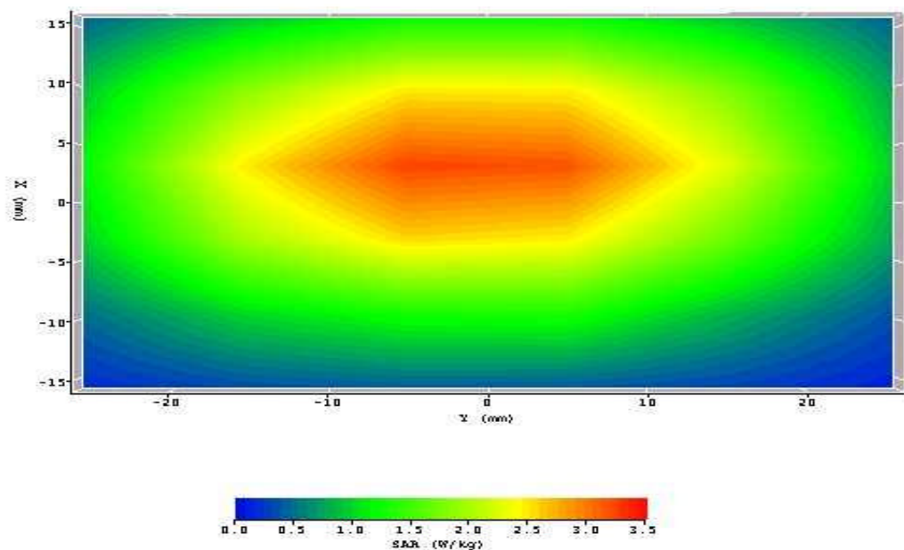
Figure 14. Validation Measurement - 1800 MHz in Body Tissue
