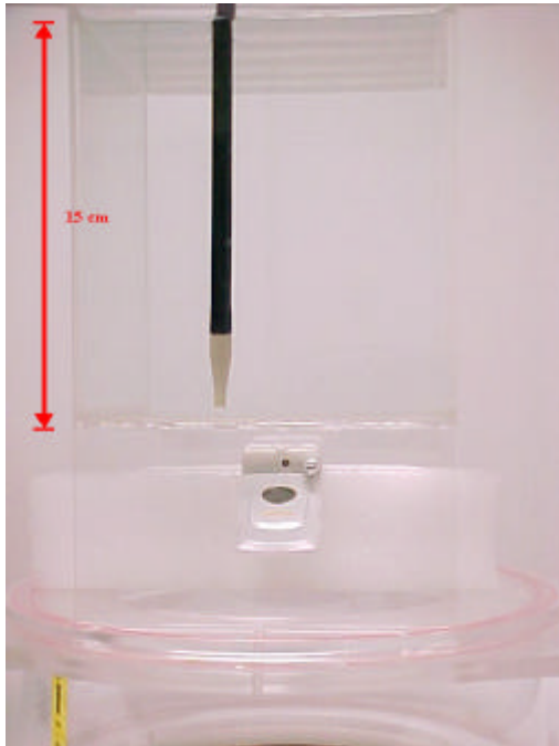
Fig S11. Battery (700 mAH) facing the phantom without Headset.
