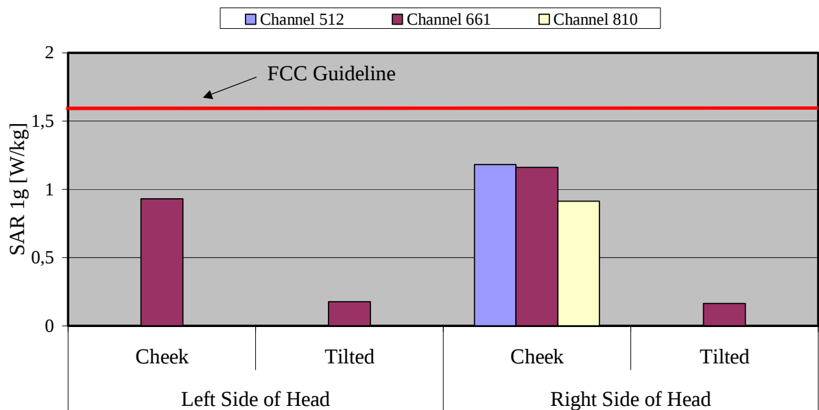
Fig. 7: The measured head phantom SAR values for the Mobicom C6088i with slim battery for PCS 1900 in comparison to the FCC exposure limit.
