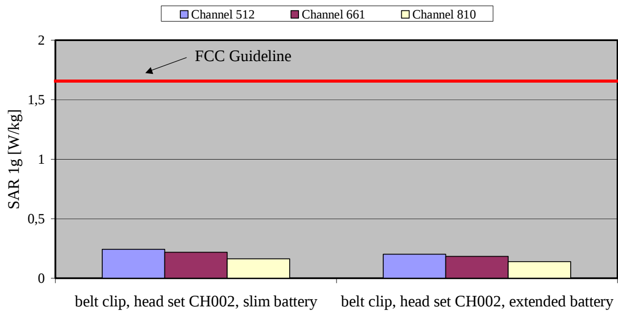
Fig. 9: The measured SAR values in body-worn configuration for the Mobicom C6088i with belt clip, headset CH002 and different batteries for PCS 1900 in comparison to the FCC exposure limit.
