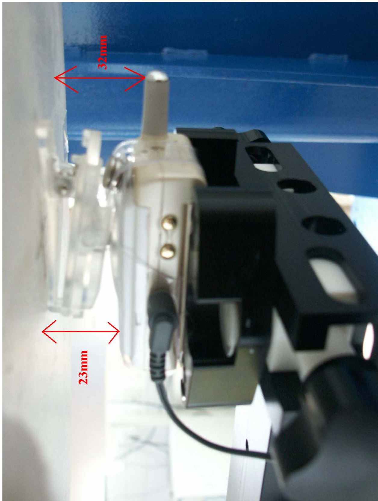
Fig. 21: Body worn configuration, belt clip, headset CH002 and extended battery
