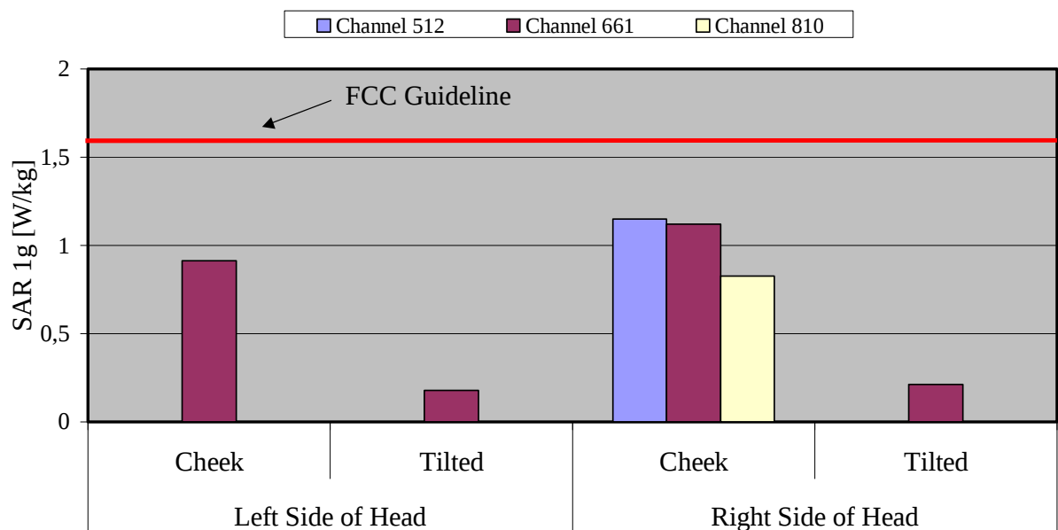
Fig. 8: The measured head phantom SAR values for the Mobicom C6088i with extended battery for PCS 1900 in comparison to the FCC exposure limit.
