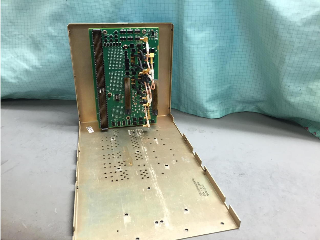
Internal Photos_Receiver CCA
