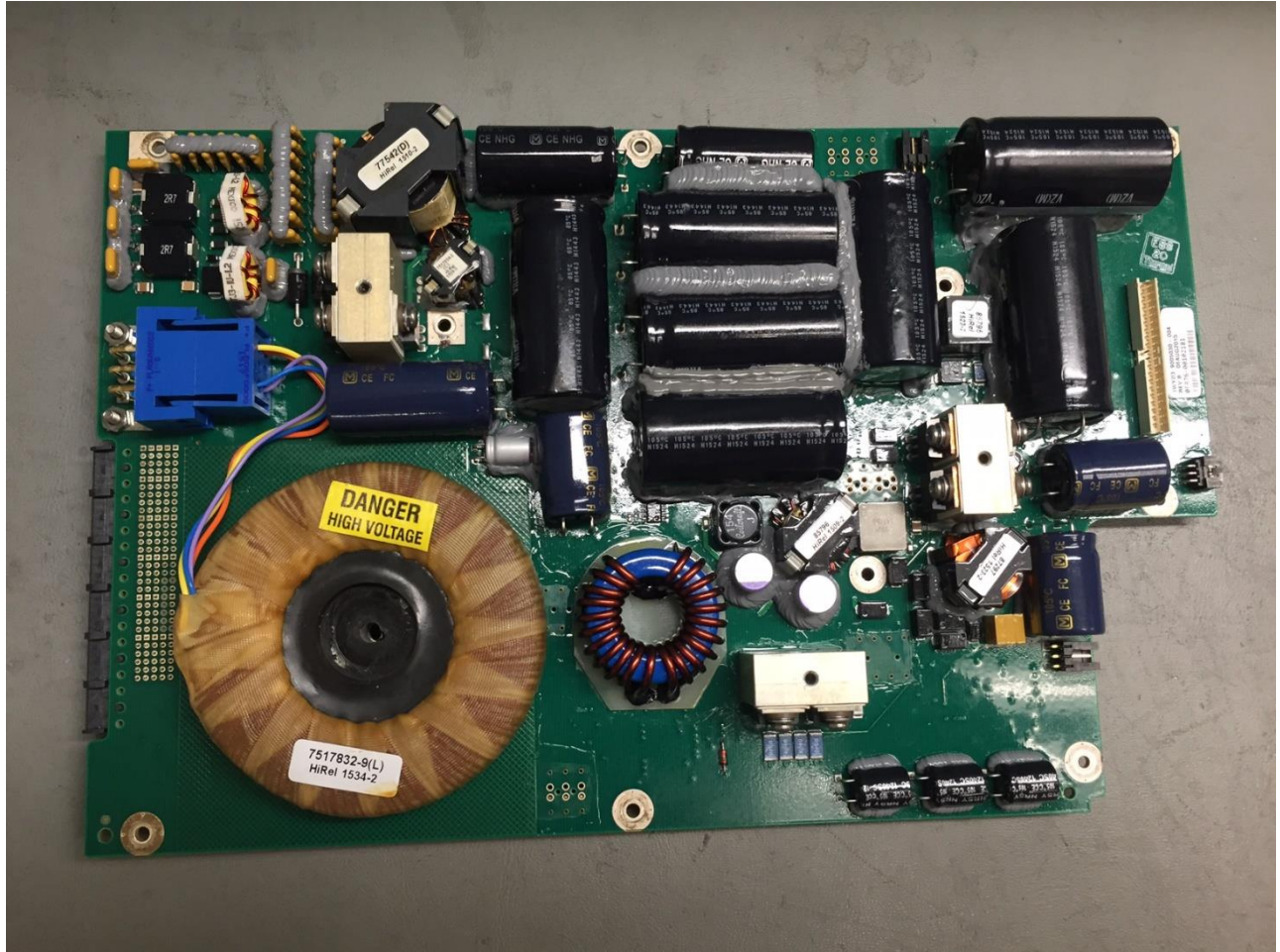
Internal Photos_Power Supply CCA
