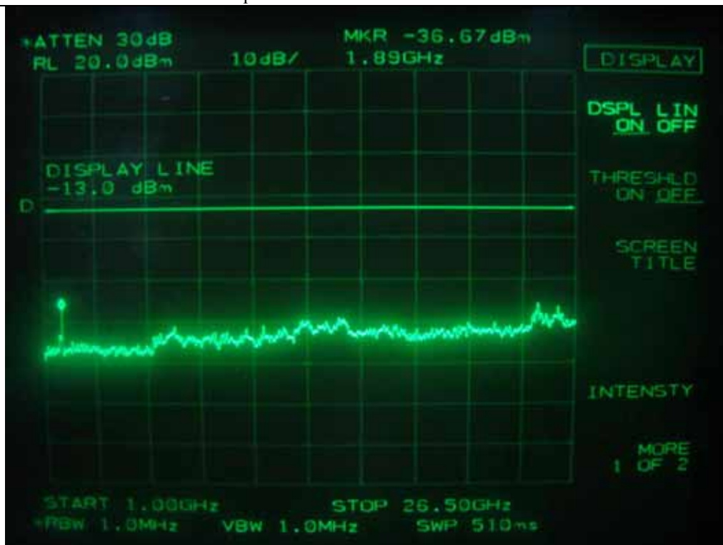
Uplink: CDMA 2000- Low Channel
