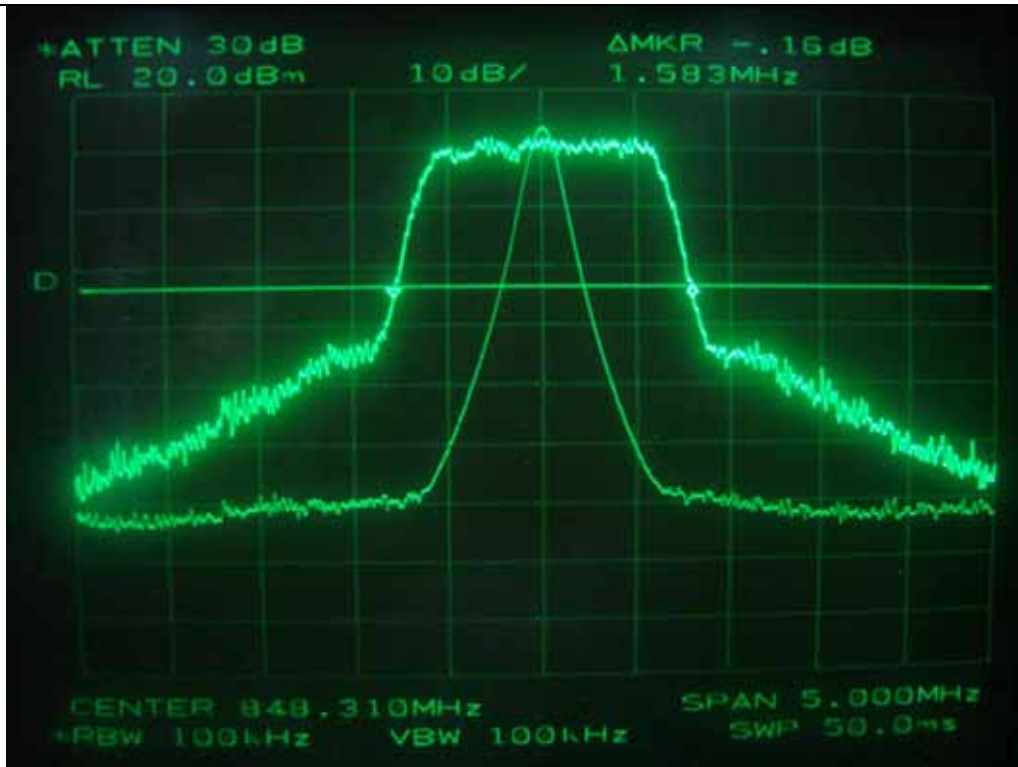
1x EVDO - 26dB Bandwidth
