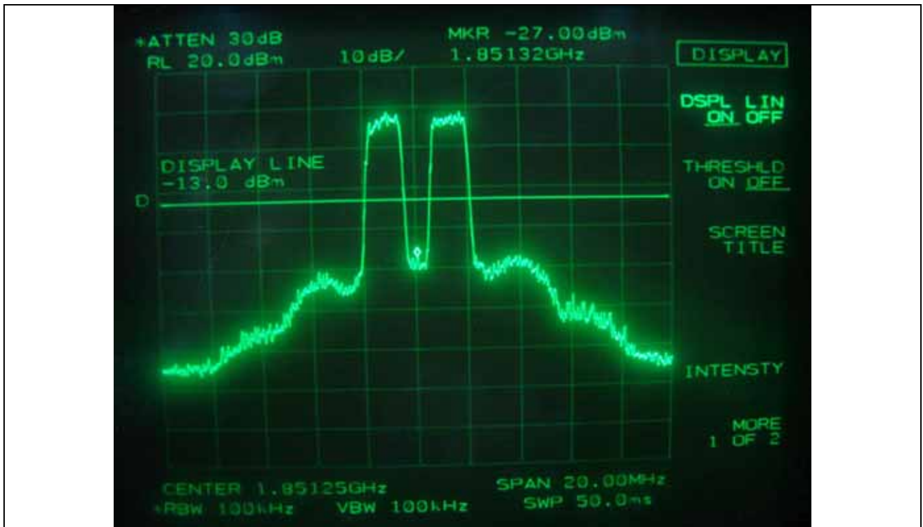
Uplink: CDMA2000 - Low Channel
