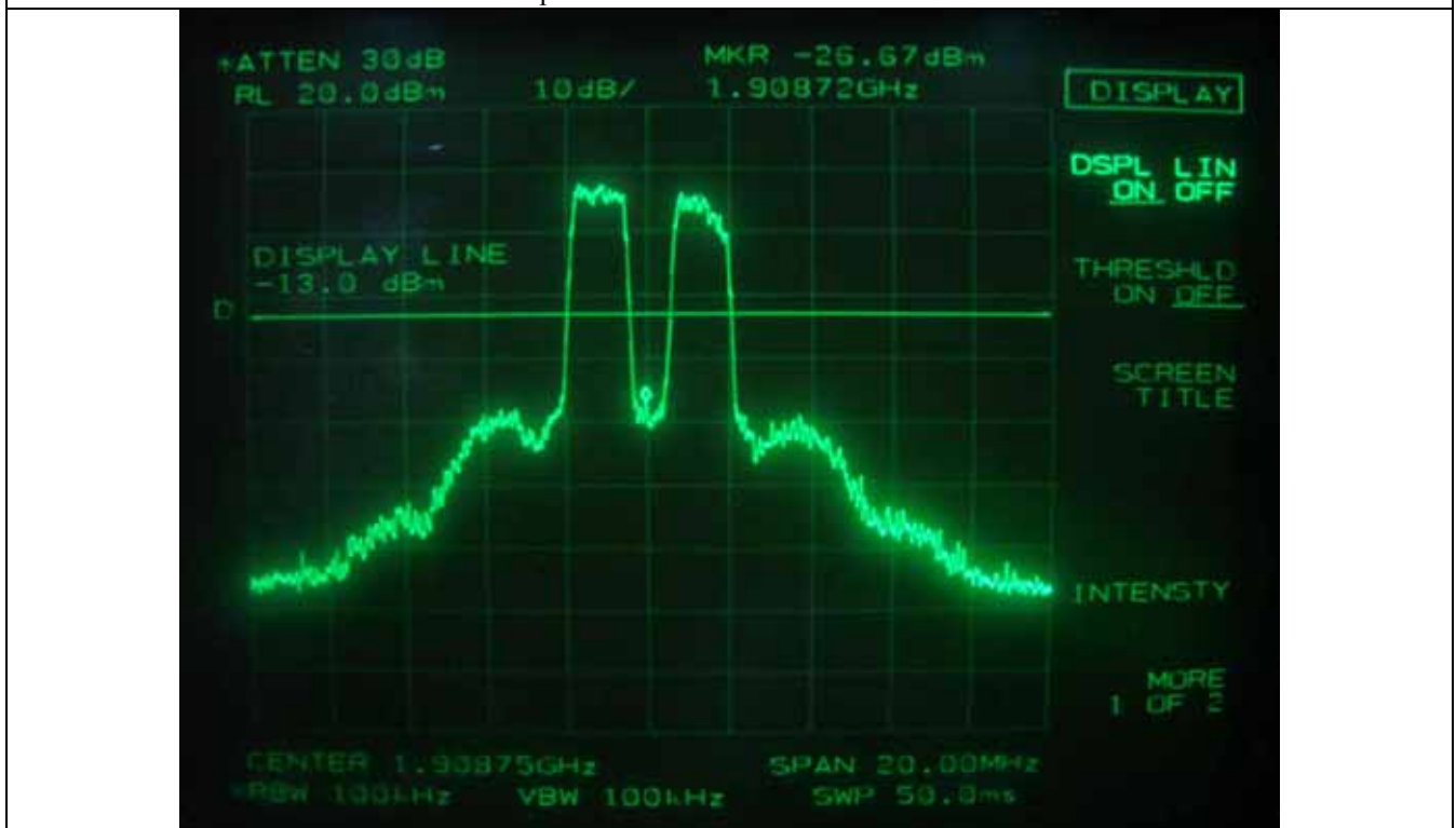
Uplink: CDMA2000 - High Channel
