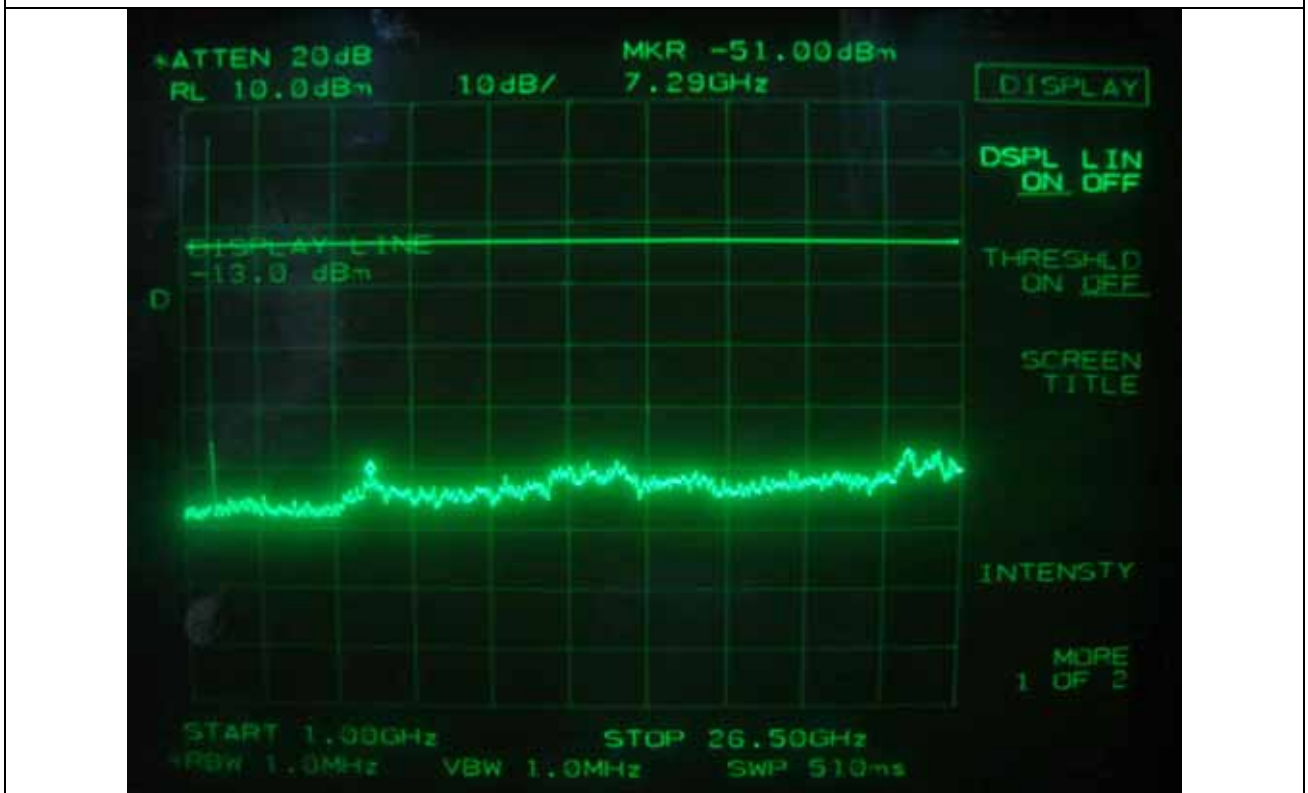
Downlink: CDMA 2000- Low Channel
