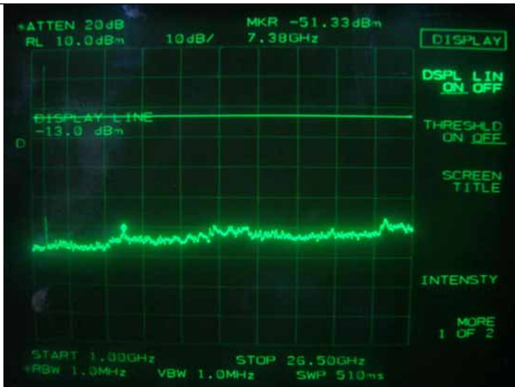
Downlink: IS-95 CDMA - Low Channel
