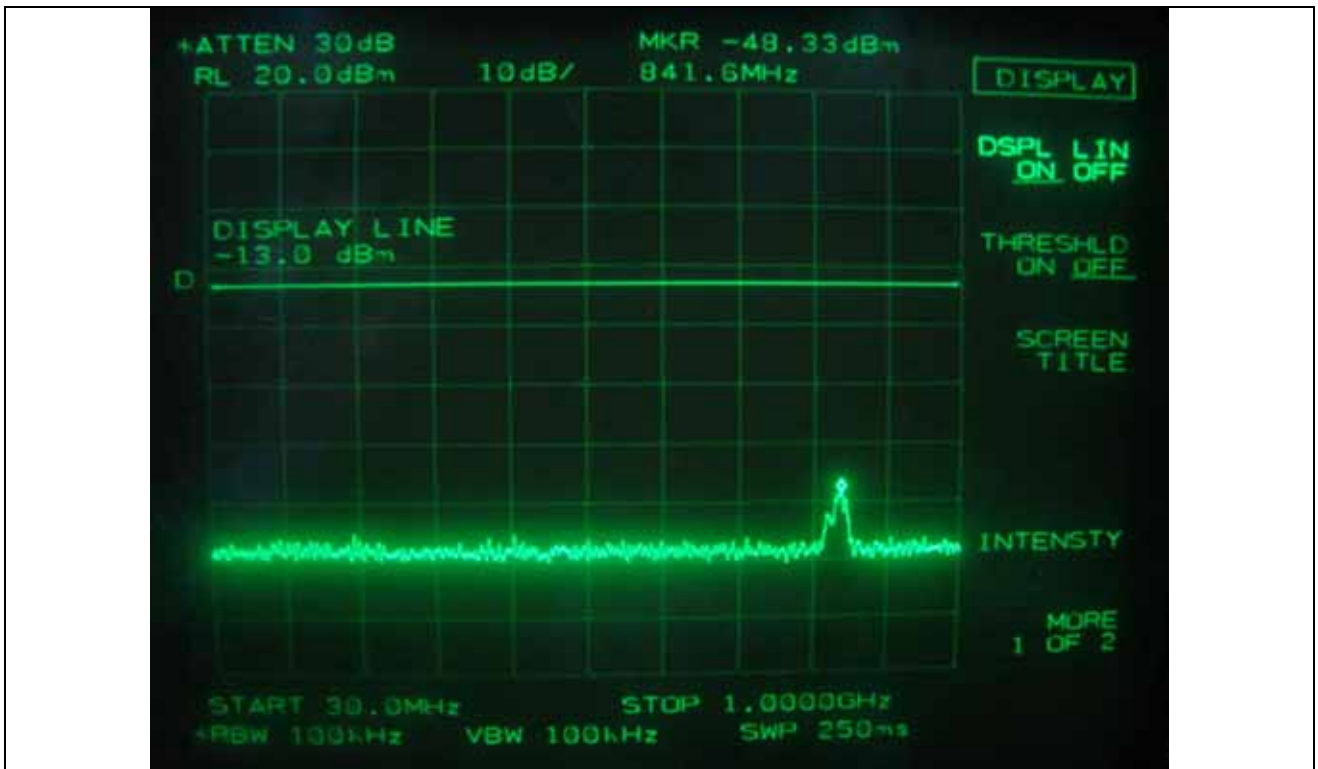
Uplink: CDMA 2000- Middle Channel
