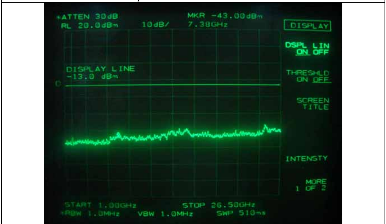
Uplink: CDMA 2000- Middle Channel
