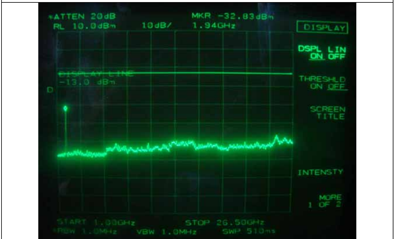
Downlink: IS-95 CDMA - Low Channel
