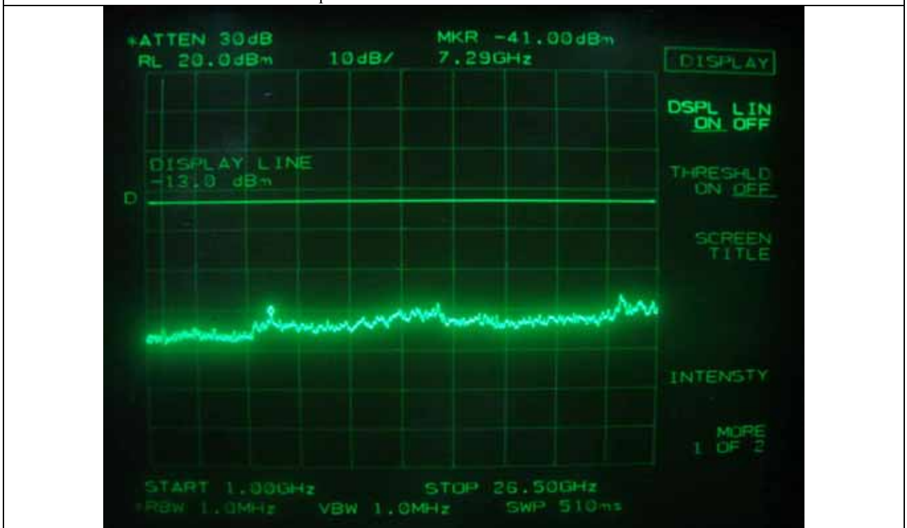
Uplink: IS-95 CDMA - Middle Channel
