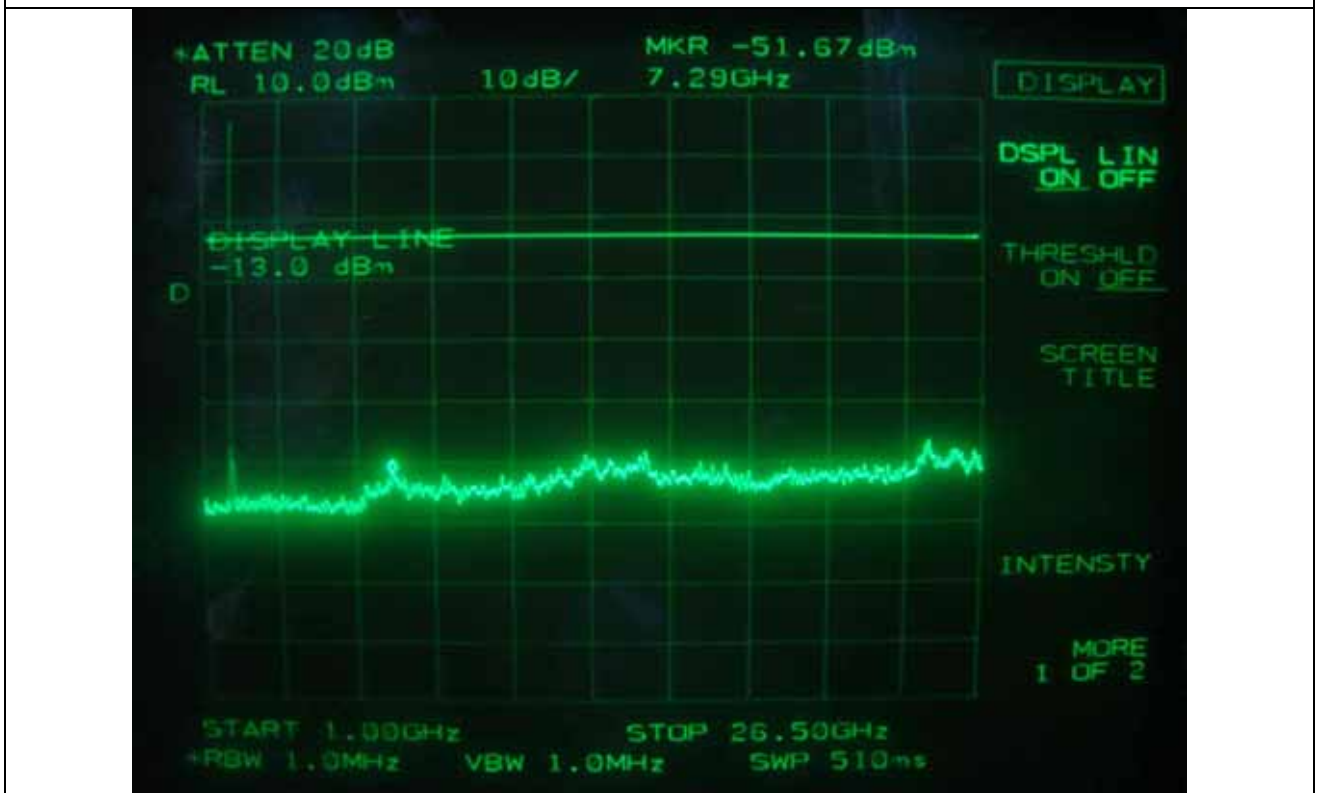
Downlink: IS-95 CDMA - Middle Channel
