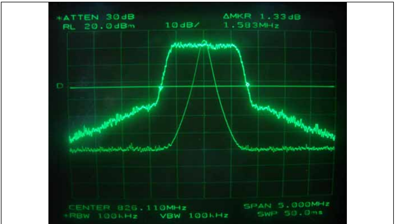
CDMA 2000 - 26dB Bandwidth
