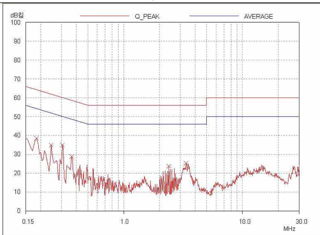
NEUTRAL LINE
