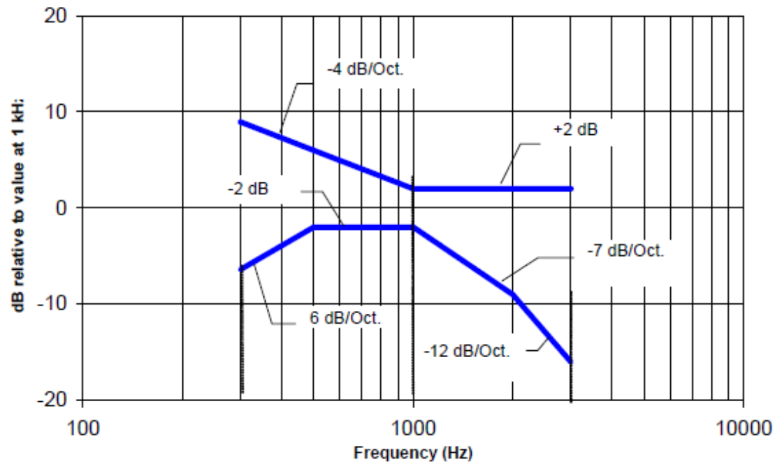
Fig. 4.2 Magnetic field frequency response for WDs with a field that exceeds -15 dB(A/m) at 1 kHz
