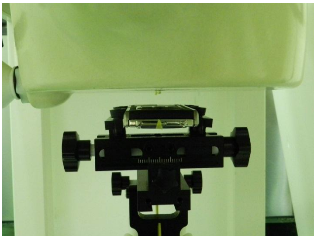
Back of the DUT with Phantom 1.5 cm Gap (without Headset)
