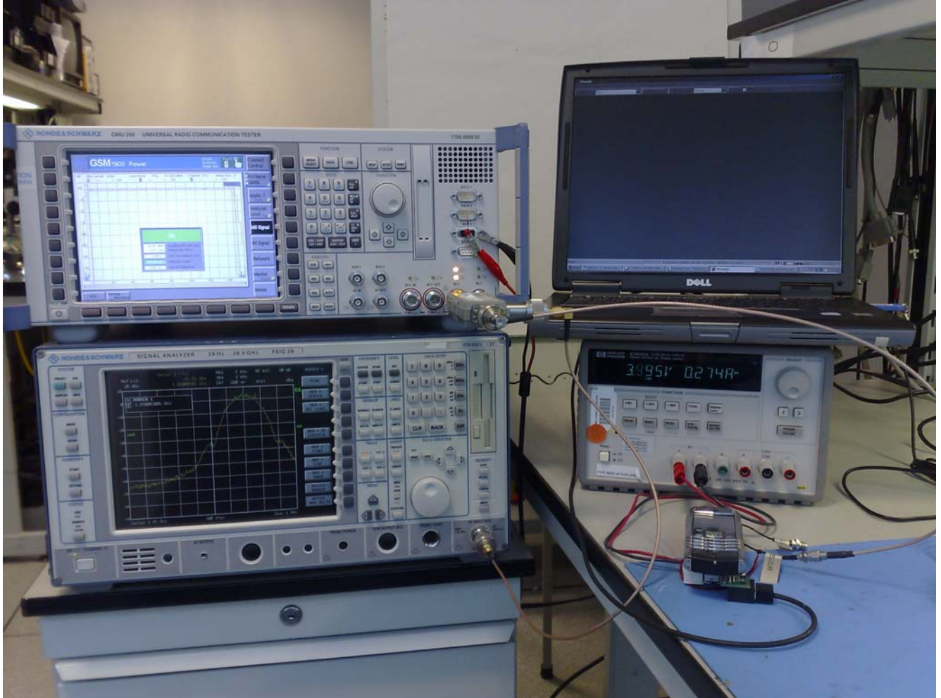
Picture 1 Band Edge Emission measurement
