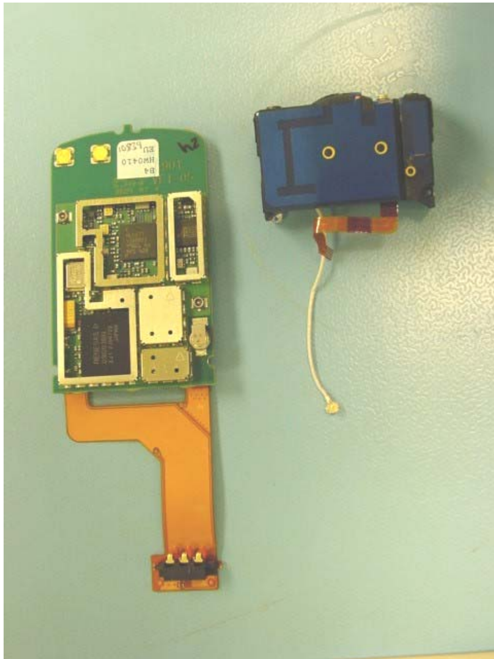
Exhibit 3: INTERNAL VIEW of Vertu FCCID: P7QRHV-3 .
