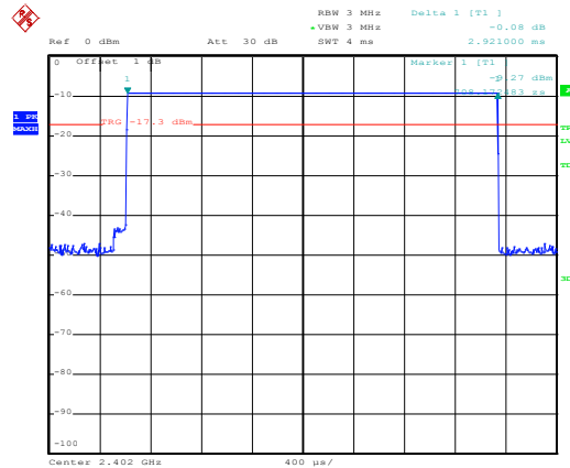
Figure 8. Plot of the Time of Occupancy (Conducted)
