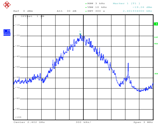
Figure 16. Plot of the Peak Power Spectral Density (Conducted) - GFSK
