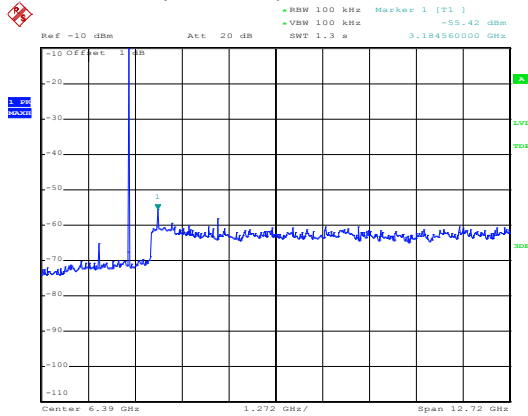
Figure 12. Plot of the Spurious RF conducted emissions - GFSK
