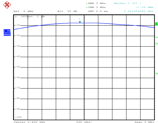
Figure 1. Plot of the Maximum Peak Output Power (Conducted) - GFSK
