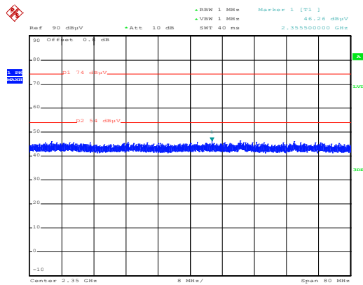
Figure 11. Plot of the Band Edge (Radiated) - GFSK
