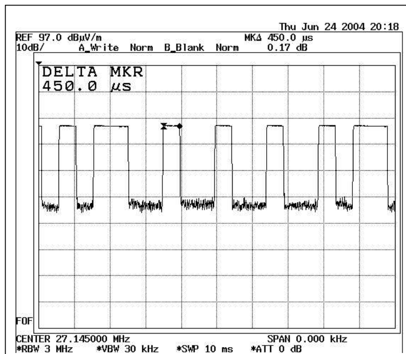
Duty Cycle 3
