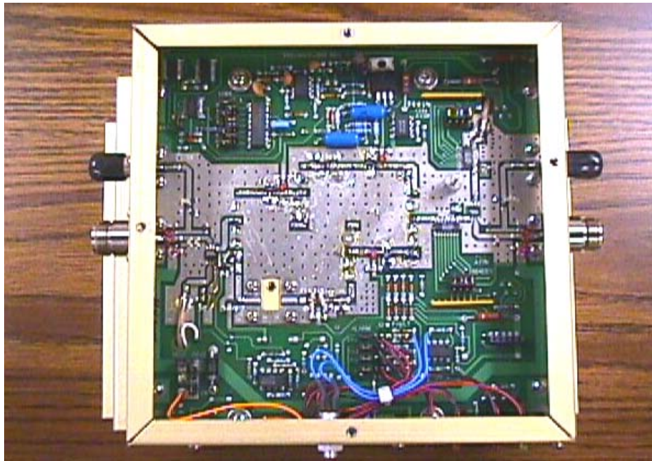
PCS PC BOARD ASSEMBLY
