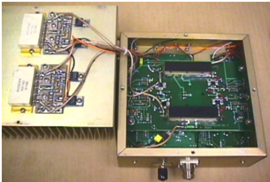
HEATSINK ASSEMBLY AND CELLULAR PC BOARD ASSEMBLY
