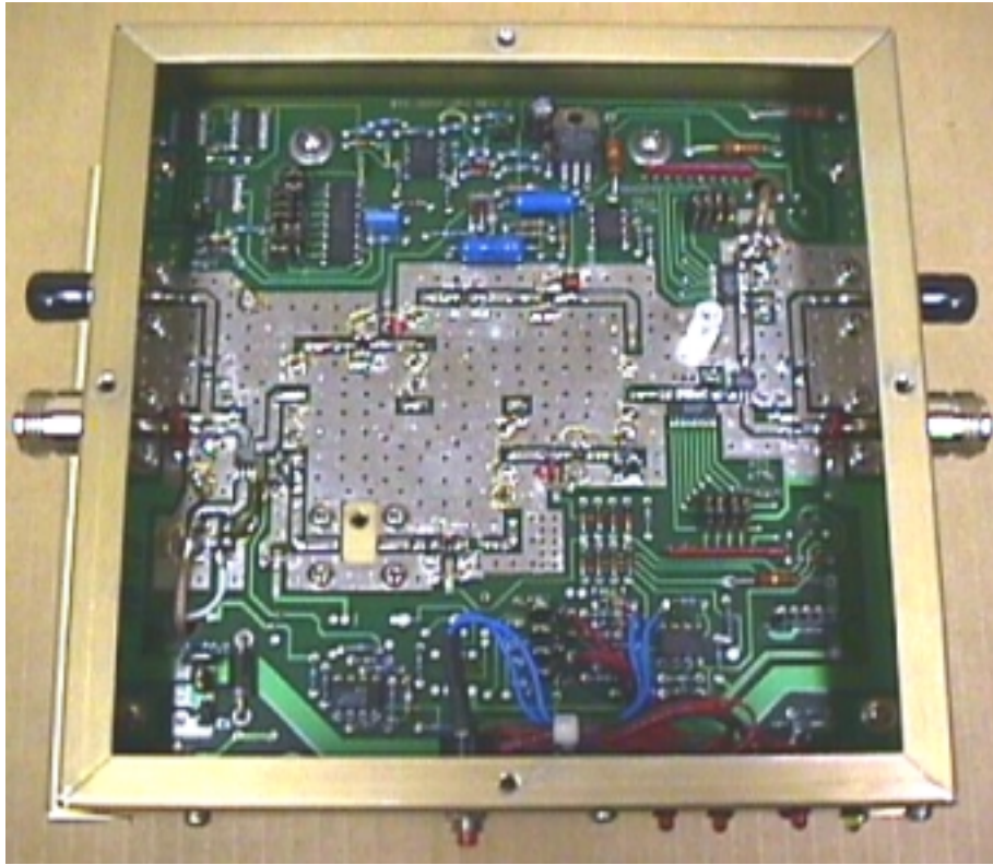
PCS PC BOARD ASSEMBLY
