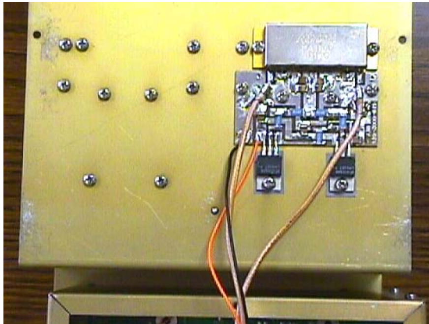
HEATSINK ASSEMBLY
