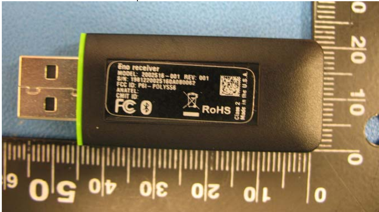
ēno receiver External Bottom with Cap Off
