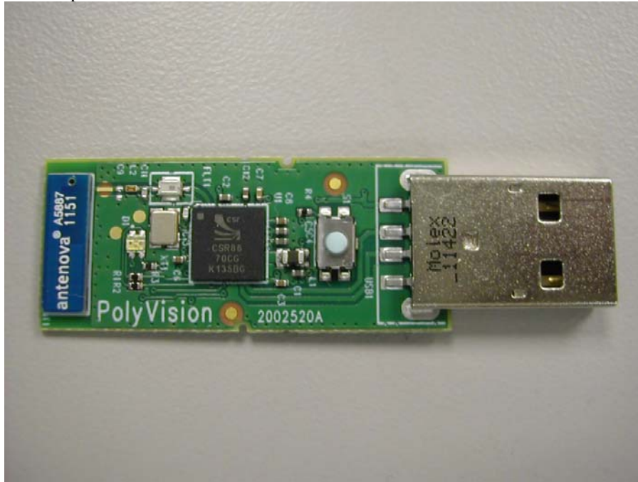
ēno receiver PCBA Top
