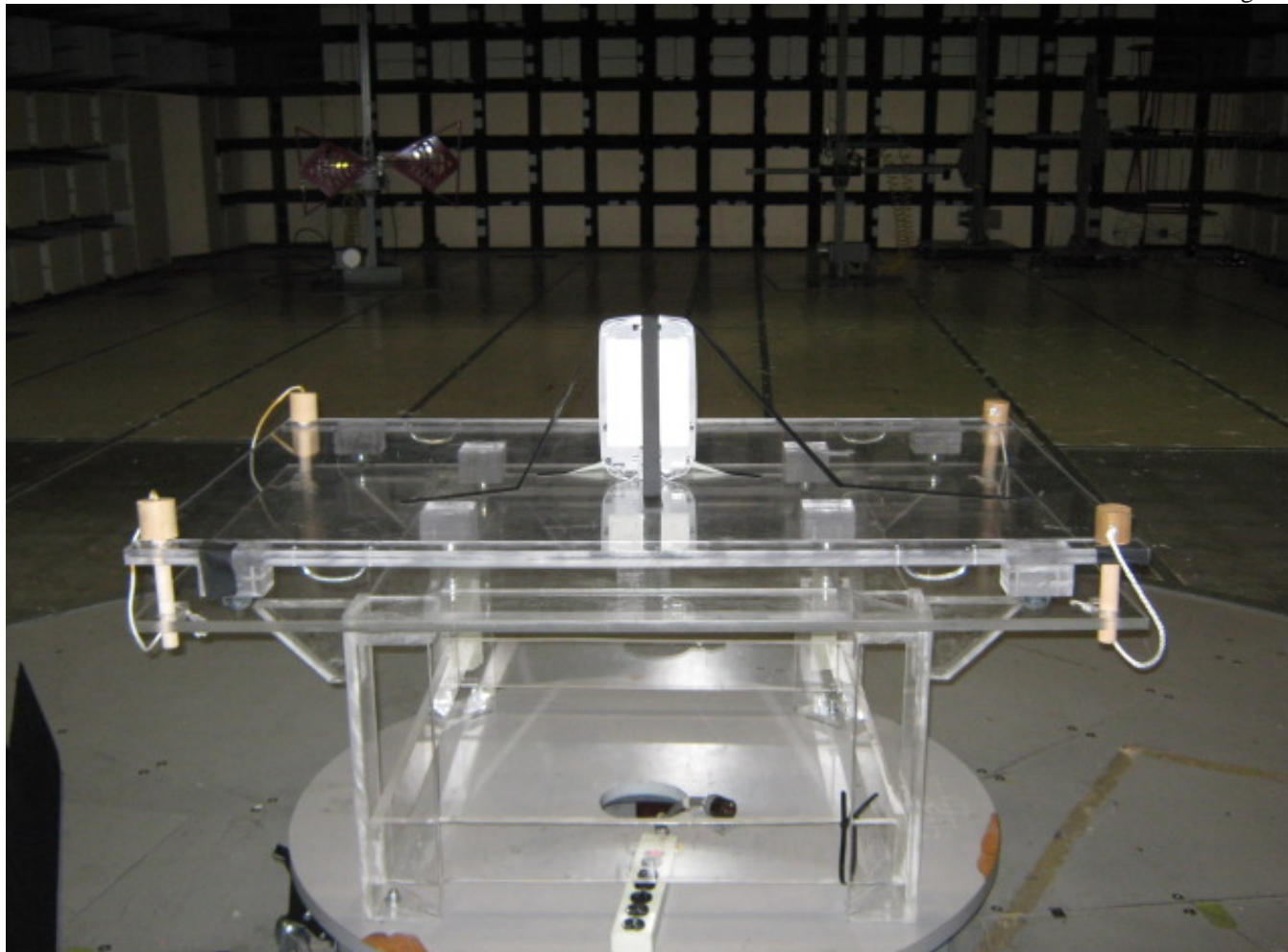
Radiated Emissions Back
