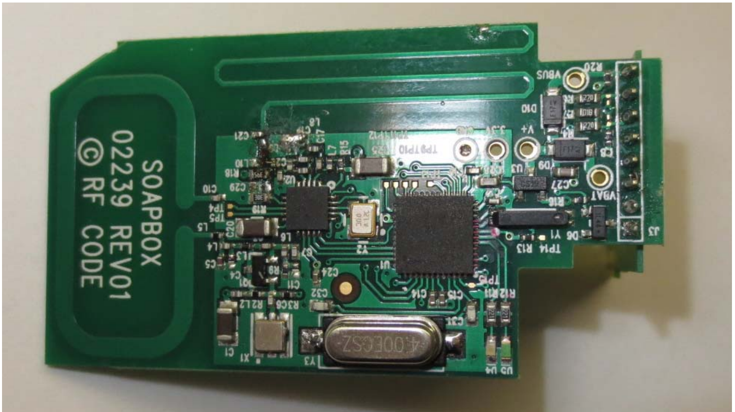
Top View – component side
