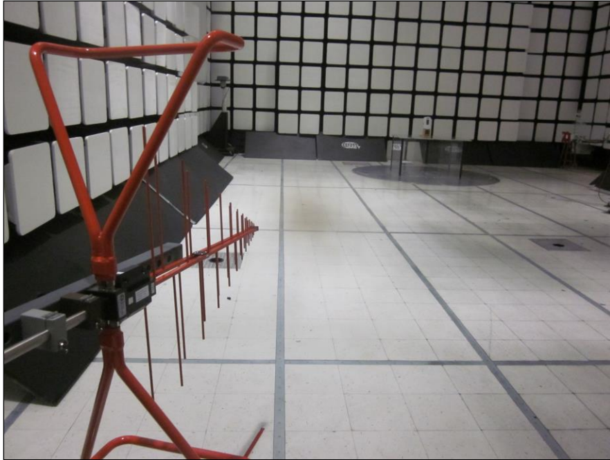
Photograph 3. Radiated Spurious Emissions, 30 MHz – 1 GHz, Test Setup
