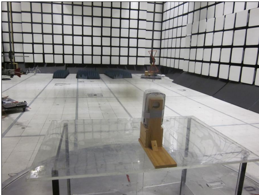
Photograph 2. Radiated Emissions, Test Setup, Rear View
