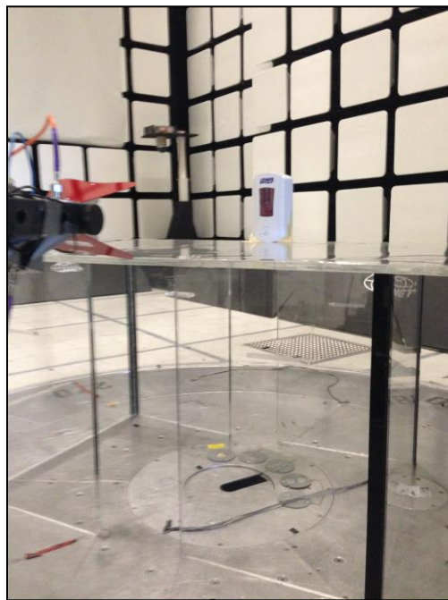
Photograph 4. Radiated Spurious Emissions, 1 GHz – 10 GHz, Test Setup
