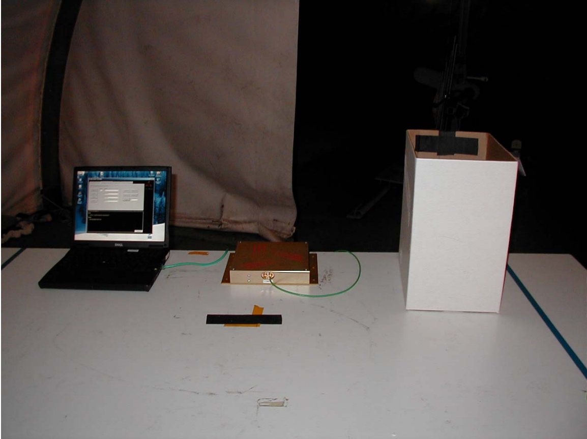
RADIATED EMISSION SETUP (1 OF 2)
