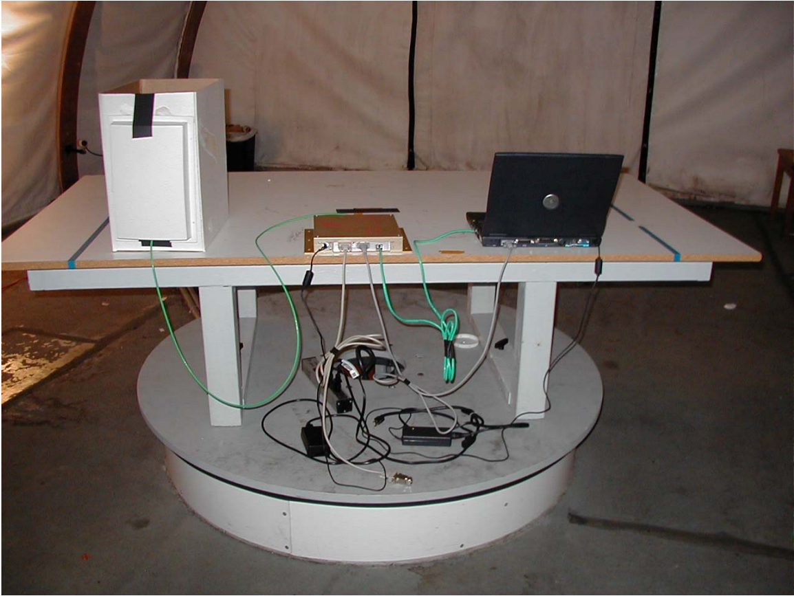
RADIATED EMISSION SETUP (2 OF 2)
