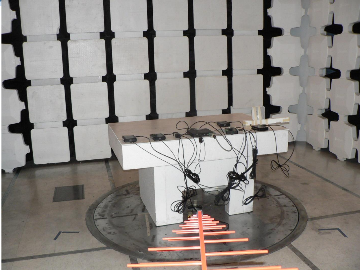
Digital Emissions Setup
