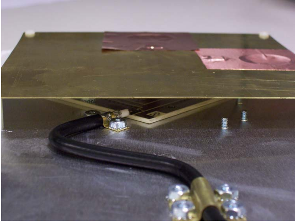
Circular Antenna Internal View
