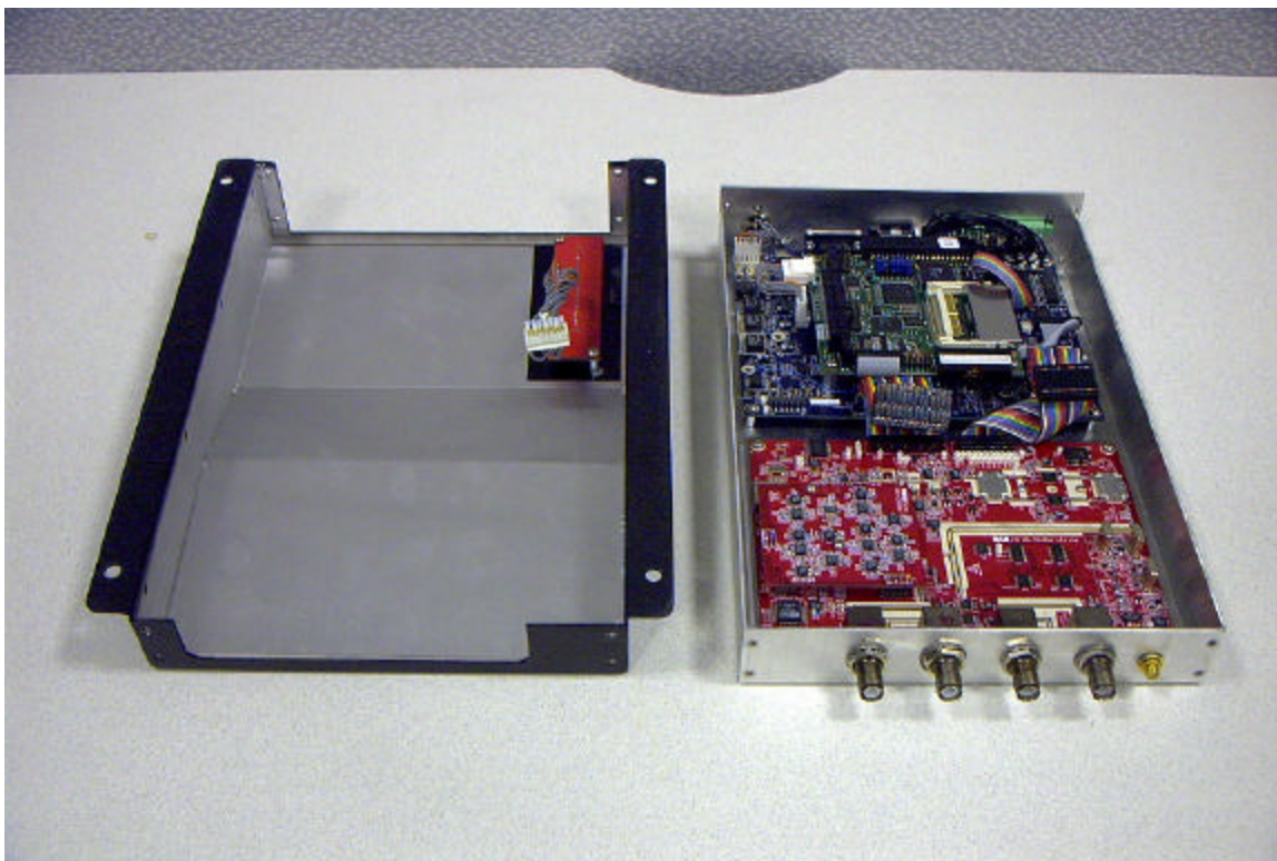
ALR 9800 Top Cover Removed
