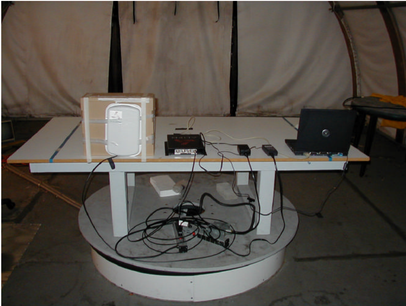
RADIATED TEST SETUP PHOTO 2 OF 2
