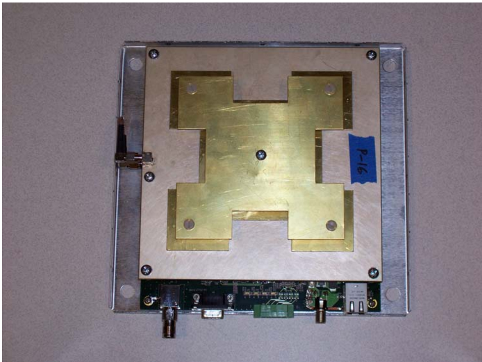
Internal Antenna Assembly
