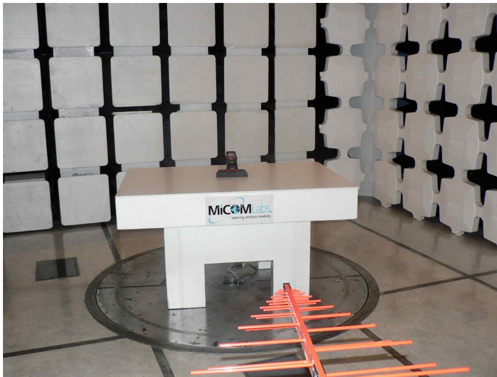
TX Spurious 30-1000 MHz
