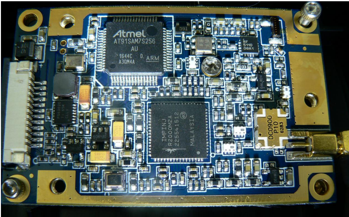
Module without Shield
