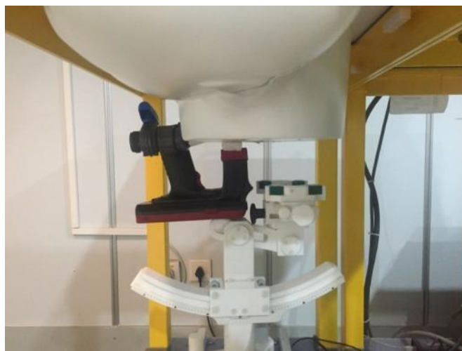
Fig.12 Body RFID(Back upside,10mm separation)
